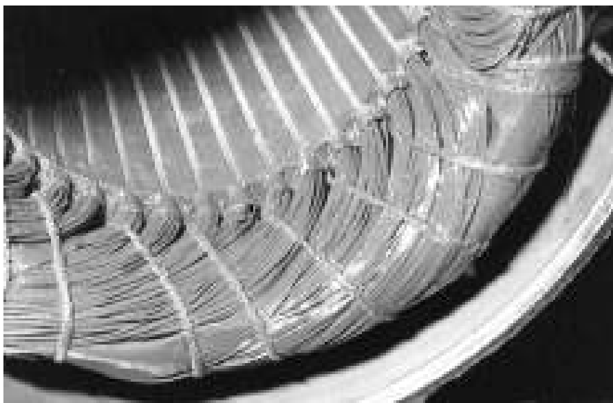
Figure 1.5. Photograph of the end-winding and slots of a random-wound stator. (Courtesy TECO-Westinghouse.)
