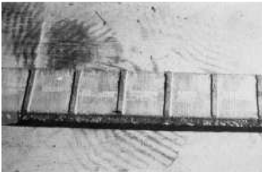
Figure 8.3. Photograph of the side of a coil suffering from insulation abrasion due to loose windings. The abrasion occurred along the length of the coil, since the coil was not installed tightly. The vertical ridges are where the vent ducts occur in the stator core.
