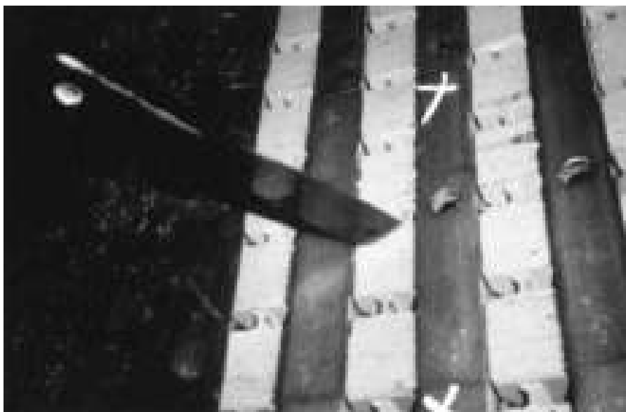
Figure 14.1. Photo of a knife being inserted between the laminations of a loose stator core.
