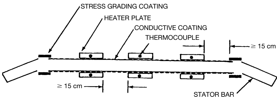
Figure 2.2. Application of heater plates to a stator bar for the IEEE 1043 voltage endurance test.
