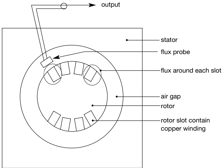
Figure 13.8. Drawing showing location of a flux probe in a turbogenerator airgap.
