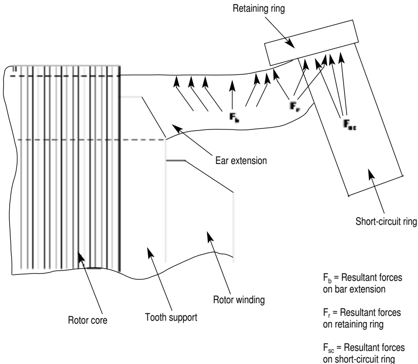
Figure 9.3. Distortion of rotor bars outside of a slot by mechanical forces during motor starting.
