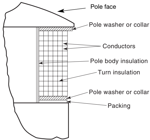
Figure 1.20. Cross section of a multilayer salient pole.
