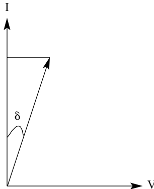
Figure 12.1. Calculation of phase angle for \tan \delta measurement.
