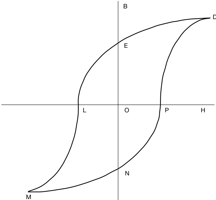
Figure 6.1. The hysteresis loop for a ferromagnetic material. The initial magnetization curve from O to D is not shown. The length O to E is the residual induction, whereas O to L is the coercive force. The width of the loop from L to P is exaggerated compared to materials commonly used in electromagnetic cores.
