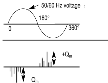
Figure 12.3. Oscilloscope display of PD pulses (lower trace) versus the power-frequency voltage waveform.
