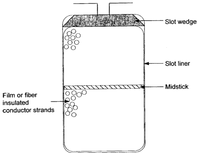
Figure 1.23. Cross section of a small wound-rotor slot.
