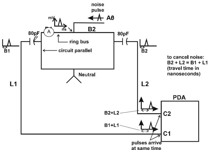
Figure 13.4. Location of capacitive couplers on the circuit ring bus of a hydrogenerator.
