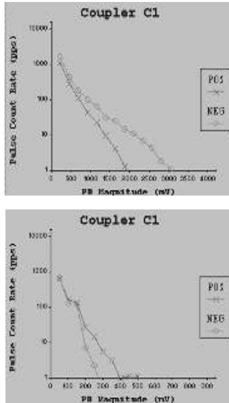
Figure 13.7. Comparison of PD activity in two stators. The stator with higher magnitude PD (on top) is most deteriorated. (Courtesy of Iris Power Engineering.)
