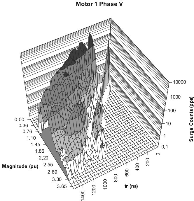
Figure 13.11. Surge repetition rate versus magnitude and risetime for a typical 600 V motor driven by a PWM-type IFD. (Courtesy Iris Power Engineering.)
