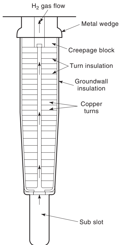
Figure 1.22. Cross section of a round rotor slot.
