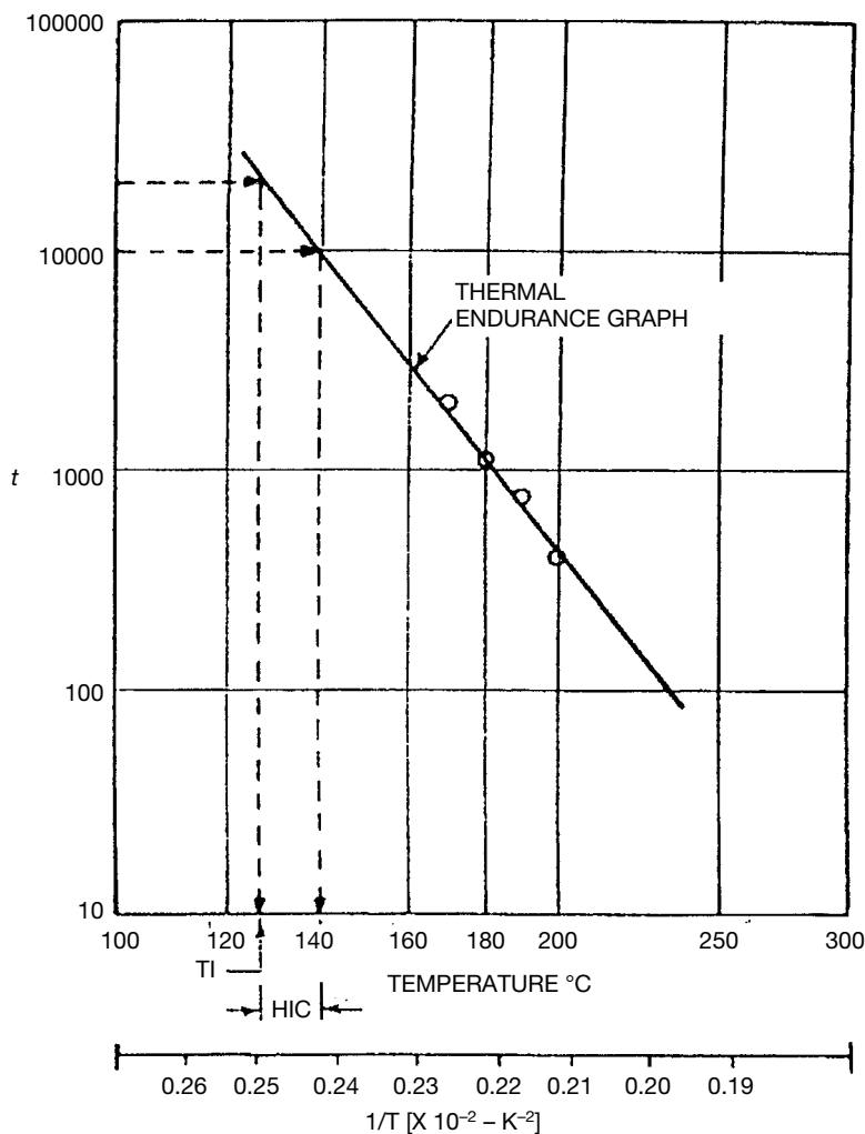
Figure 2.1. Typical thermal endurance plot for a Class B (Class 130) material. Note the thermal index corresponds to a life of 20,000 hours. (Copyright © 1989 IEEE. All rights reserved.)
