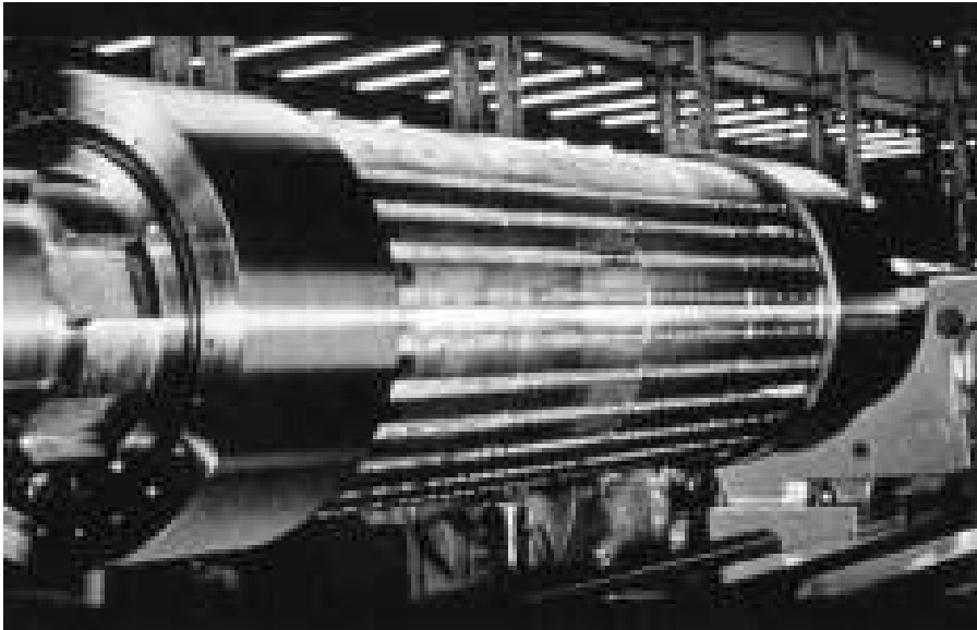
Figure 1.2. Phototgraph of a small round rotor. The retaining rings are at each end of the rotor body.
