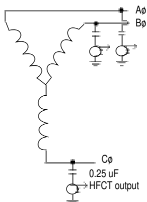
Figure 13.2. Placement of HFCT sensors to measure PD.
