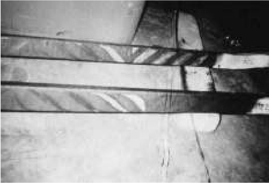
Figure 8.4. Photograph of a stator bar removed from a large hydrogen-cooled stator. The light-colored arcs are where the side ripple springs abraded the groundwall insulation.
