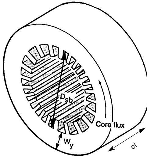
Figure 14.3. Dimensions for calculating core area.
