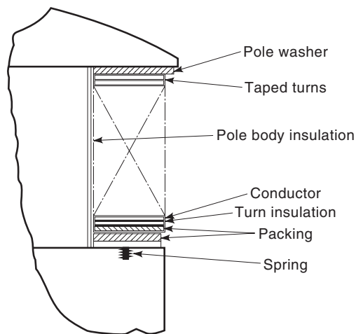
Figure 1.21. Cross section of a "strip-on-edge" salient pole.
