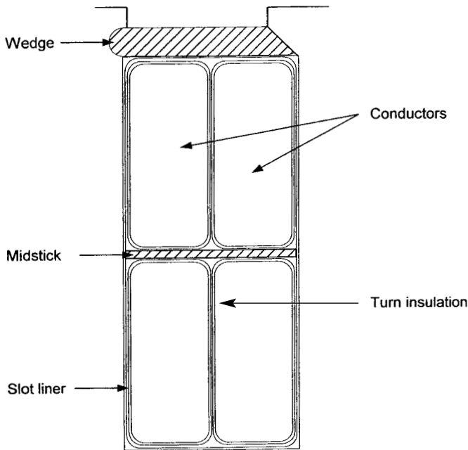
Figure 1.24. Cross section of a large wound stator slot.
