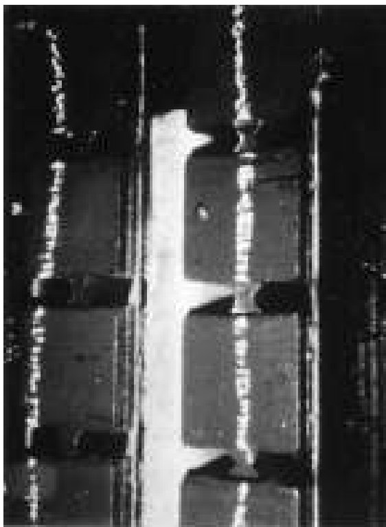
Figure 8.5. Photograph of two stator slots taken from the axis of an air-cooled machine. The stator wedges have been removed, exposing the tops of the two coils. The semiconductive coating on the coil connected to the phase terminal has disappeared.
