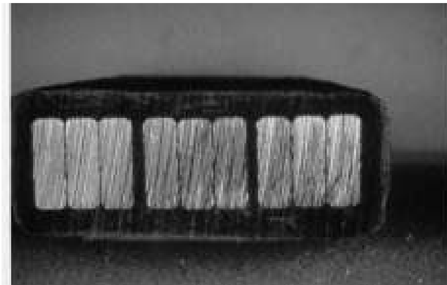
Figure 1.10. Cross-section of a multitransformer coil, with three turns and three strands per turn.
