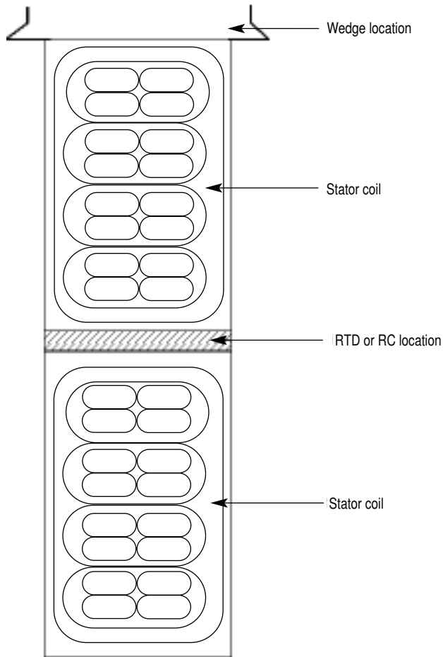
Figure 13.1. Placement of an RTD or TC between the coils/bars in a stator slot.
