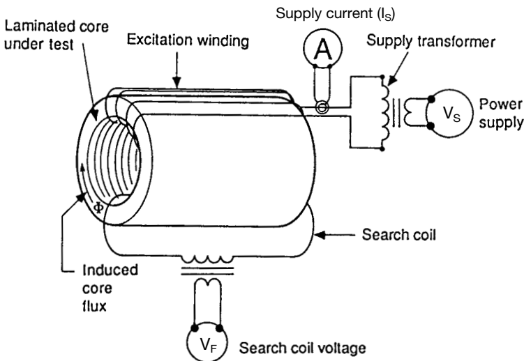
Figure 14.2. Test arrangement for rated core flux test.
