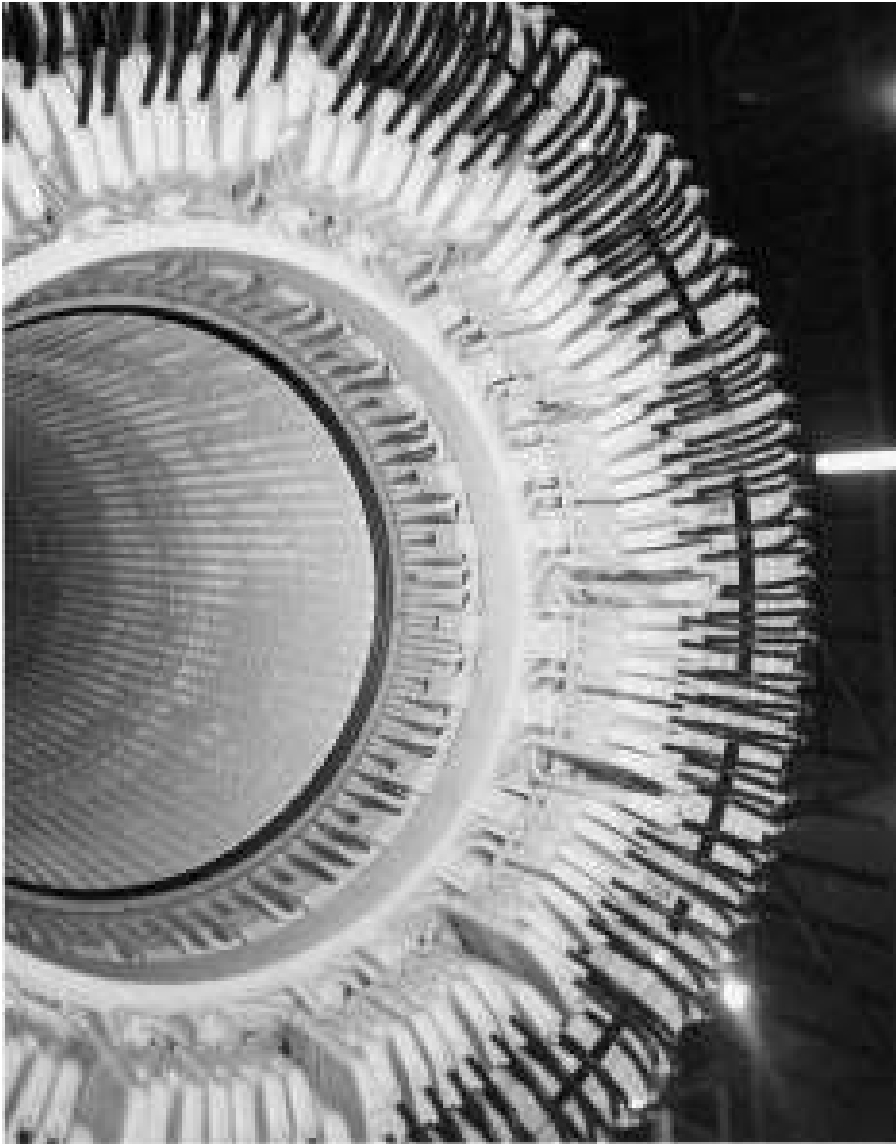
Figure 1.7. Photo of a turbogenerator stator winding using Roebel bars.
