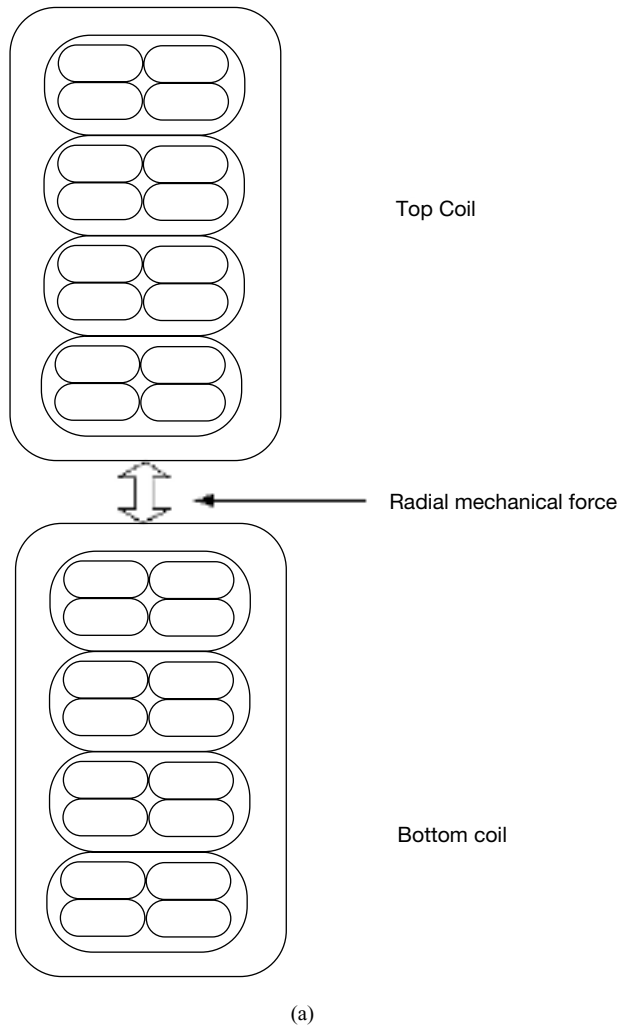
Figure 1.17. Schematics showing the magnetically induced mechanical forces occurring (a) between the top and bottom layers of coils in the end-winding.
