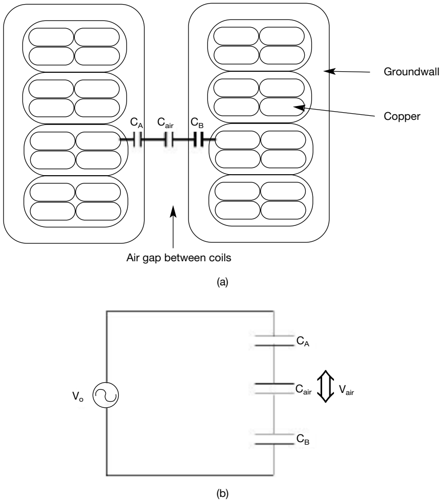
Figure 8.9. Cross section of two adjacent coils in the end-winding where PD will occur if the distance between the coils is too small.
