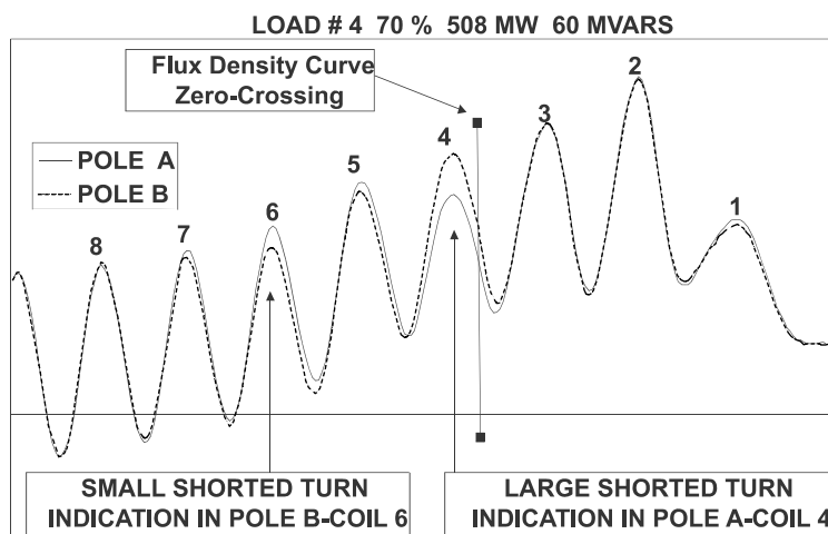
Figure 13.9. Flux probe output recorded by a digital oscilloscope. The smallest signal ripple is associated with the slot with a shorted turn. (Courtesy of GeneratorTech.)
