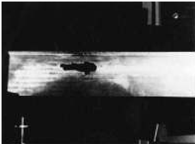
Figure 9.1. Hole abraded through the ground insulation from a slot liner near the end of a rotor slot.
