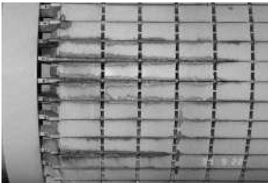
Figure 10.1. Core lamination burning due to broken rotor bars in an SCI rotor.
