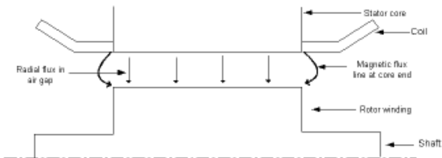
Figure 1.11. Side view of a generator showing the radial magnetic flux in the air gap and the bulging flux at the core end, which results in an axial flux.
