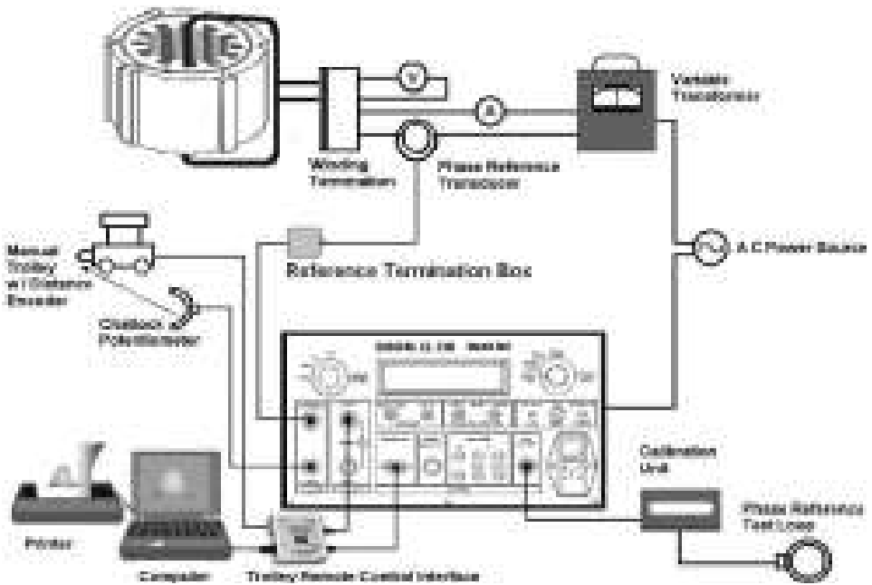
Figure 14.5. EL-CID test setup for a stator core. (Courtesy Adwel International.)
