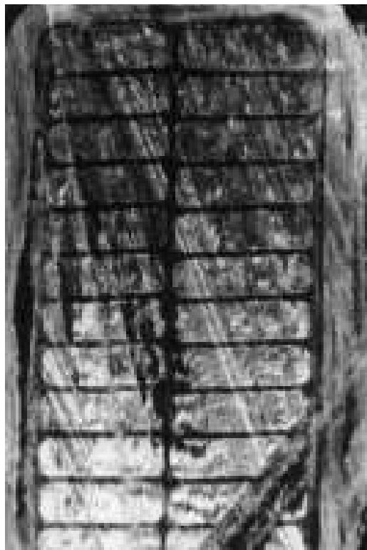
Figure 8.1. Cross section of a stator bar in which the thermal cycling forces have caused the groundwall to shear away from the copper. The black gap around the copper is where the shear occurred.
