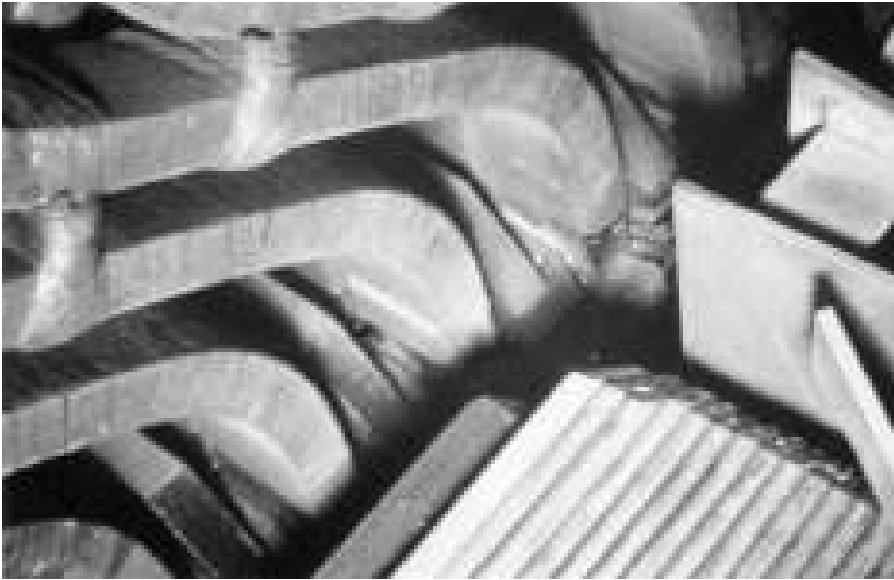
Figure 8.6. Photograph of the end-winding area from a hydrogenerator. The white band around some of the coils just outside the slot indicates where the coating overlap area has degraded.
