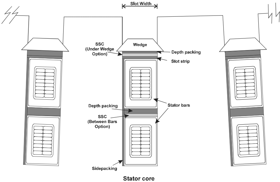
Figure 13.3. SSC location either under a wedge or between the top and bottom coils/bars.
