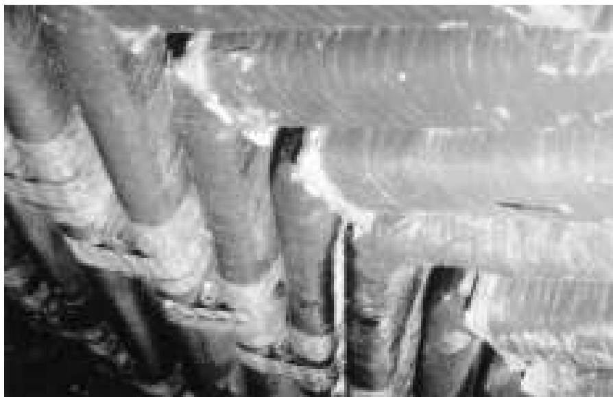
Figure 8.10. PD between adjacent coils in different phases results in white powder on the coil surfaces.
