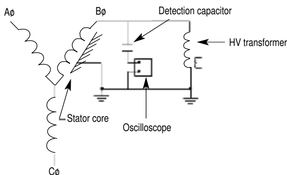
Figure 12.2. Measurement of PD pulse currents.
