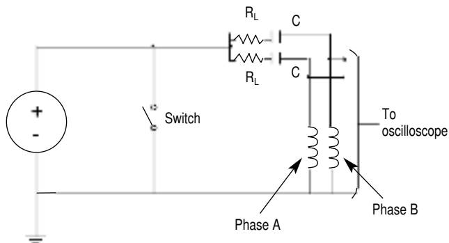
Figure 12.4. Schematic of a surge comparison tester applied to two of three phases of a stator.
