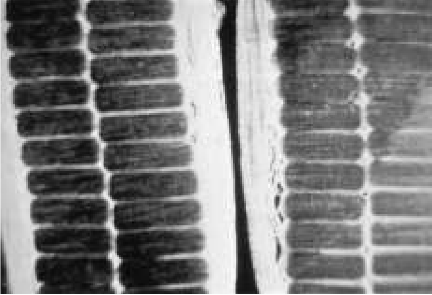
Figure 8.2. Cross section of a 12-turn coil from a 6.6 kV motor stator made using the global VPI process. The dark voids near the copper resulted from poor impregnation with epoxy, just outside of the slot.
