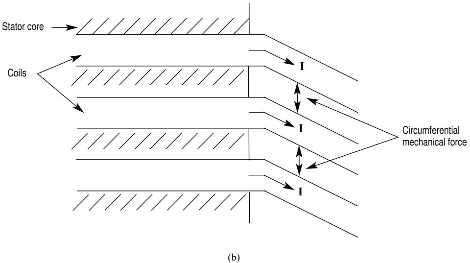
Figure 1.17. (b) between adjacent coils.
