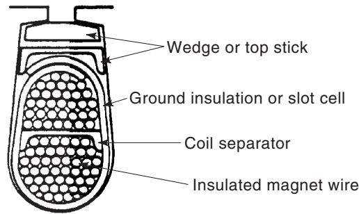
Figure 1.8. Cross section of a random stator winding slot.
