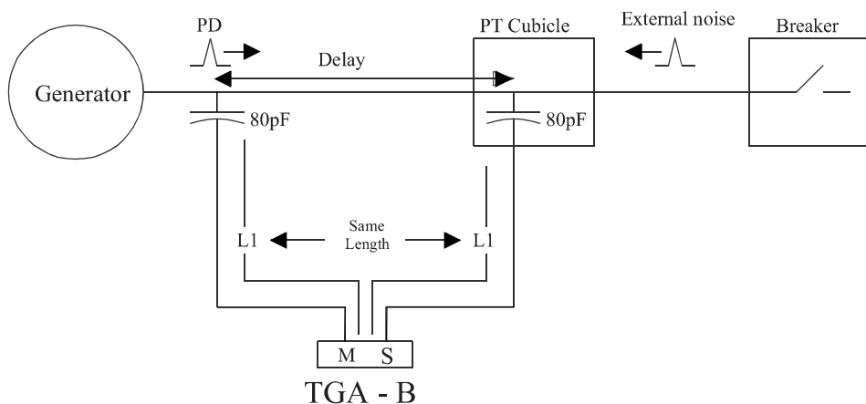
Figure 13.5. Installation of two capacitors per phase to separate PD from noise.
