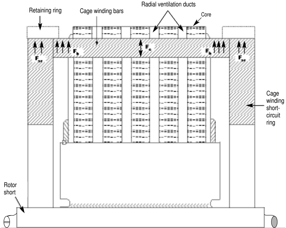
Figure 9.2. Different mechanical forces that occur in an SCI rotor.
