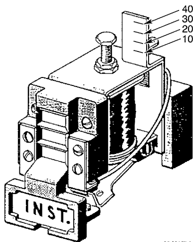
FIGURE 5.12 Electromechanical instantaneous unit.
