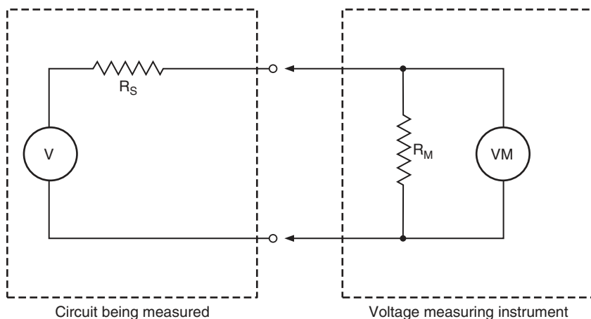
FIGURE 3.21 Equivalent circuit of voltage measurement.
