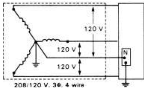
FIGURE 9.6 Grounding a 208/120-V three-phase, four-wire system.
