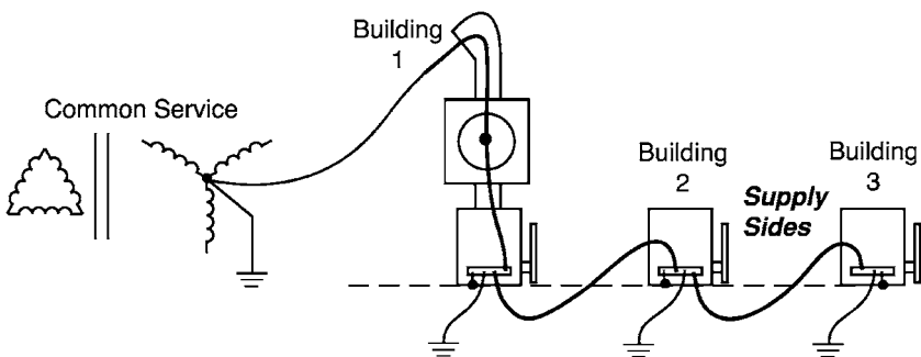
FIGURE 4.22 Common service with no equipment grounding conductor run. (Courtesy of AVO Training Institute, Inc.)
