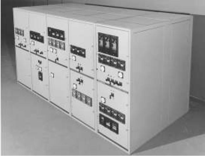
FIGURE 3.5 Metal-clad, medium-voltage switchgear for vacuum-type circuit breakers. (Courtesy General Electric.)
