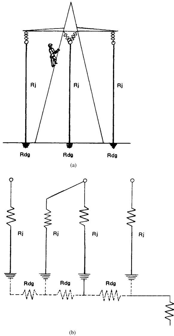
FIGURE 3.26 Two incorrect, nonpreferred safety ground configurations.
