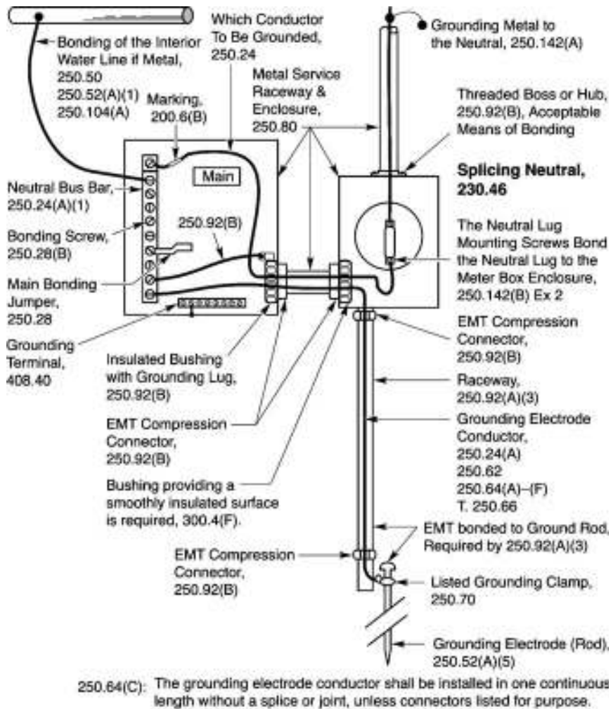
FIGURE 4.23 Service grounding and bonding requirements. (Courtesy of AVO Training Institute, Inc.)
