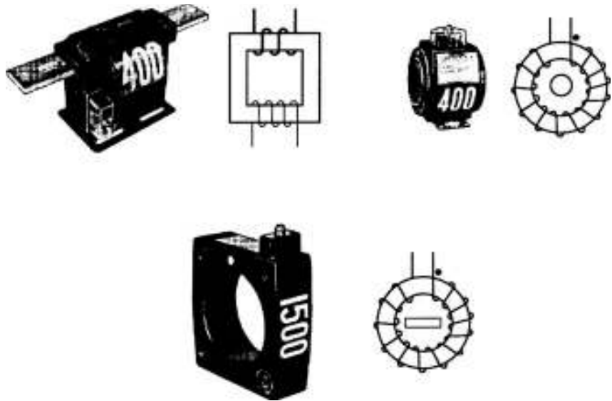
FIGURE 10.1 Typical current transformers. (Courtesy AVO Training Institute.)
