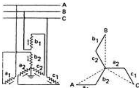
FIGURE 10.7 Grounding autotransformer with interconnected Y (also called zigzag windings).
