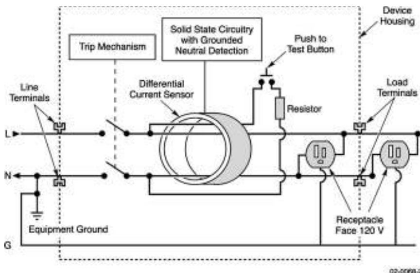
FIGURE 4.15 Internal diagram of a ground-fault circuit interrupter (GFCI). (Courtesy of AVO Training Institute, Inc.)
