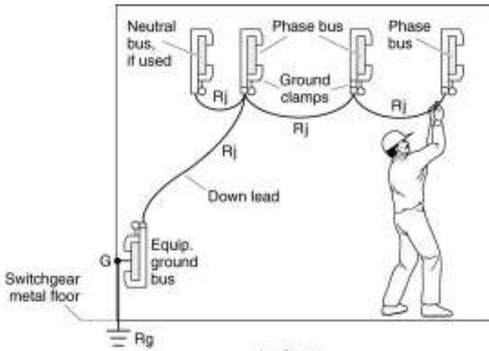
(a) Switchgear
