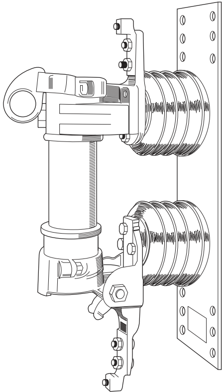
FIGURE 3.17 Open-air, fused disconnect switch. (Courtesy General Electric.)
