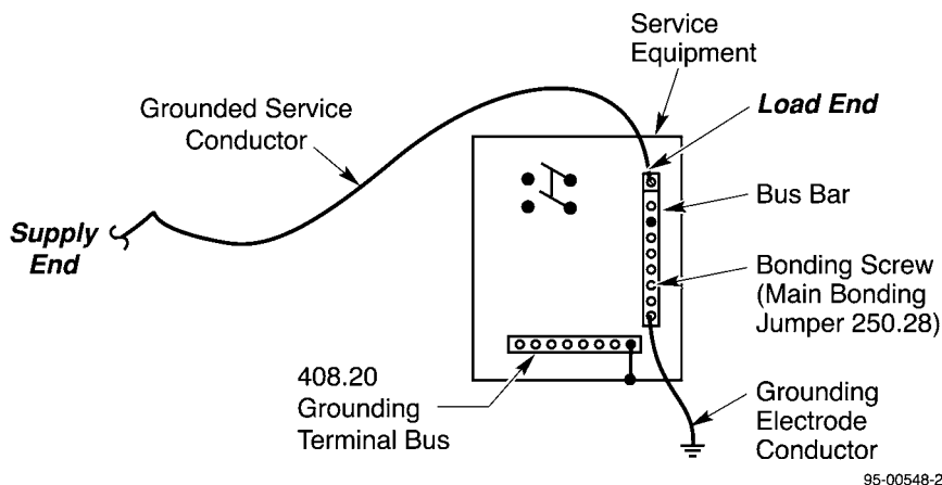
FIGURE 4.6 Grounding service conductor connection to grounding electrode. (Courtesy of AVO Training Institute, Inc.)
