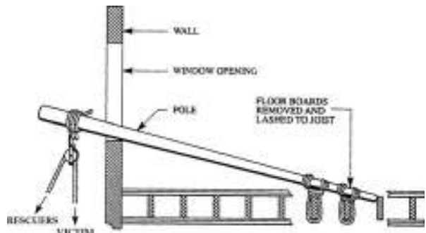
FIGURE 7.17 Gin pole hoist. (Courtesy AVO, International.)
