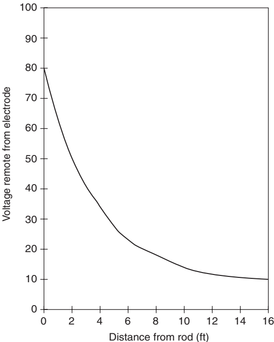
FIGURE 1—Typical Voltage-Gradient Distribution Curve.
