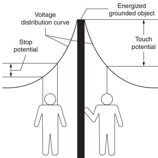
FIGURE 2—Step and Touch Potentials.
