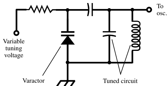
electric tuning
