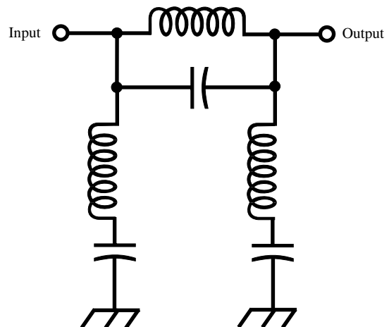
rejection filter
