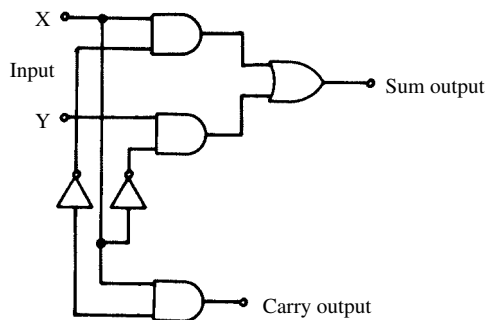
half-adder
