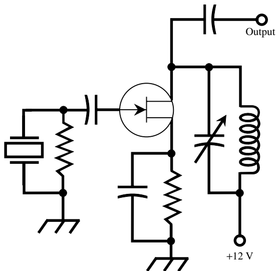
Miller oscillator
