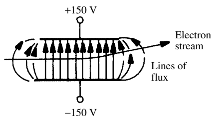
electrostatic deflection
