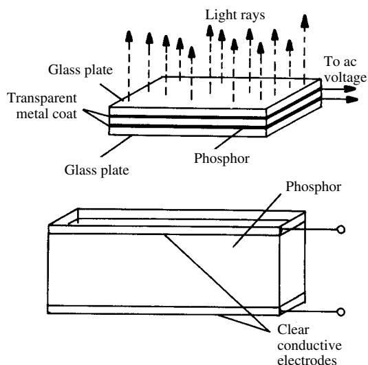
electroluminescent cell
