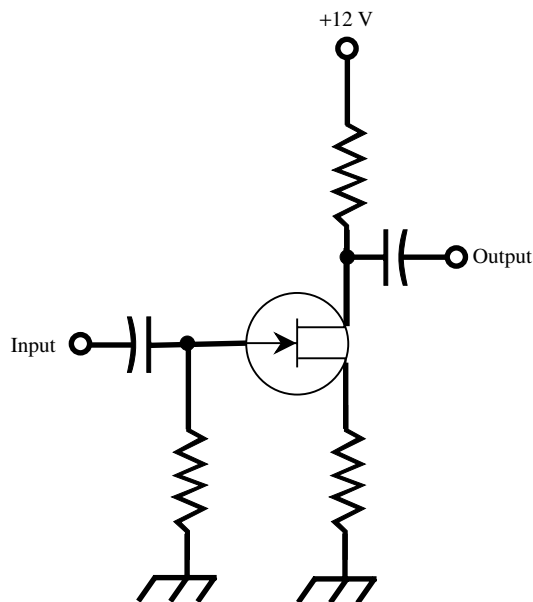
broadband amplifier
