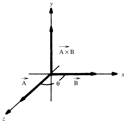
cross product
