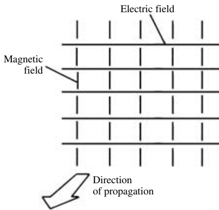
electromagnetic field
