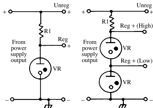
L-type voltage regulator
