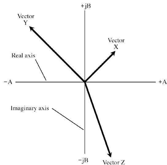
Argand diagram
