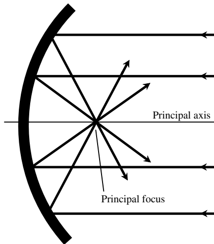
principal focus
