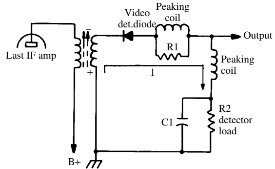
video detector
