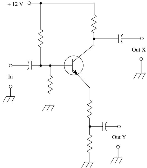
paraphase inverter
