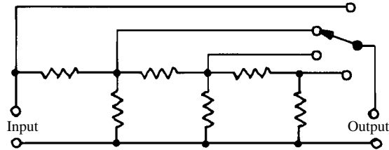
ladder-type attenuator
