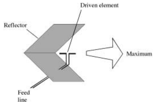
corner-reflection antenna
