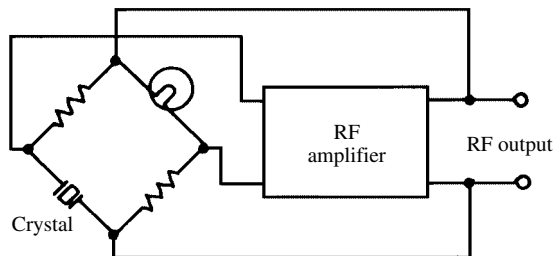
Meacham oscillator
