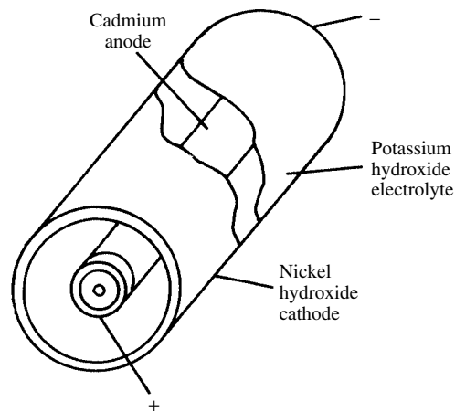
nickel-cadmium cell
