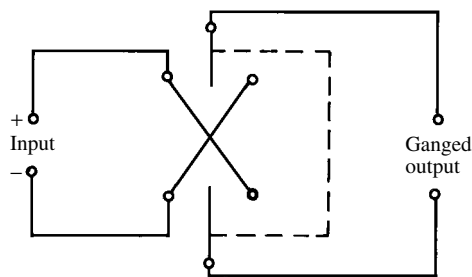
reversing switch
