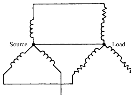
wye-wye circuit
