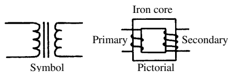
transformer, 1
