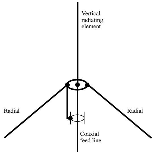
radials
