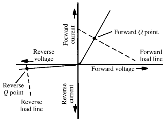
Q points on diode characteristic
