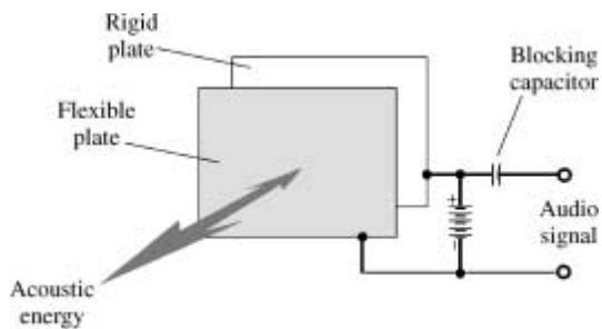
electrostatic speaker
