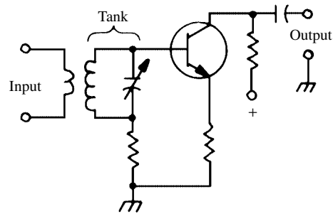
input tank
