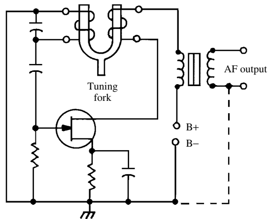
fork oscillator
