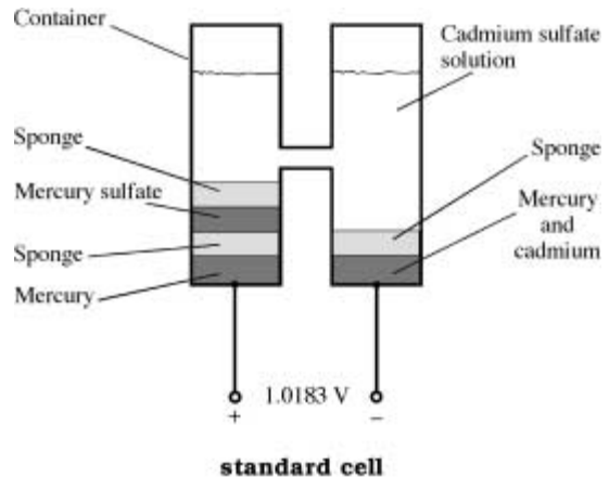
standard cell
