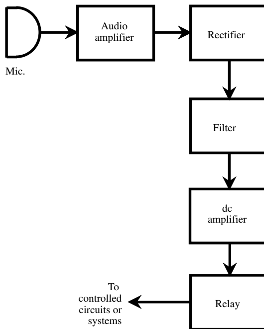
sound-operated relay
