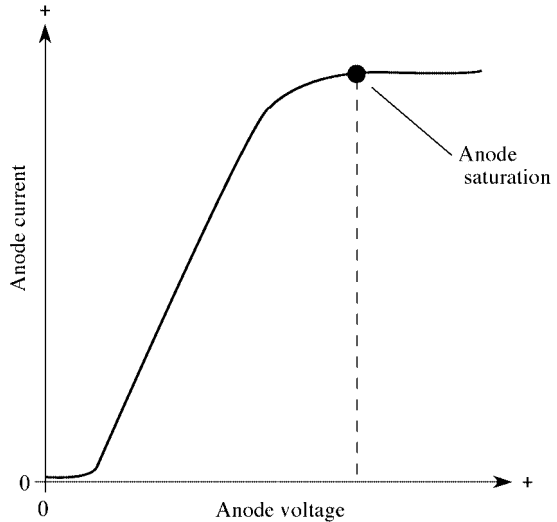
anode saturation
