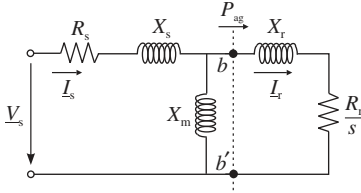
Figure 2.73. Equivalent circuit of an induction motor under steady-state conditions.
