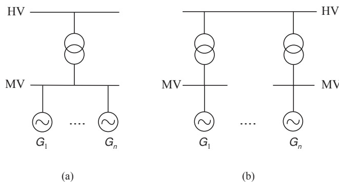
Figure 7.38. Generators parallel-connected to (a) MV bus; (b) HV bus.
