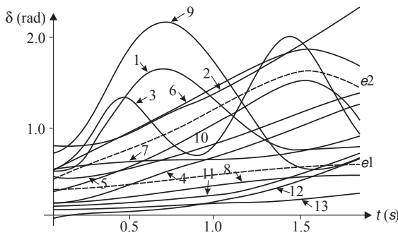
Figure 10.29. Illustration of the transient process in the equivalent system.
