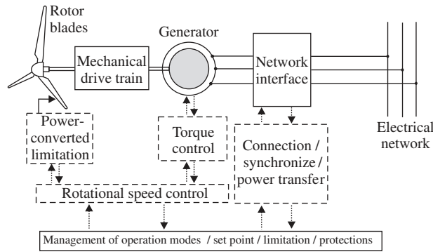
Figure 4.18. General control structure of a wind turbine [7].
