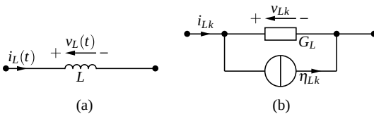
Figure 15.3. Single-phase inductance and associated companion model.
