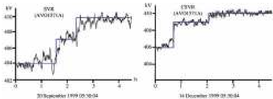
Figure 7.73. Voltage set point and voltage response with SVR and CSVR at EDF.
