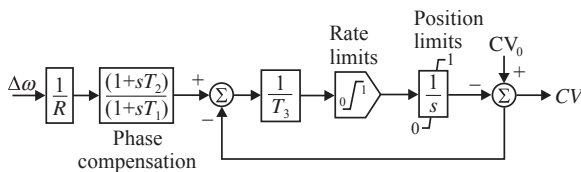
Figure 3.23. Digital electrohydraulic controls (Westinghouse) [1].
