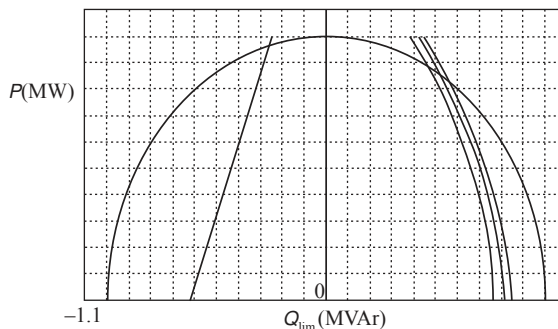
Figure 7.54. Curves of the over- and underexcitation generator limits, respectively, at the right-hand and left-hand sides.
