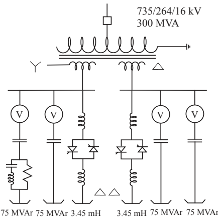
Figure 13.18. Simplified one line diagram Nemiskau/Albanel SVC's [10].
