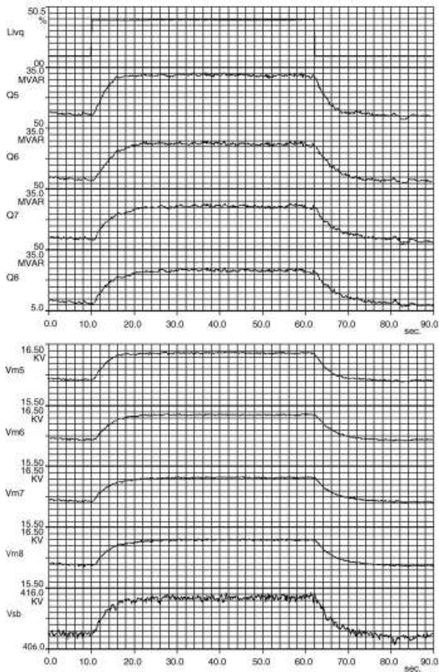
Figure 7.59. Step response of a power plant reactive power control loops showing a dominant time constant of about 5s. V_{sb} represents the local HV pilot bus bar voltage transient.
