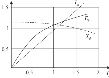
Figure 2.33. Variation of synchronous reactance.
