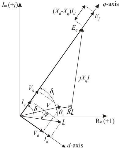
Figure 2.16. Phasor diagram of the synchronous machine under balanced steady state.
