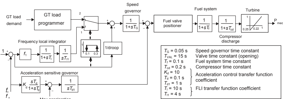
Figure 14.23. Simplified single-shaft gas turbine block diagram.
