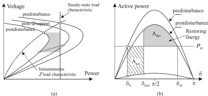
Figure 8.10. Parallelism between voltage stability and angle stability [20].
