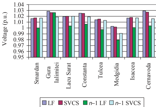
Figure 7.69. Voltage profile in case with the generator outage.
