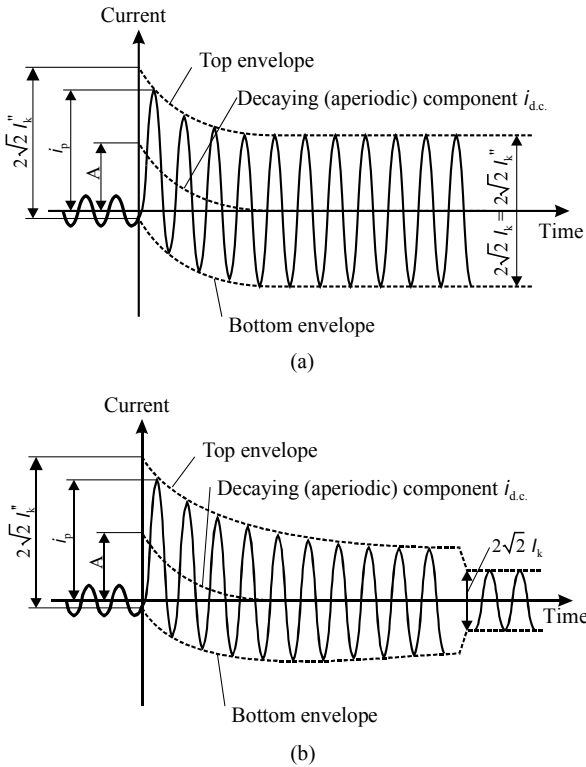
Figure 5.2. Typical wave of a short-circuit current: (a) far-from-generator short circuit with constant AC component; (b) near-to-generator short circuit with decaying AC component. (Reprinted with permission from IEC 60909. [1])
