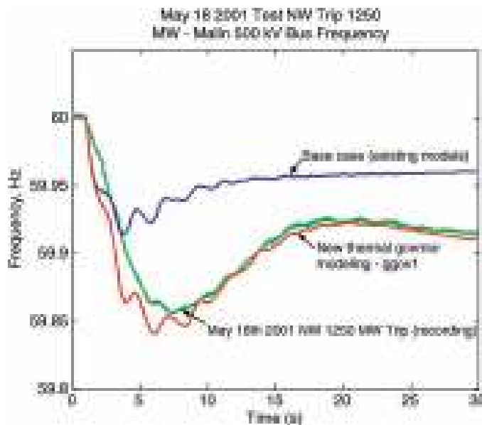
Figure 6.38. System frequency response simulations with the new governor model compared with May 18, Test recordings for the NW 1250 MW trip, all AGCs switched off.
