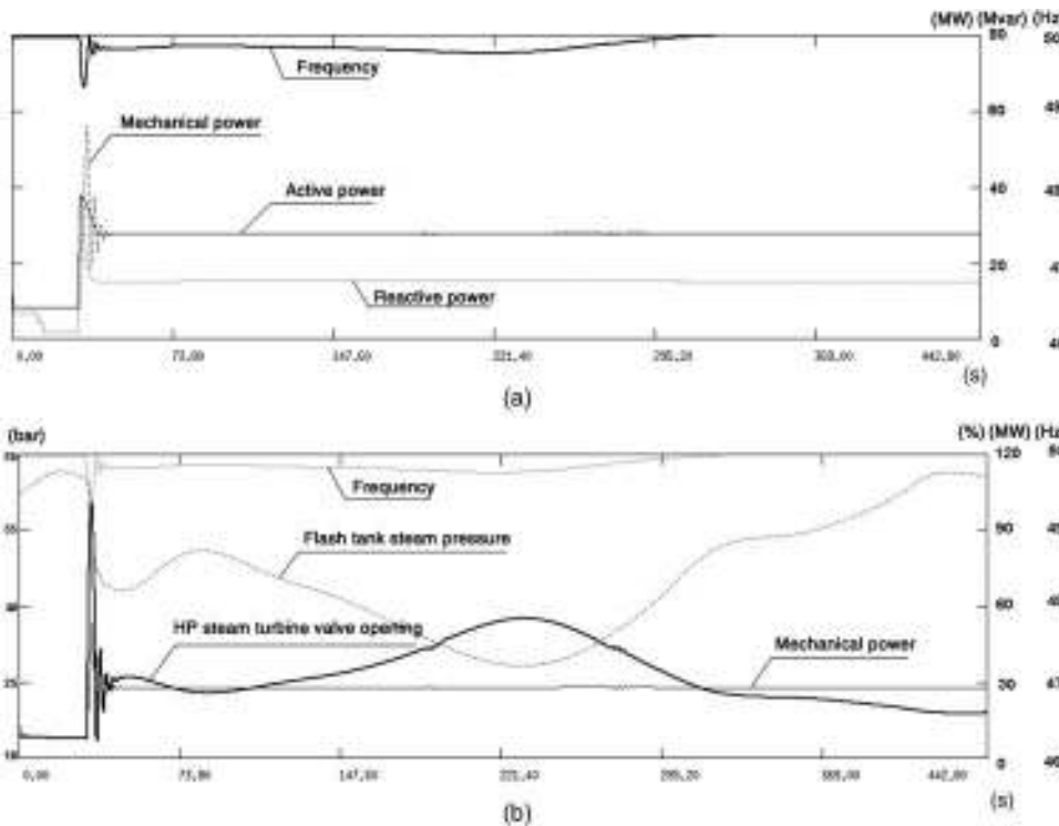
Figure 14.3. Simulation of the pick-up of a load of 18 MW by a 320-MW SPP.
