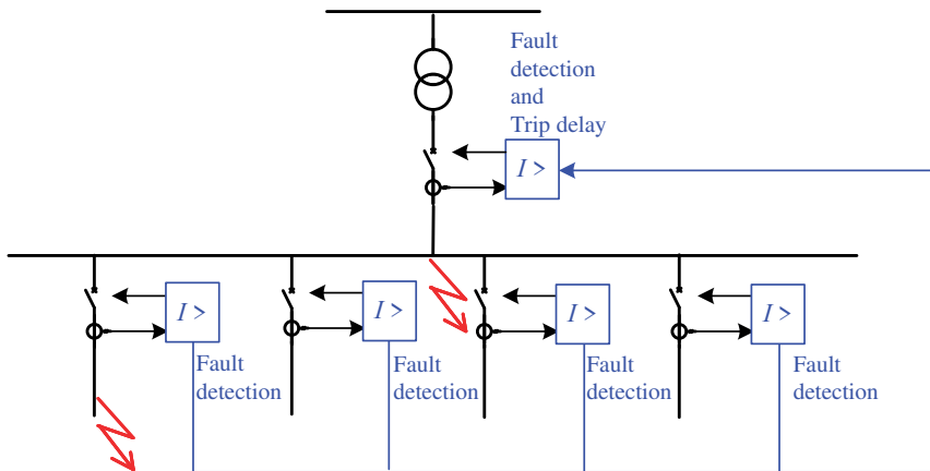
Figure 12.19. Reverse blocking of overcurrent relays in radial networks.
