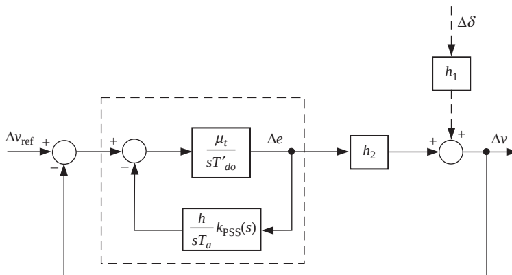
Figure 9.64. PSSs seen from the voltage loop.
