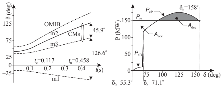
Figure 10.8. SIME method results for a three-generators system [2]: (a) the time evolution of the three generators and of the OMIB; (b) the P - \delta characteristic of the OMIB and the equal area criterion.
