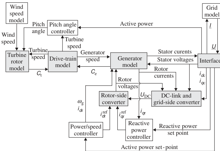
Figure 4.24. Control block diagram of a DFIG wind turbine (Adapted from [8]).
