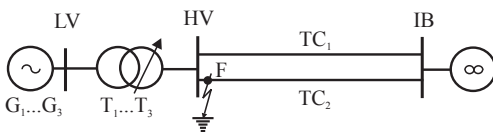
Figure 10.31. One-line diagram of the examined power system.
