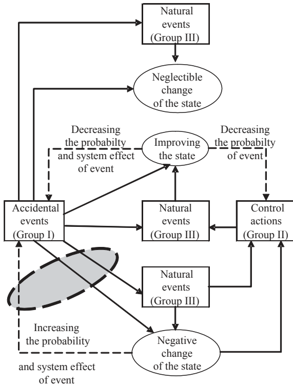
Figure 13.36. Cause-effect relationships between EPS events and its state changes.
