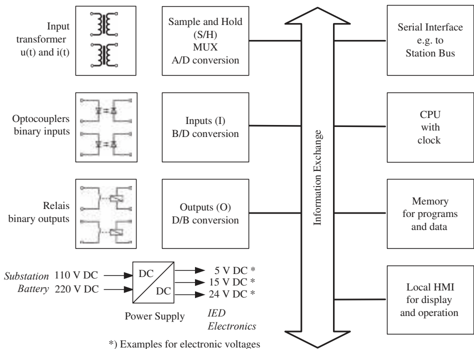
Figure 12.5. Principle diagram of a numerical protection device.
