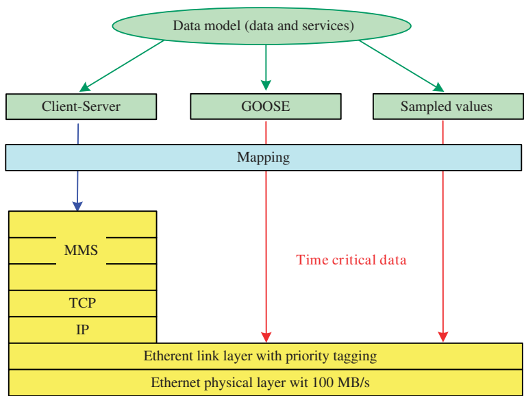
Figure 12.6. Stack as used in IEC 61850 and the relationship to the data model.
