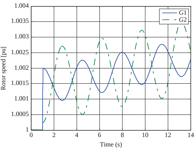
Figure 9.12. Behavior of the rotor speed of two generators (second-order dynamic model): case of doubled inertia of generator G1.
