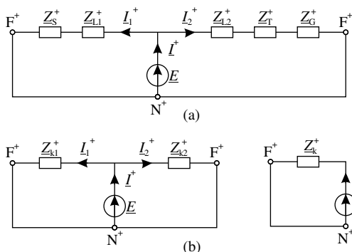
Figure 5.33. Equivalent circuit of the nonmeshed electric network from Figure 5.32: (a) positive-sequence network; (b) reduced positive-sequence network.
