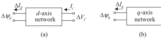
Figure 2.26. The d - and q -axis networks identifying terminal quantities.
