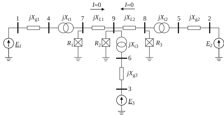
Figure 9.13. Three-area test system.
