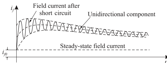
Figure 2.23. Field current of a synchronous machine during a three-phase short circuit at its terminals.
