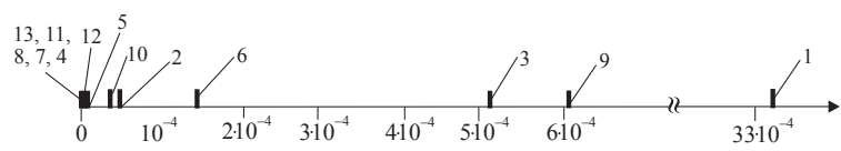
Figure 10.21. Location on the number axis of disturbance impact indices for generators.
