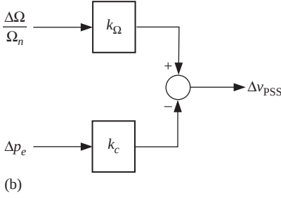
Figure 9.60. (a) General block diagram of PSSs on excitation control of units; (b) its simplification in case of systems with dominantly thermal generating units.
