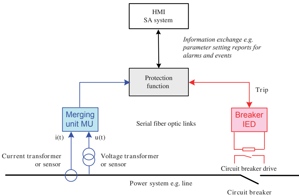
Figure 12.8. Protection chain with serial links.
