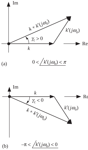
Figure 9.26. Stabilizing and destabilizing effects of the transfer function k'(s) : (a) stabilizing effect; (b) destabilizing effect.
