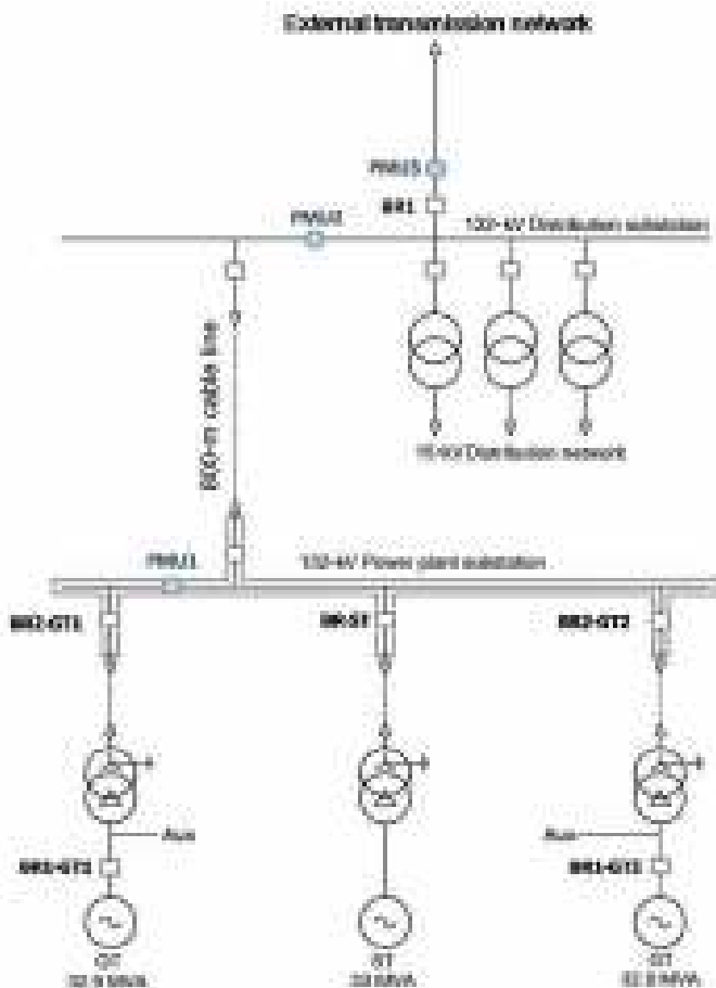
Figure 14.10. Scheme of the simulated power plant and the local network. (PMU1, PMU2, and PMU3 indicate the position of the three-phasing measurement units installed during the experimental tests described in Section 14.3.2.3.)
