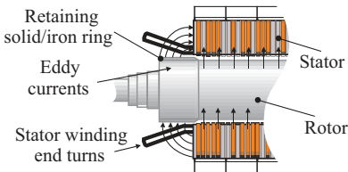
Figure 2.43. View of stator winding end region.
