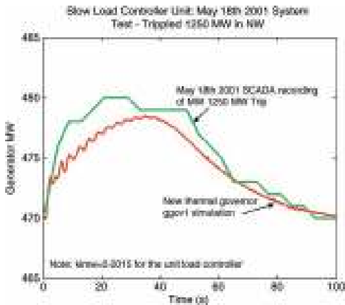
Figure 6.37. Simulations of a thermal unit with a “slow” load controller of Code T2 compared with its May 18, Test SCADA recordings.
