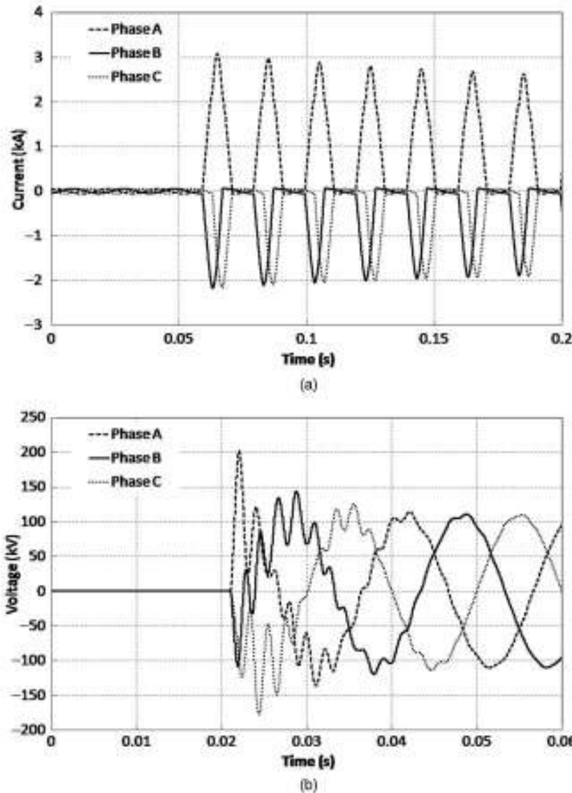
Figure 14.11. Transients during network component energization: (a) generator currents during TR-GT1 energization; (b) 132-kV distribution substation phase voltages during cable line energization; (c) generator currents during the energization of TR-D1 feeding a 0.58-MW and 0.28-MVar load.
