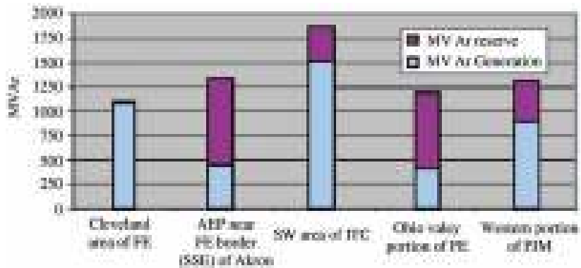
Figure 13.2. Reactive reserves of representative groups of generators at 04:00 p.m. on August 14, 2003. AEP, American Electric Power system operator.
