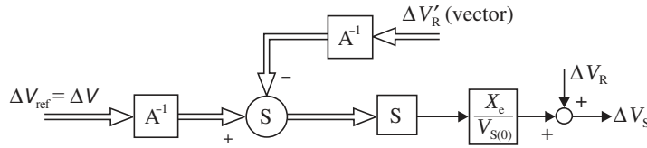
Figure 7.43. Linear equivalent model of a power plant with n generators, connected to an equivalent grid: link between the generators and the EHV bus bar voltages.
