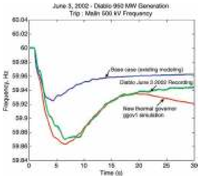
Figure 6.40. Governor model verification—950 MW Diabolo generation trip in California on June 3, 2002.
