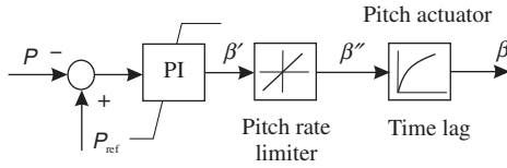
Figure 4.20. Pitch control for active stall wind turbine [8].
