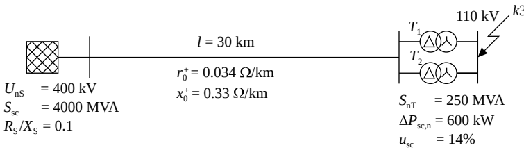
Figure 5.30. Radial electric network fed from one source.
