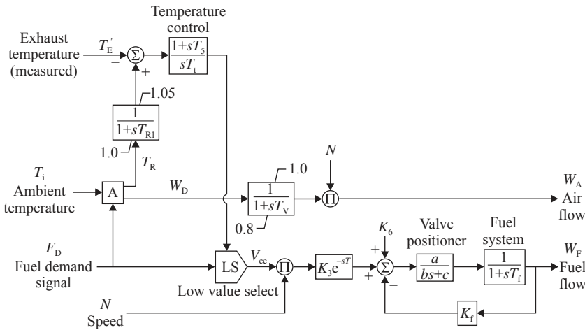
Figure 3.31. Gas turbine fuel and airflow controls. (Reprinted with permission from Ref. 11. © 1994 IEEE.)
