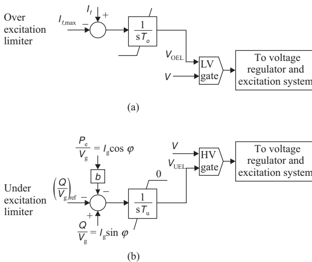
Figure 2.62. The block diagram of the over- and underexcitation limiters [12].
