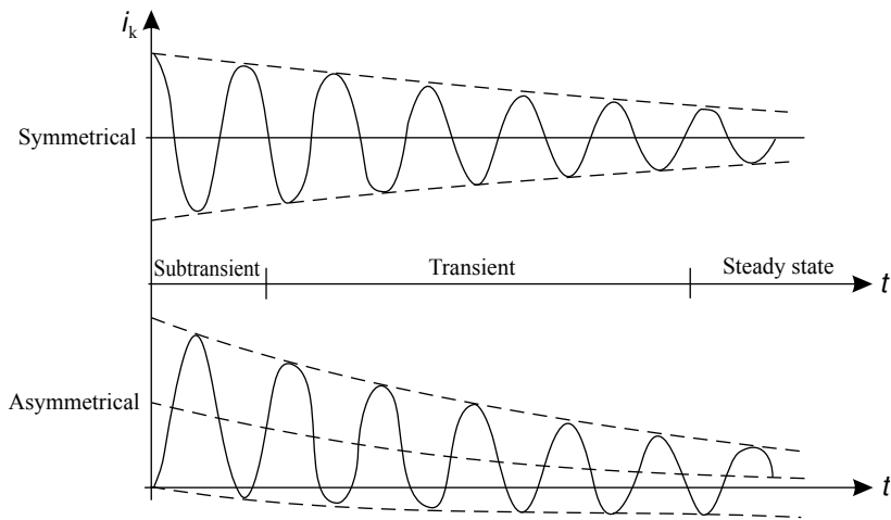
Figure 5.4. Short-circuits current near a generator [2].
