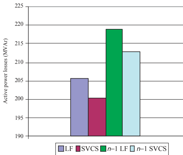
Figure 7.71. Active power losses of the system.
