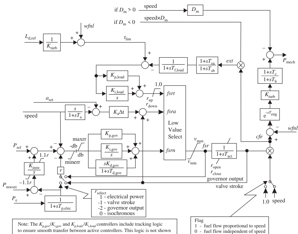
Figure 6.28. General thermal turbine governor model ggov1 (GE-PSLF stability program) described in Section 6.5.5 for steam and gas turbines.
