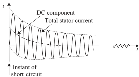
Figure 2.21. Stator current upon a short-circuit occurrence.
