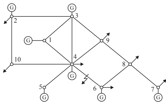
Figure 10.12. A 225 kV CIGRE test network.
