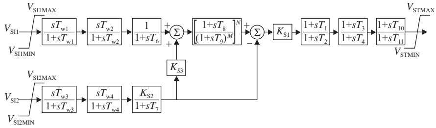
Figure 2.67. Type PSS2B—dual-input power system stabilizer. (Reprinted with permission from Ref. 36.)
