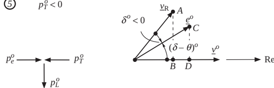
Figure 9.40. Unit in generation mode in the same operating point ( e^o , v^o , (\delta - \theta)^o , p_e^o are const.): effect of the decrease in real transit p_T^o with the increase in real load p_L^o .
