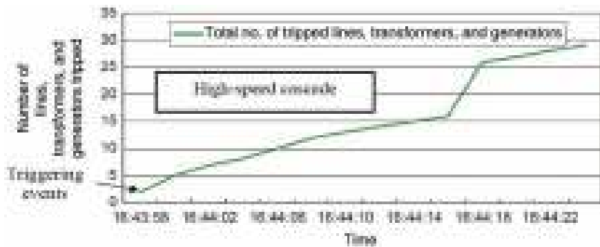
Figure 13.29. Accumulated lines, transformers and generators tripping during the cascade in Croatia blackout on January 12, 2003 [16].
