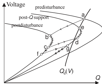
Figure 8.9. Voltage dynamics as viewed from the V - Q plane [20].
