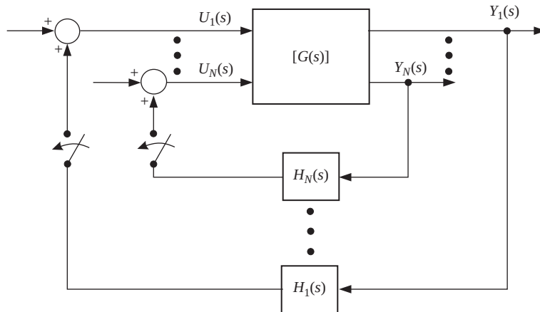
Figure 9.61. Local additional feedbacks.
