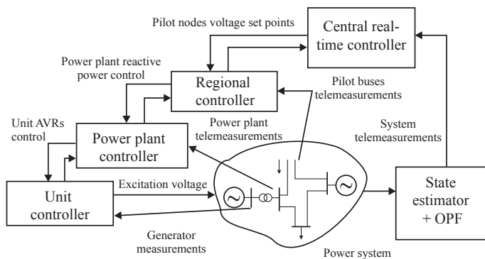
Figure 7.52. A hierarchical structure for transmission network voltage control.
