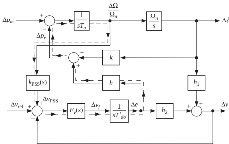
Figure 9.63. Effect of PSSs on voltage loop.
