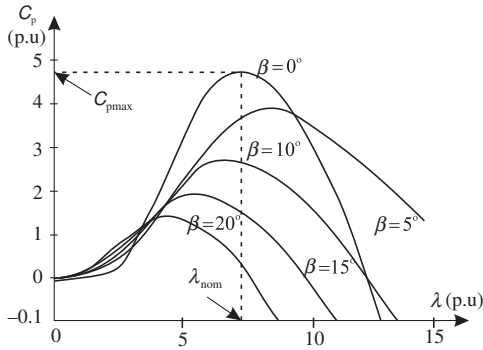
Figure 4.5. C_p(\lambda, \beta) characteristics with control of the blade pitch angle [1].
