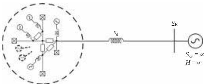
Figure 9.67. Highly meshed area connected to the rest of the system via a long line.
