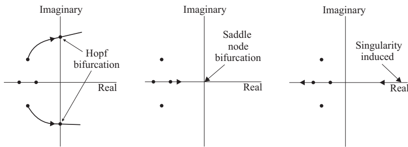
Figure 11.22. Locus of the eigenvalues close to three types of bifurcation to changes in the loading parameters [43].
