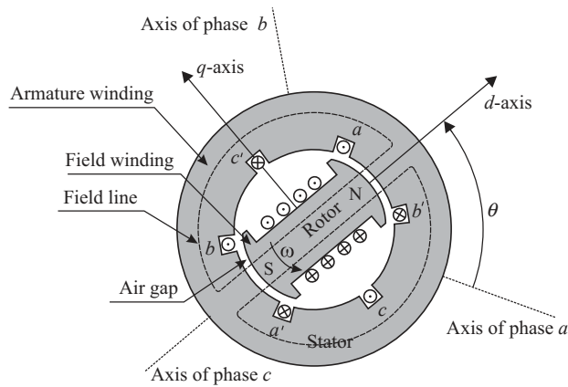
Figure 2.1. Schematic diagram of a three-phase synchronous machine.
