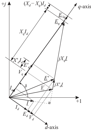
Figure 2.35. Synchronous generator phasor diagram with damper winding neglected, under transient conditions, in terms of E_q , E_{Iq} , and E'_q .
