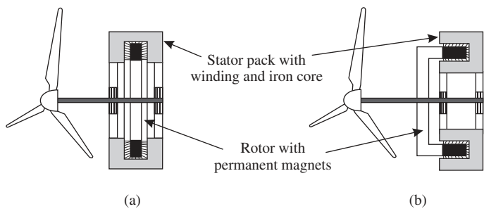
Figure 4.12. Schematic representation of double air gap designs for machines with (a) axial; (b) radial air gap. (Reproduced from Ref. 6.)
