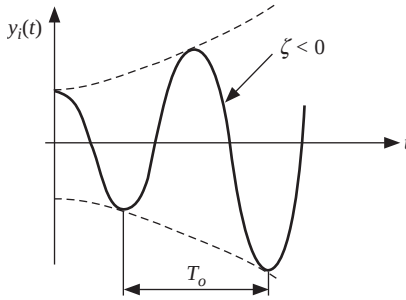
Figure 9.18. Undamped electromechanical oscillation.
