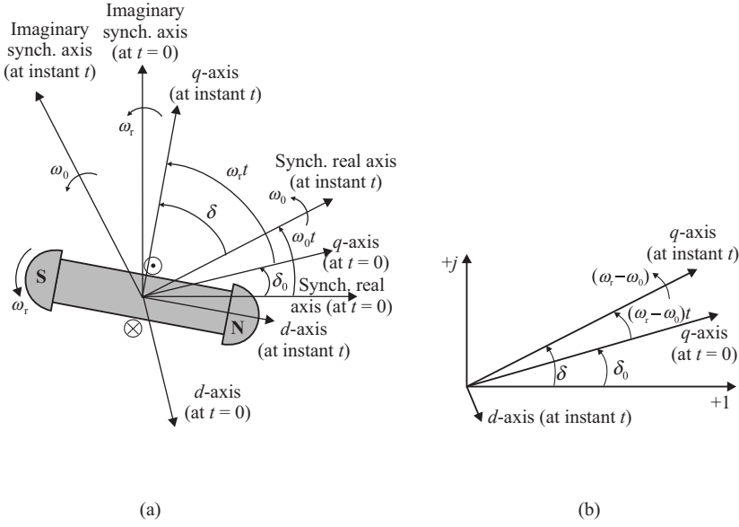
Figure 2.4. The definition of angles.
