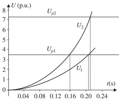
Figure 10.11. Estimation of critical clearing time by different ways of applying the Lyapunov function method.
