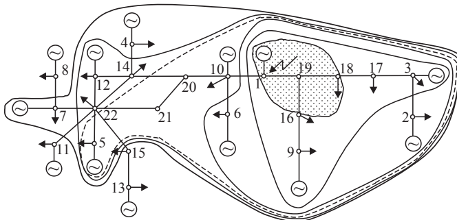
Figure 10.23. Decomposition of a system on the basis of disturbance impact index.
