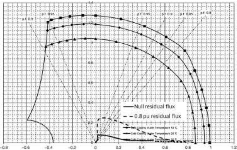
Figure 14.12. Comparison between GT1 P - Q trajectories during the TR-GT1 energization and the synchronous machine capability limits.
