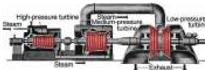
Figure 3.2. The structure of a steam turbine.
