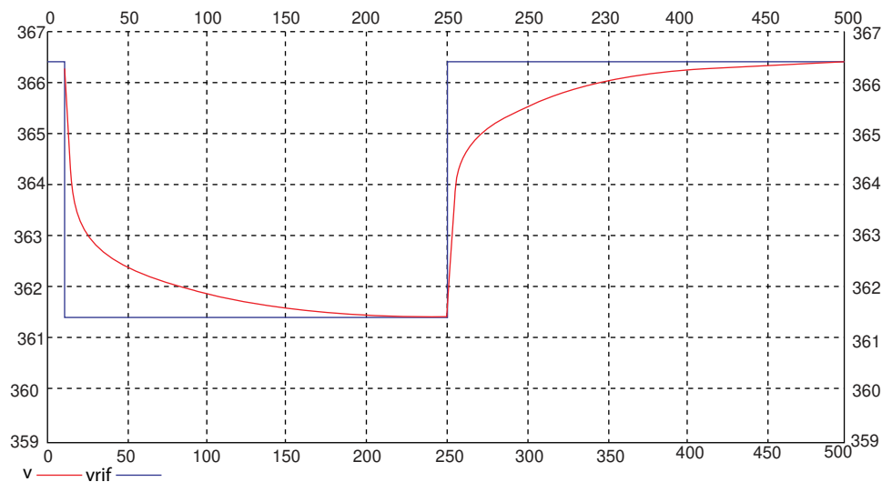
Figure 7.48. Transients of the power plant high-side bus bur voltage V_s following step variations of the HSVC voltage set point.
