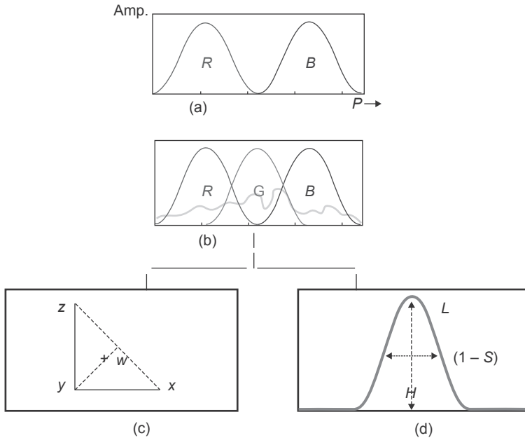
Figure 22.1 The nature of non-orthogonal sensors
