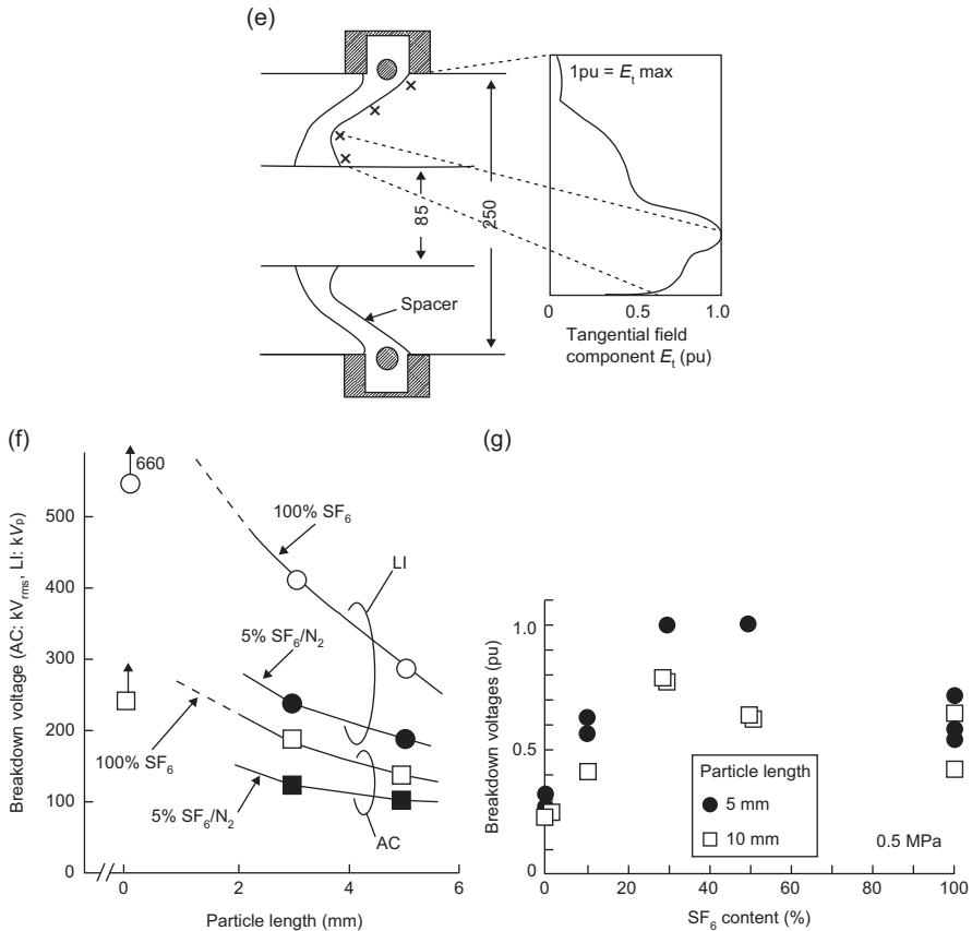
Figure 3.11 Further breakdown characteristics in \text{N}_2 - \text{SF}_6 mixtures [18]
