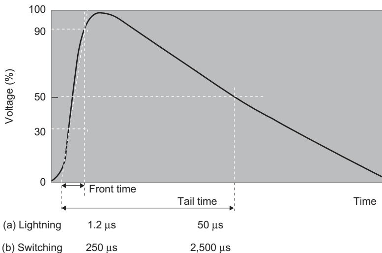
Figure 2.6 Impulse voltages to determine standard insulation levels (a) is for lightning impulse voltage 1.2/50 μs and (b) is for switching impulse voltage 250/2,500 μs
