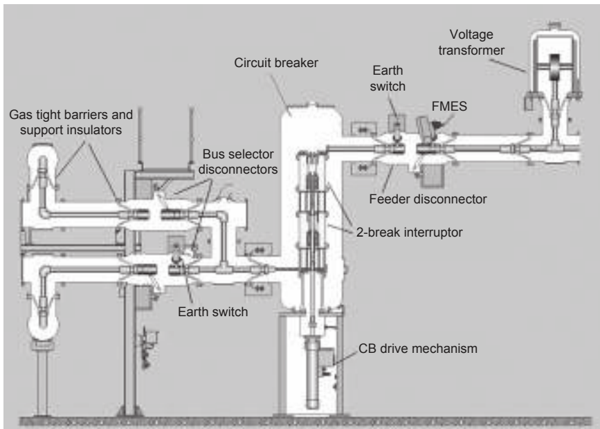
Figure 21.6 Typical 420 kV GIS bay cross section
