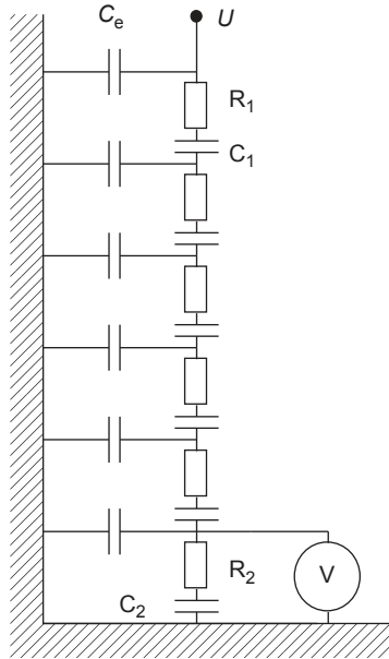
Figure 15.18 Damped capacitive voltage divider
