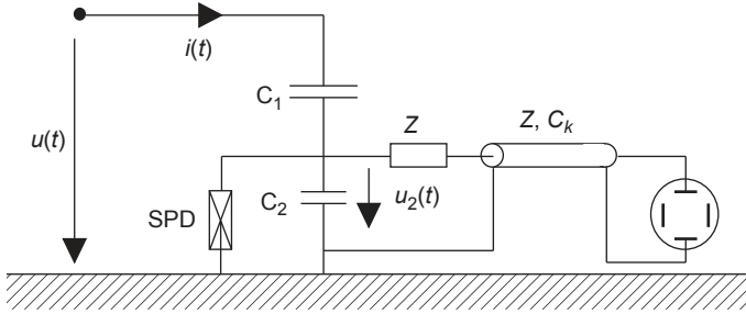
Figure 15.19 Equivalent circuit of a capacitive divider
