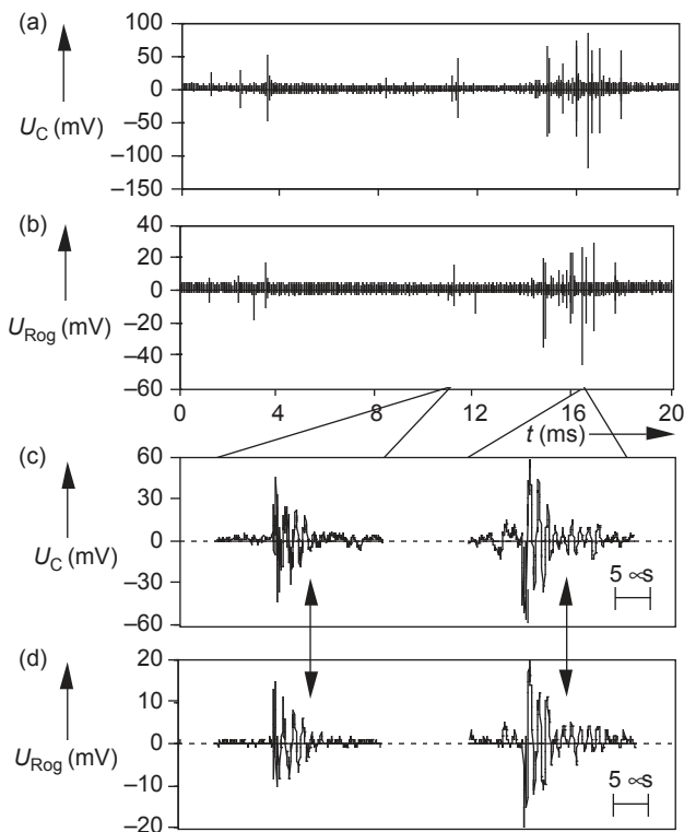
Figure 17.8 Example of more advanced partial discharge signal techniques
