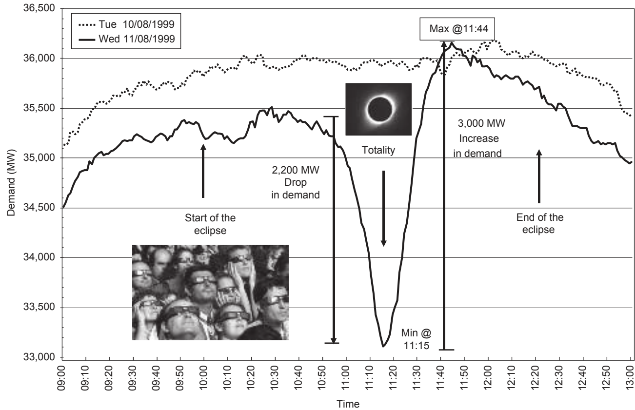
Figure 1.8 Effect of the total solar eclipse on NGC demand – 11 August 1999
