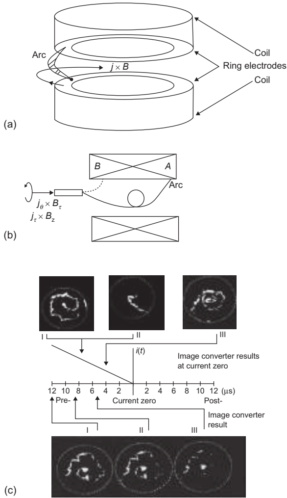
Figure 7.13 Electromagnetic interrupters
