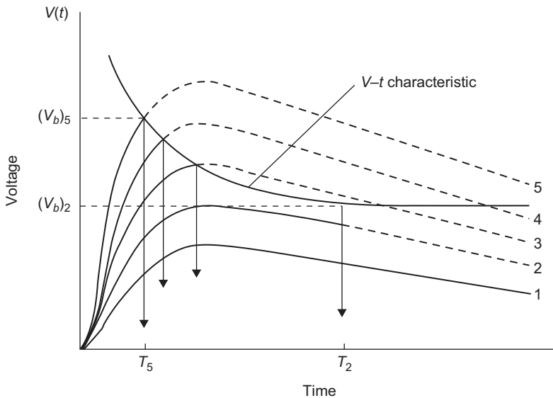
Figure 19.19 Voltage-time characteristics
