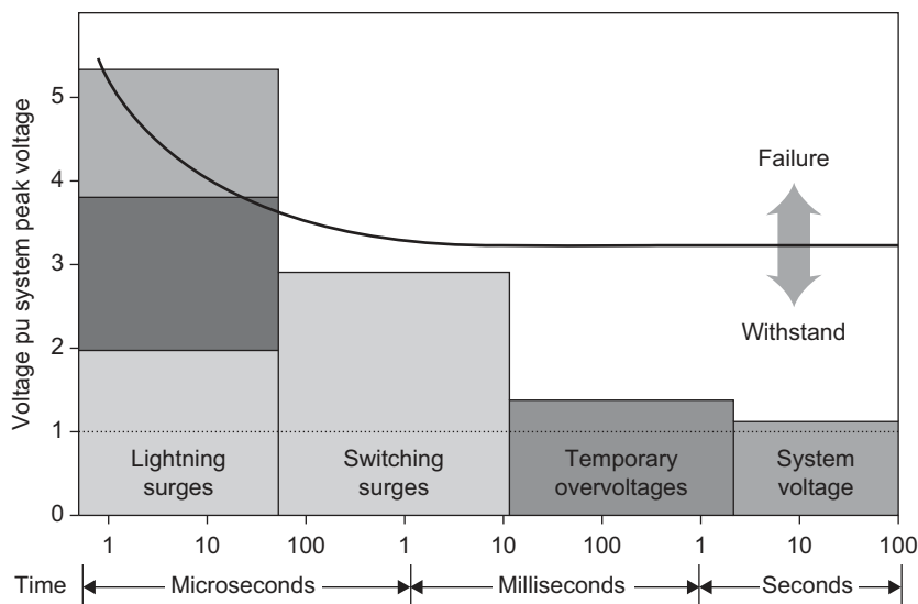
Figure 2.4 Voltage–time characteristics
