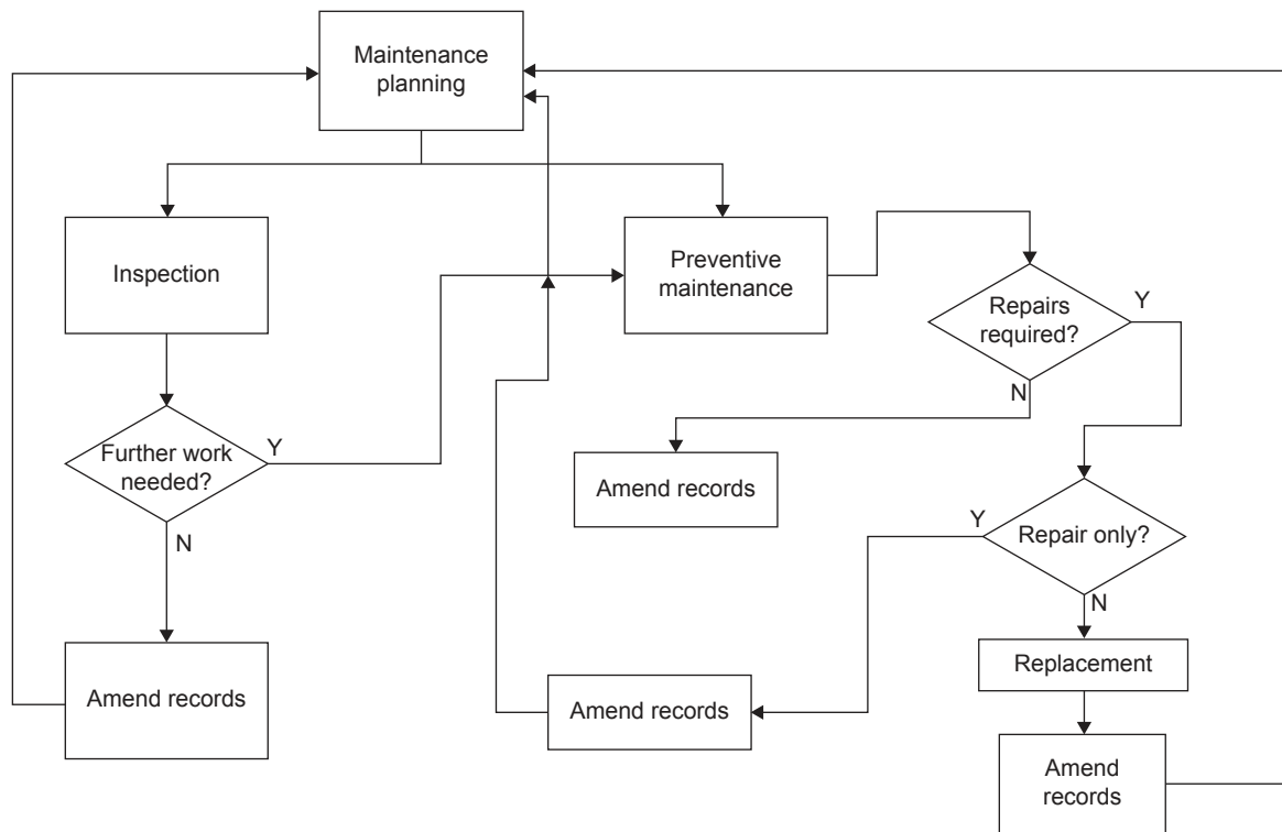
Figure 11.8 Simplified maintenance flow diagram
