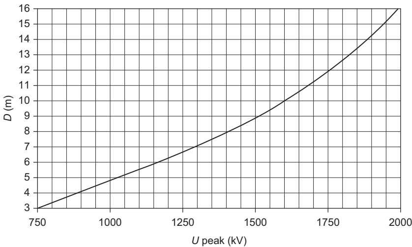
Figure 19.25 Test clearances [4]
