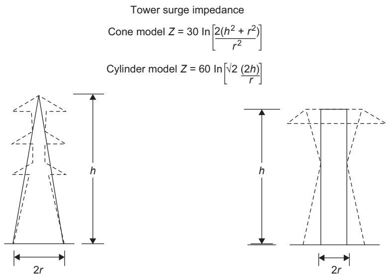
Figure 2.24 Tower surge impedance
