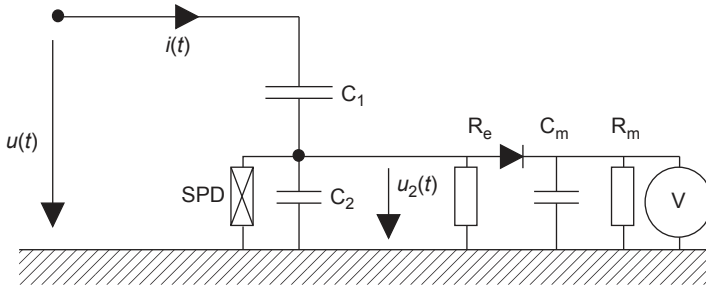
Figure 15.16 AC peak value measuring circuit with a capacitive divider
