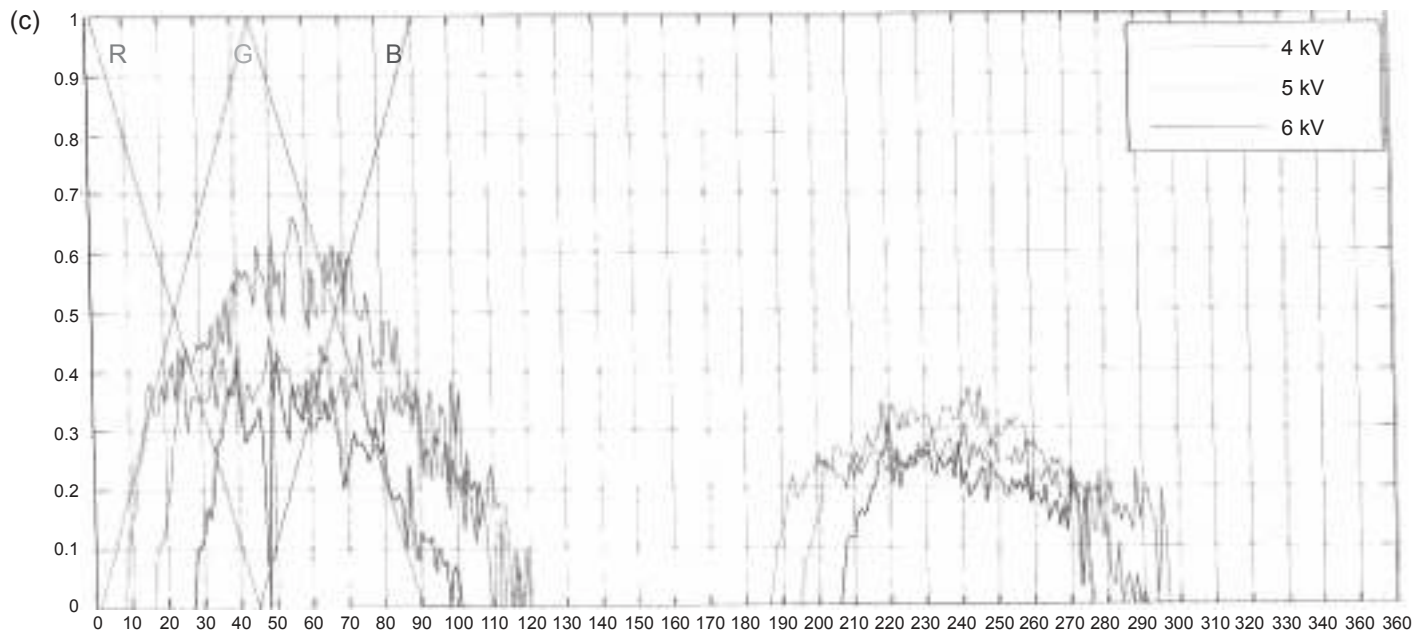
Figure 22.8 Partial discharge signals for 50 Hz voltage oscillations
