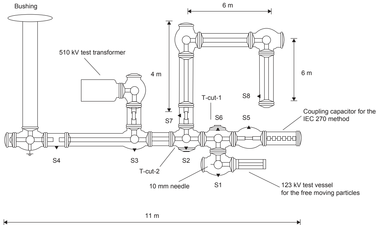
Figure 17.10 Set-up for a UHF partial discharge measurement on a gas-insulated substation
