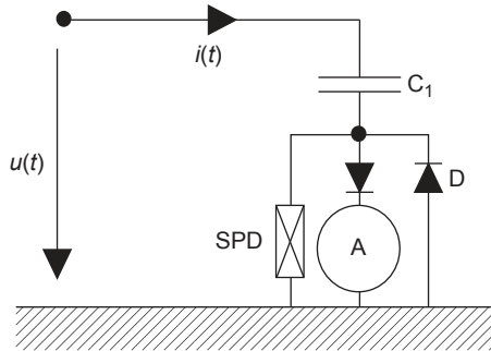
Figure 15.15 AC peak value measuring circuit
