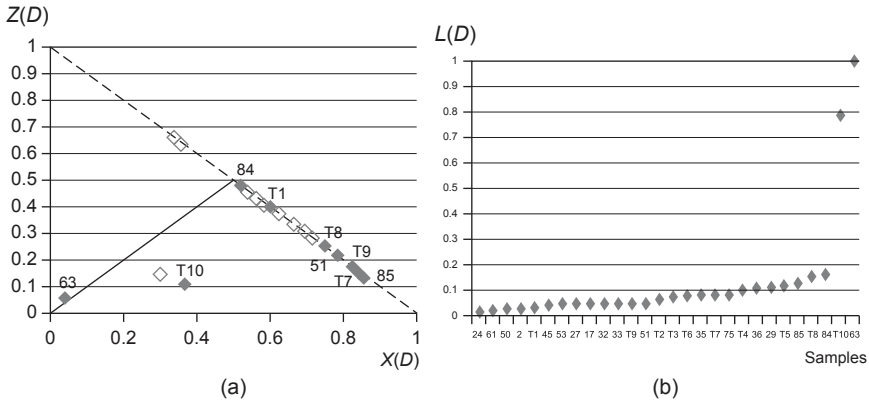
Figure 22.12 Chromatic representation of dissolved gases in transformer oils (a) z : x Chromatic Cartesian diagram of severe overheating ( z(D) ) versus electrical discharging ( x(D) ) with local overheating ( y(D) ) as parameter (equi-distribution point – 0.33, 0.33) (b) Chromatic strength of dissolved gases for the various oil samples of Figure 22.6 in ascending order
