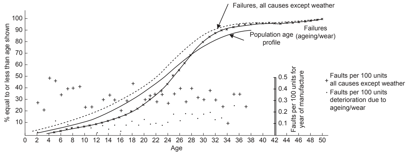
Figure 11.4 Pole mounted transformers: cumulative failures and age profile (1985/86)
