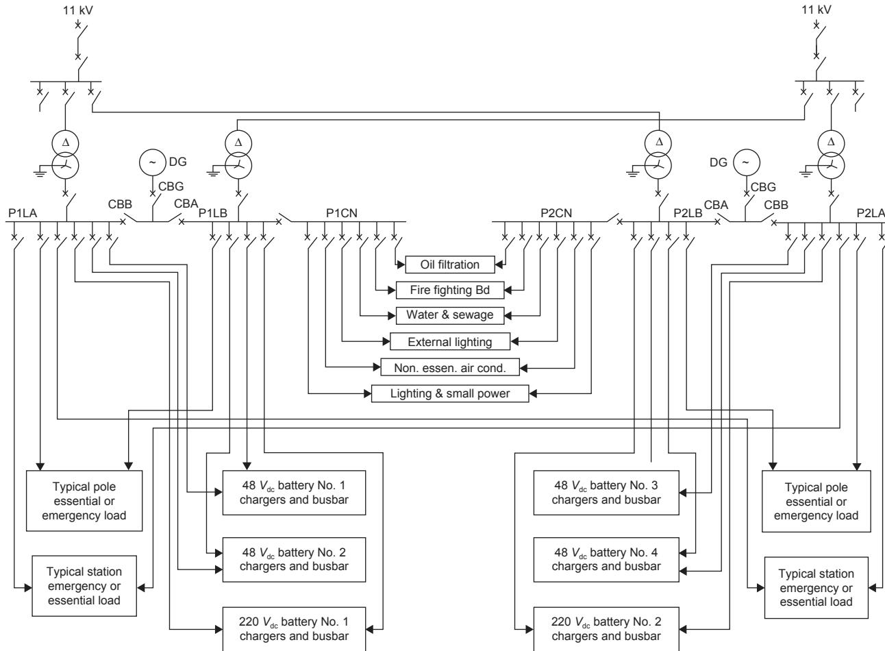
Figure 4.9 AC auxiliary power supply scheme for converter station
