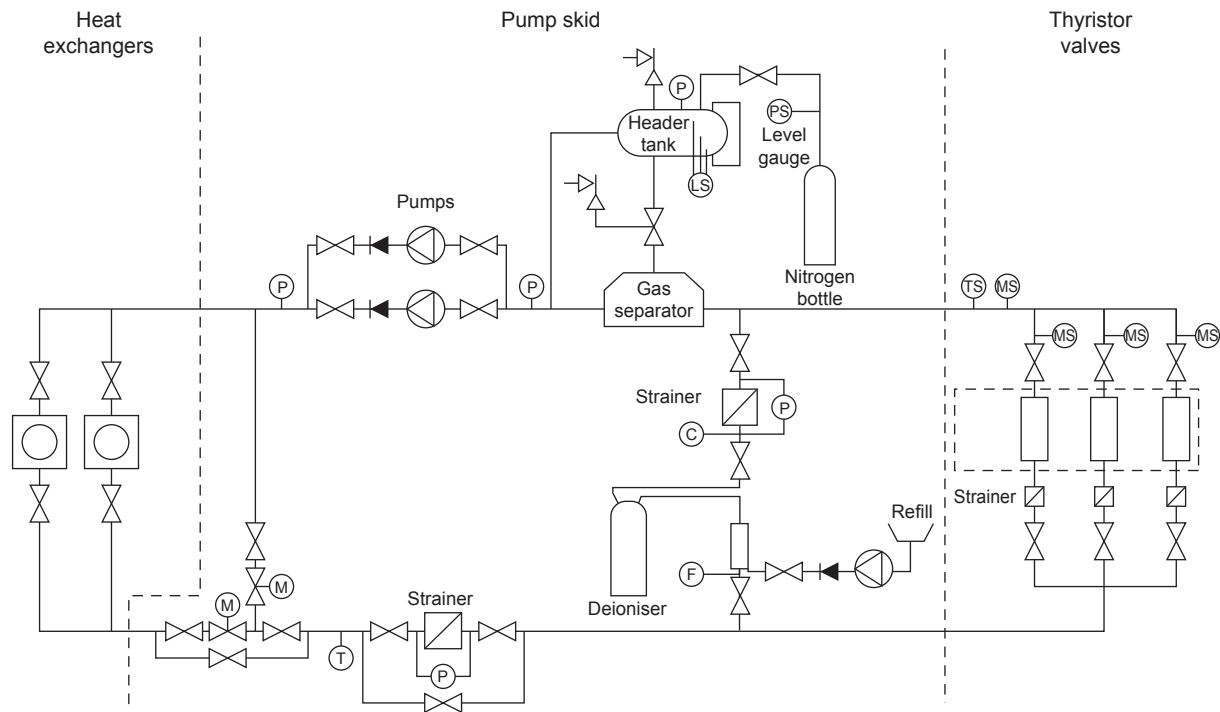
Figure 4.8 Typical cooling plant diagram
