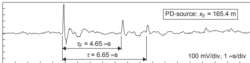
Figure 17.9 Partial discharge measurement and location on a cable on-site
