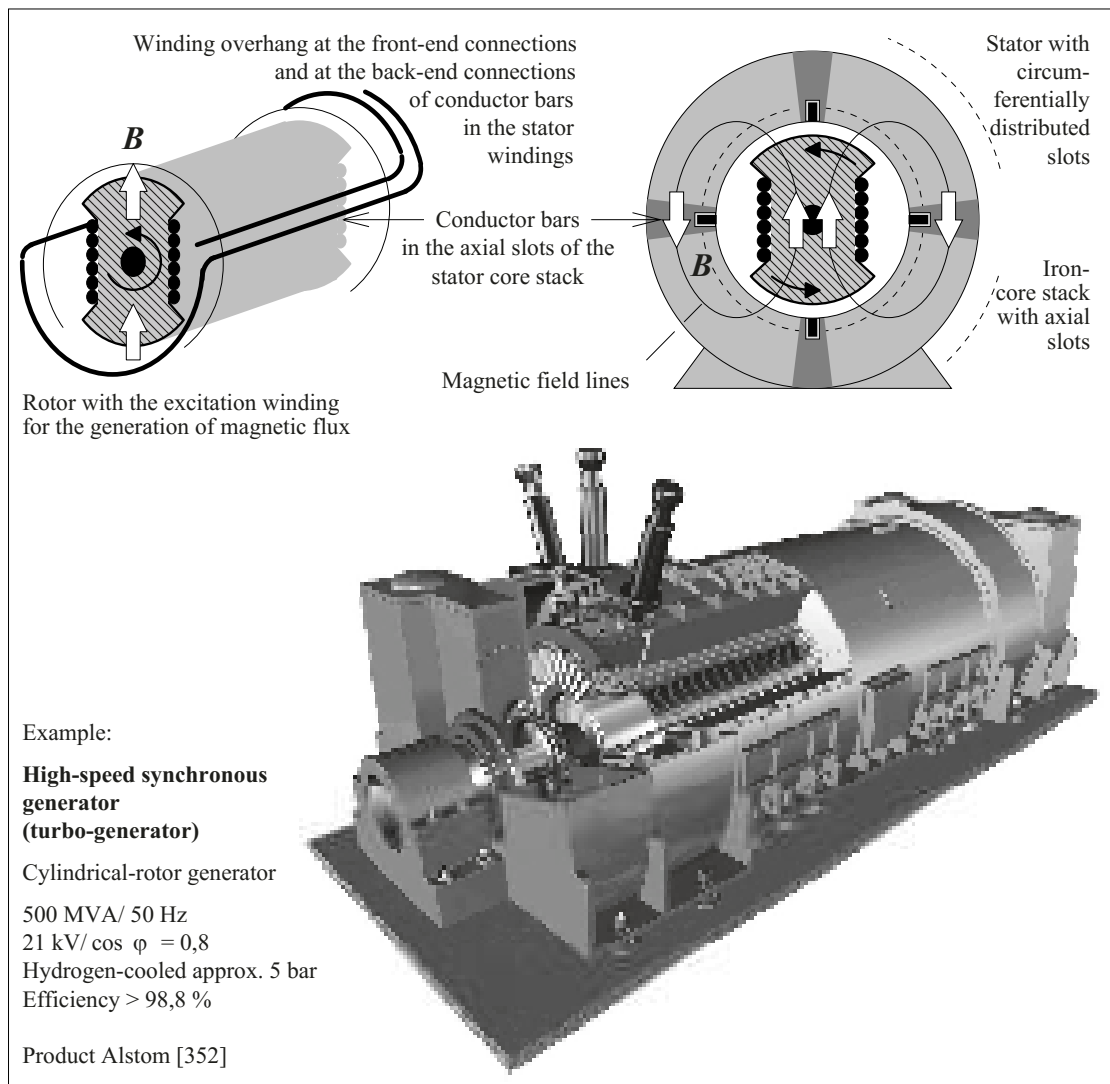
Figure 7.1.6-1: Principle and construction of an electrical synchronous machine (schematic).
