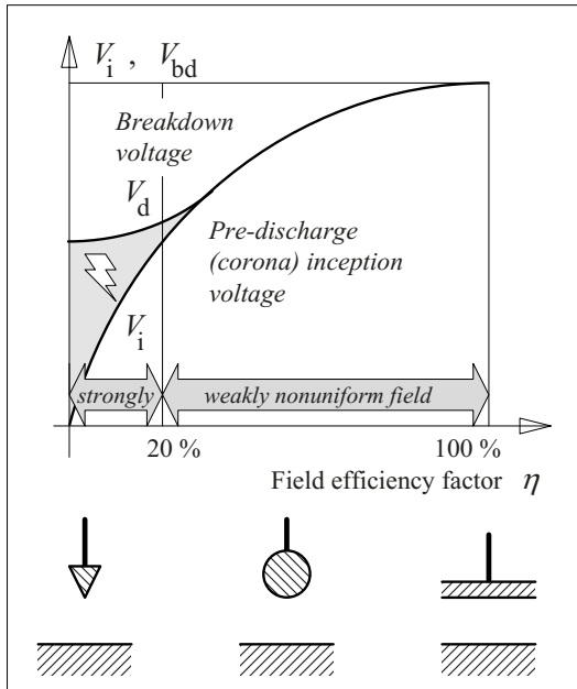
Figure 3.2-24: Pre-discharge (corona) inception and breakdown voltage in strongly and weakly non-uniform fields at constant electrode distances.
