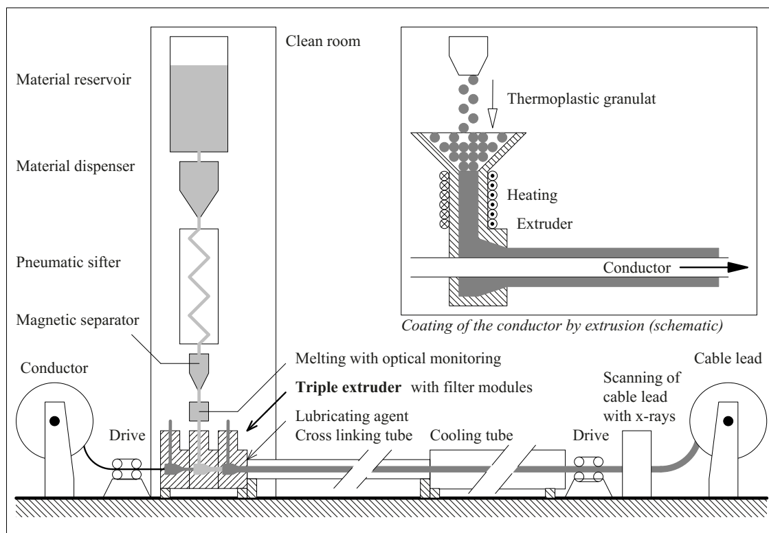
Figure 5.3-3: Manufacturing a high voltage XLPE cable lead by triple extrusion in a horizontal procedure.
