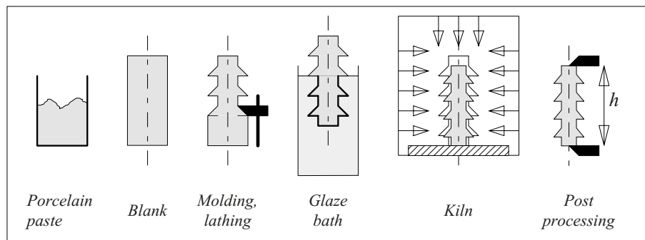
Figure 5.2-2: Manufacture of porcelain insulators
