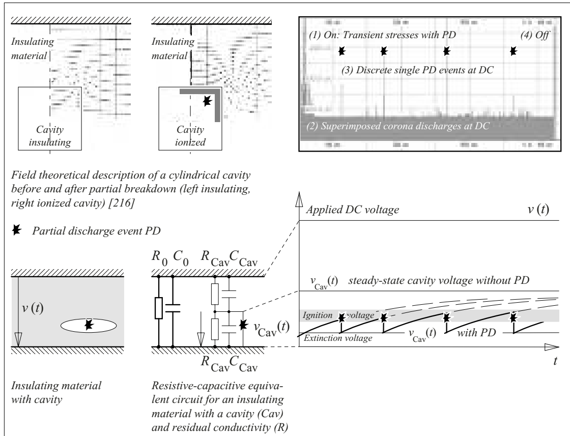
Figure 3.6-5: Internal partial discharges (PD) at DC voltage in a gas-filled cavity.
