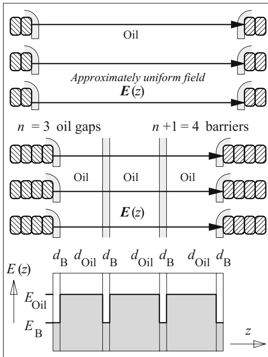
Figure 7.1.3-8a: Transformer leakage flux gap between two windings with a large oil gap (top) and with barriers for subdividing it into electrically stronger subgaps with smaller volumes (center and bottom) [274].
