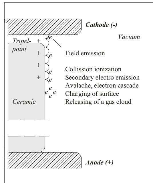
Figure 3.7-3: Reduced surface strength in vacuum.
