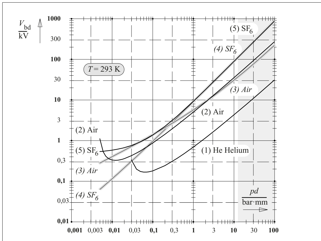
Figure 3.2-14: Calculated breakdown voltages as function of pd (Paschen curve) for different gases:
