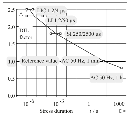
Figure 7.1.3-13: Design values for the electric strength of oil gaps as a function of stress duration in comparison to the one-minute AC voltage strength (r.m.s. value), expressed as a Design Insulation Level (DIL) [274].
