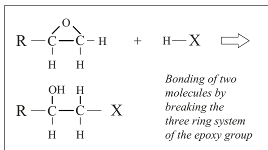
Figure 5.3-9: Reaction of the epoxy group.
