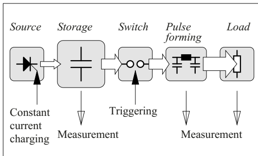
Figure 7.4.2-1: Impulse generator (schematic).
