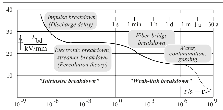
Figure 3.4.1-1: Breakdown strength of a liquid dielectric as a function of voltage-stress time (transformer oil, d = 2.5 \text{ mm} , V = 200 \text{ mm}^3 ) without respect to the statistical dispersion which increases with time, see fig. 3.4-2.
