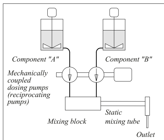
Figure 5.3-16: Principle of a two-component mixer (simplified).
