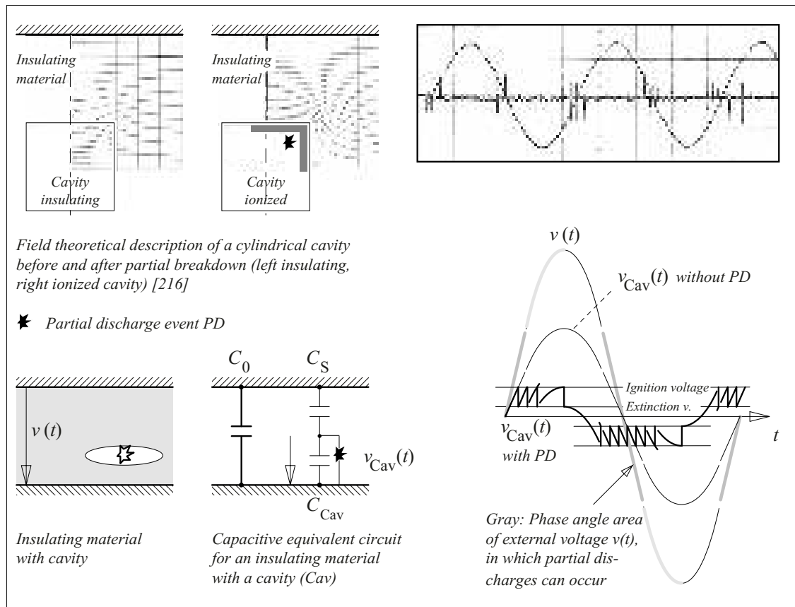
Figure 3.6-2: Internal partial discharges (PD) at AC voltage in a gas-filled cavity.
