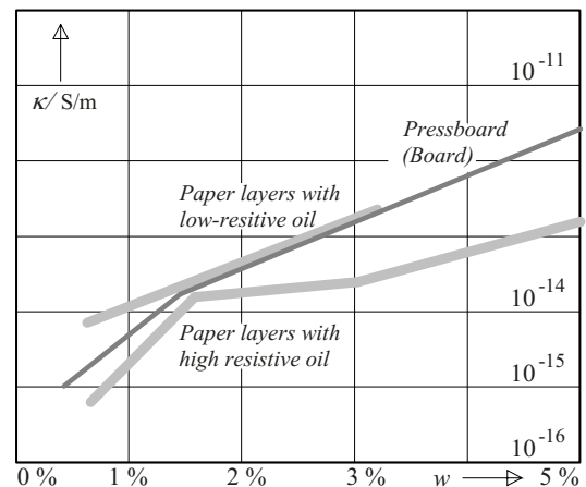
Figure 5.5-5: Conductivities of oil-impregnated paper OIP (light grey curves) and pressboard (Transformer-board, dark grey curve) for different water contents w for high and low resistive insulating oils. Schematic representation for room temperature [429], [436].
