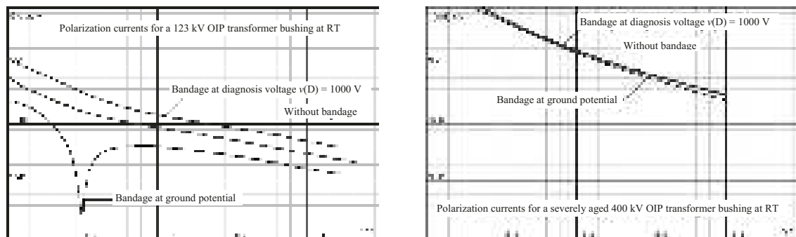
Figure 6.4.7-12: PDC measurements on high voltage bushings with bandages in the center of the grading contour ( worst-case bandages ) for demarcating the scope of the current through the bushing dielectric [428], [430], [434]. Left: new 123 kV OIP bushing. Right: severely aged and thermally unstable 400 kV OIP bushing (also refer to figure 6.4.7-9).
