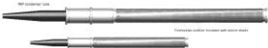
Figure 7.2.3-3: Technological leap in conjunction with the transition from 400 kV to 800 kV HVDC systems, illustrated with the example of cast-resin-impregnated RIP transformer bushings [432] (length 8.1 and 13.5 m respectively; other technical data in Table 7.2.3-2, photo HSP Hochspannungsgeräte GmbH, Troisdorf).
