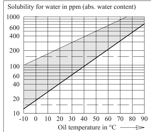
Figure 3.4.2-4: Absolute water saturation concentration in ppm as function of oil temperature for a mineral oil with low aromatic content (approx. 10 %, lower curve) and for aromatics (100 %, upper curve) [59].
