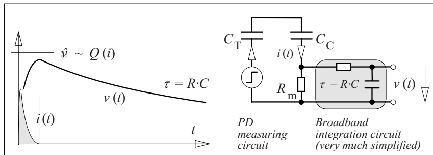
Figure 6.4.2-3: Broadband integration of a compensating current i(t) in a PD measuring circuit by a RC low pass.
