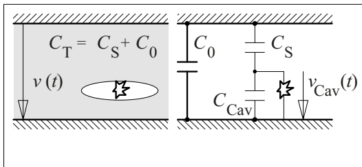
Figure 6.4.2-2: Simplified equivalent circuit for describing internal partial discharges in a test object.
