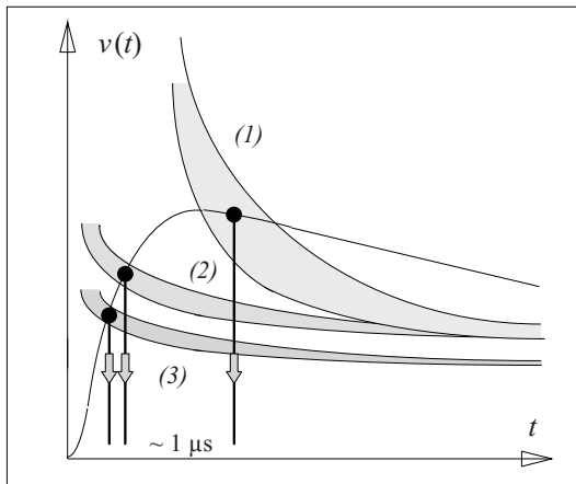
Figure 3.2-23: Voltage-time characteristics for a simple air-gap (1), an insulating gap in a GIS (2) and a lightning arrester (3).
