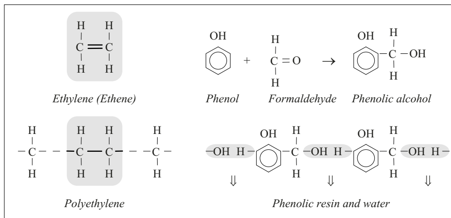
Figure 5.3-2: Examples of polymerization and polycondensation with elimination of water.
