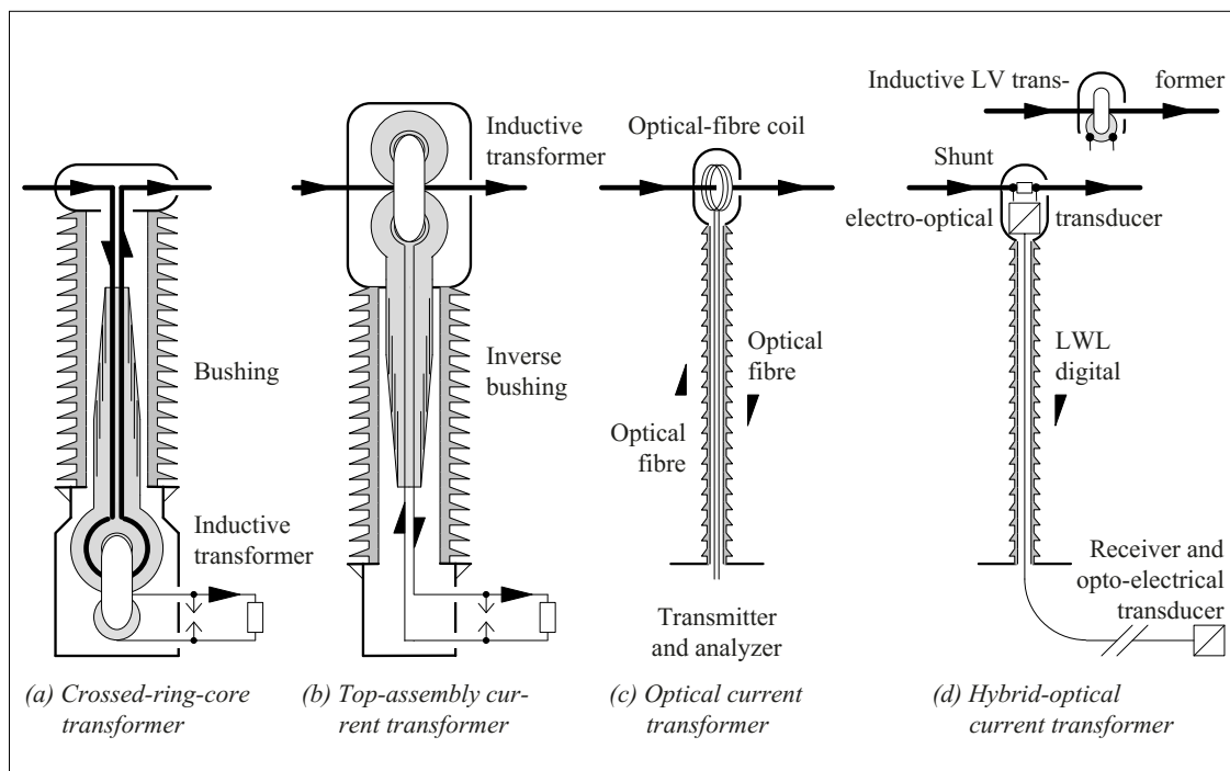
Figure 6.3.5-3: Current transformers.
