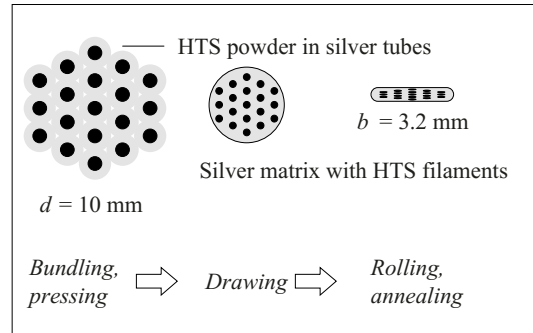
Figure 7.5.2-1: Manufacturing HTS tape conductors.
