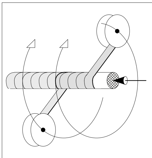
Figure 5.5-8: Winding a conductor with overlapping paper tapes (Cable or tape winding).
