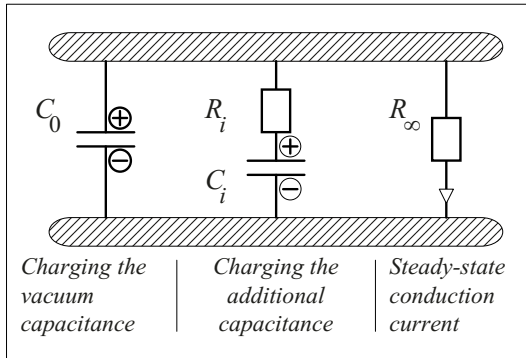
Figure 4.1-2: Network model of the dielectric.
