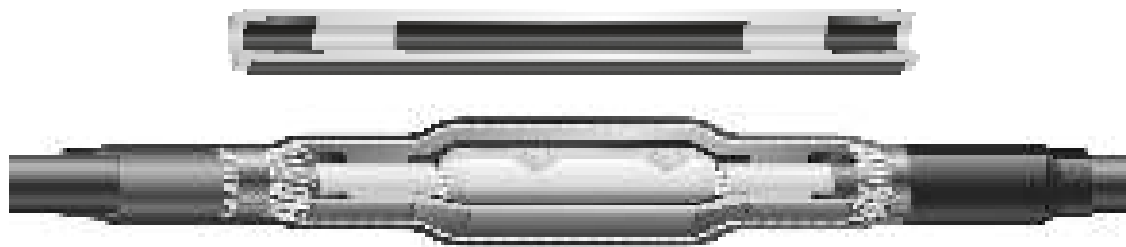
Figure 7.1.1-6: Permanent elastic connecting joint of silicone elastomer for XLPE medium voltage cables. Top: Joint body with conductive deflectors for geometric field grading (left and right, earth potential) and with "Faraday cage" for covering the metallic through connector (center, high voltage potential). Bottom: Joint mounted according to cold-shrinking technique, cf. Figure 7.1.1-7. The sheath is connected on both sides by coil springs, the outermost layer is formed by the external tube. Photos Tyco Electronics, now TE Connectivity.
