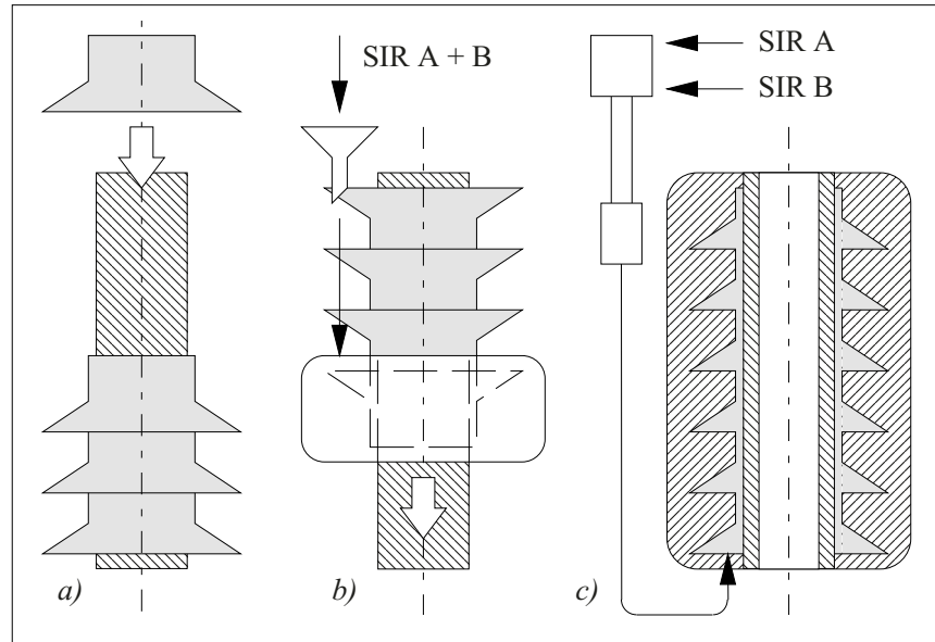
Figure 5.3-20: Manufacture silicone-shed composite insulators on a glass-fiber reinforced insulating tube or insulating rod:
