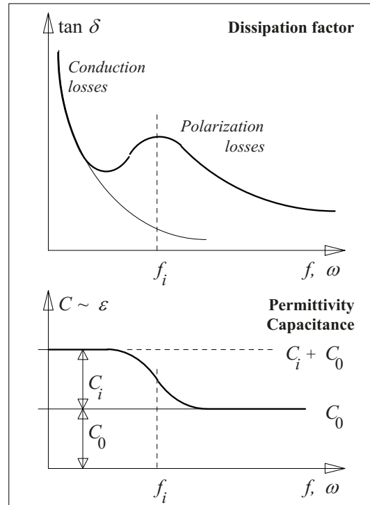
Figure 4.1-4: Dielectric parameters in the frequency domain.
