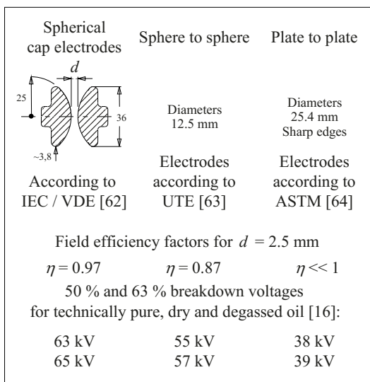
Figure 3.4.2-3: Breakdown voltages (r.m.s. values) of insulating oil in different test arrangements [16].
