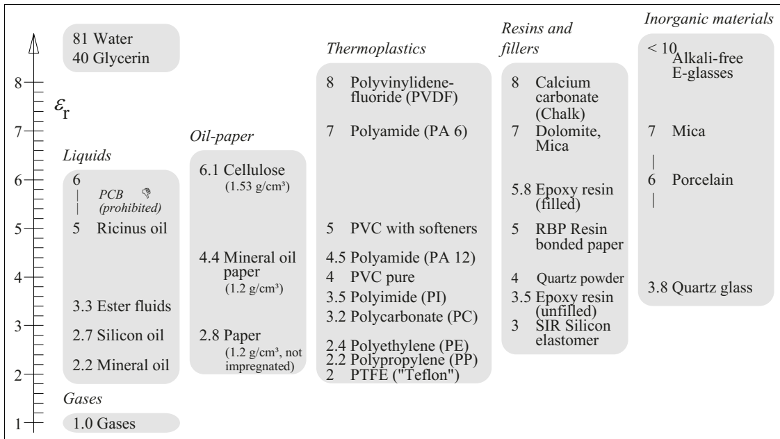
Figure 4.2-2: Permittivities of technically important materials at technical frequencies (up to 1 MHz) under atmospheric standard conditions ( T = 20^\circ\text{C} , p = 1\text{ bar} ) as orientation values.
