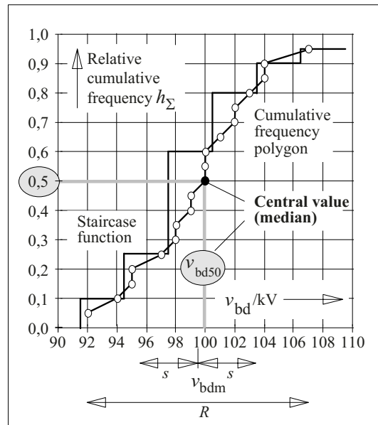
Figure 3.1-3a: Relative cumulative frequency (rate of occurrence) of measured values as empirical distribution function with and without division into classes.
