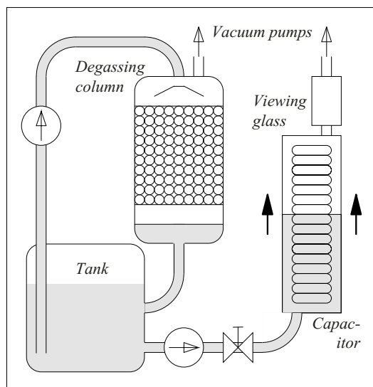
Figure 5.4-2: Processing of insulating oil and impregnation of a capacitor (schematic).
