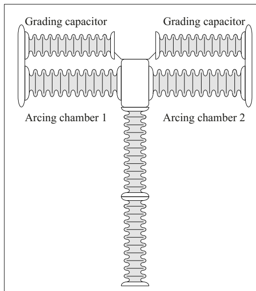
Figure 7.1.5-2: Series-connection of two circuit-breaker units in an outdoor installation (schematic).
