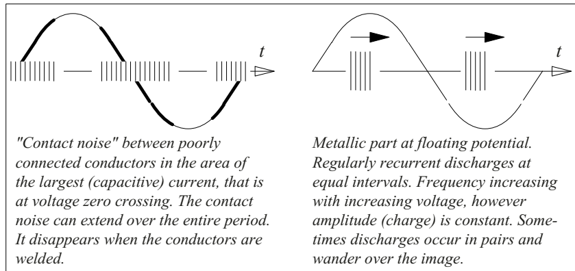
Figure 3.6-8: Characteristic partial discharge pattern for the observation with the oscilloscope. The impulse amplitude is a measure for the apparent charge [67], [72].
