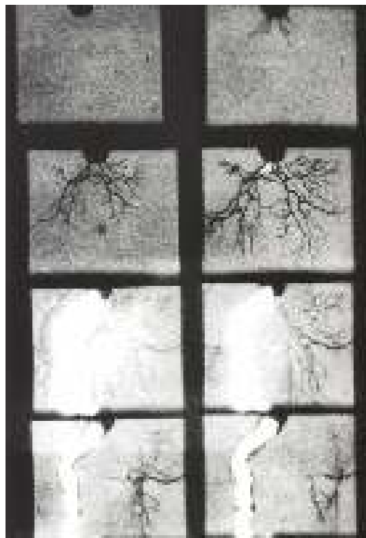
Figure 3.4.1-9: Negative discharge channels (so-called primary streamers) with branched structure [424]. For explanations see Figure 3.4.1-7.
