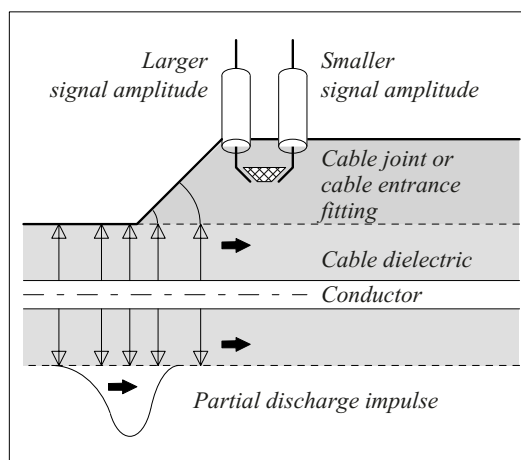
Figure 6.4.8-4: Directional coupler technique.
