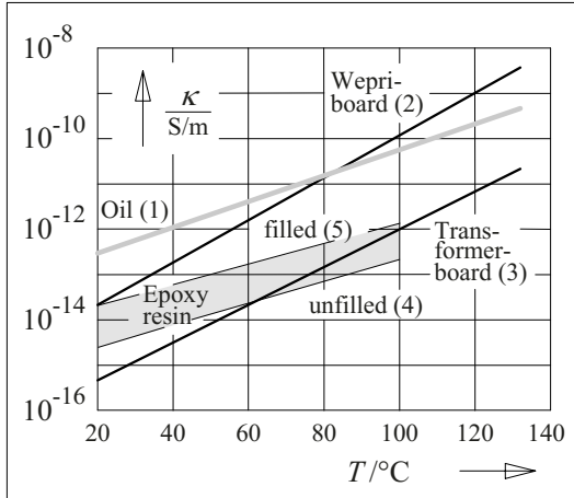
Figure 4.2-9: Temperature dependence of apparent conductivity at E = 0.5 \text{ kV/mm} (low field area).
