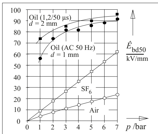
Figure 3.4.2-5: Pressure dependence of electrical strength (50 % breakdown peak-values) for ○ air at d = 2\text{ mm} (Eq. 3.2-25 with k = 5 ), □ sulfur hexafluoride at d = 2\text{ mm} (Eq. 3.2-43), ● oil at AC voltage and d = 1\text{ mm} [60], ■ as well as oil at lightning impulse voltage (1.2/50 \mu\text{s} ) and d = 2\text{ mm} [66].
