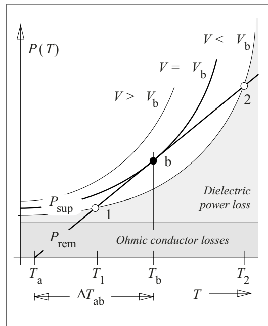
Figure 3.5-3: Balance of supplied and removed heat for thermal breakdown with stable (1) and unstable (2, b) working points for determining the so-called thermal breakover voltage.
