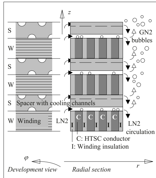
Figure 7.5.4-6: Superconducting disc winding with spacers and LN 2 /GN 2 insulation (concept).
