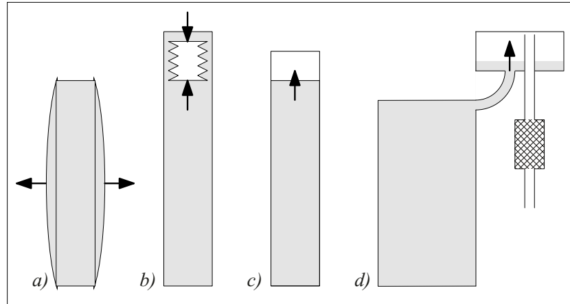
Figure 5.4-1: Compensation of thermal expansion of insulating liquids:
