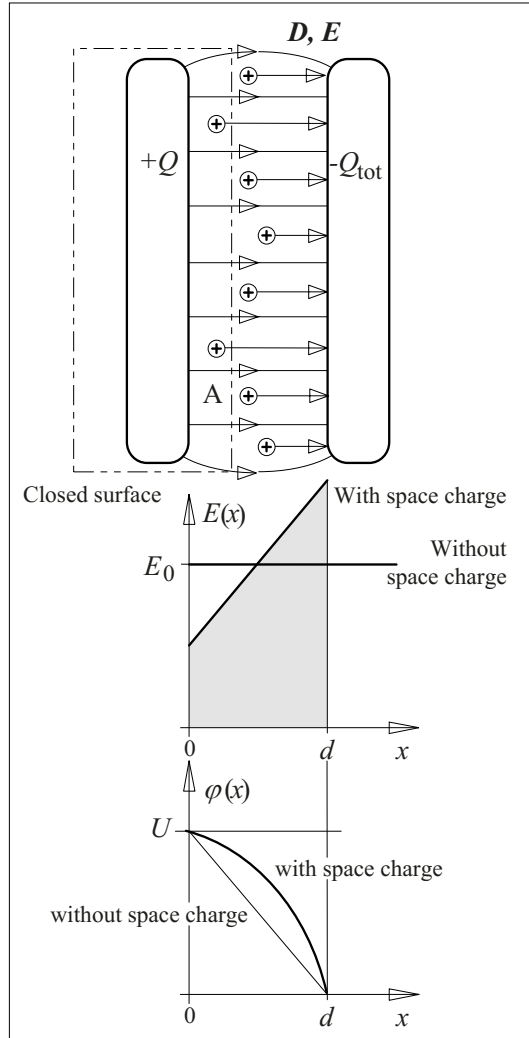
Figure 2.3-6: Space charges in the dielectric of a parallel plate capacitor (see fig. 2.3-5).
