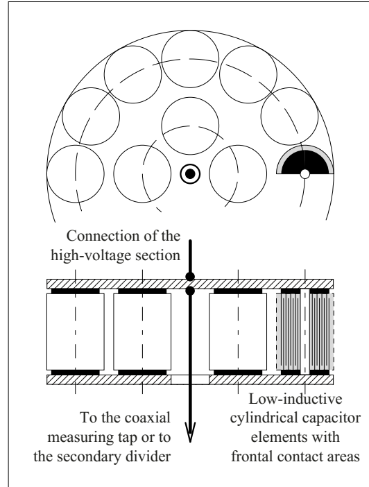
Figure 6.3.4-7: Low-inductive design of a capacitive divider's low-voltage arm.
