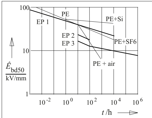
Figure 3.5-5: Lifetime characteristic for different dielectrics at AC voltage [22]:
