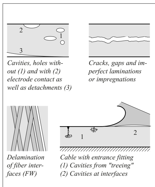
Figure 3.6-7: Partial discharge sources in solids.
