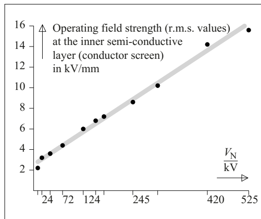
Figure 7.1.1-3: Typical operating field strengths in XLPE cables [312].
