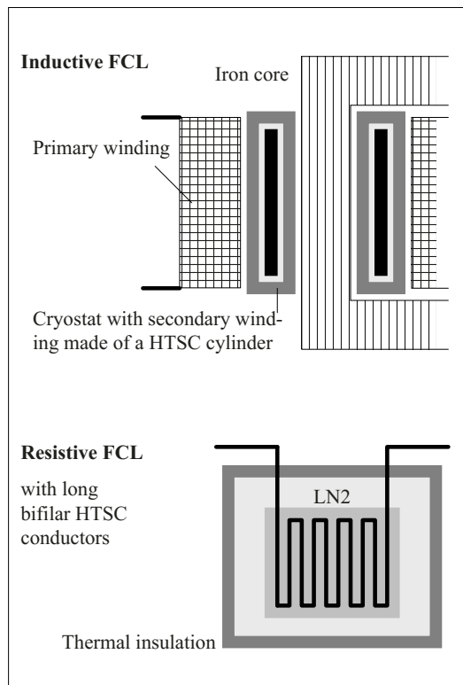
Figure 7.5.4-2: Superconducting fault current limiter (FCL), inductive and resistive principles (top and bottom).
