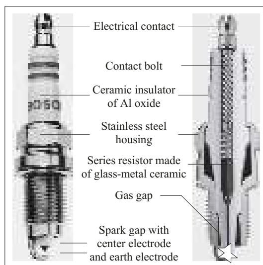
Figure 7.4.6-1: High-performance spark plug, photo Robert Bosch GmbH.
