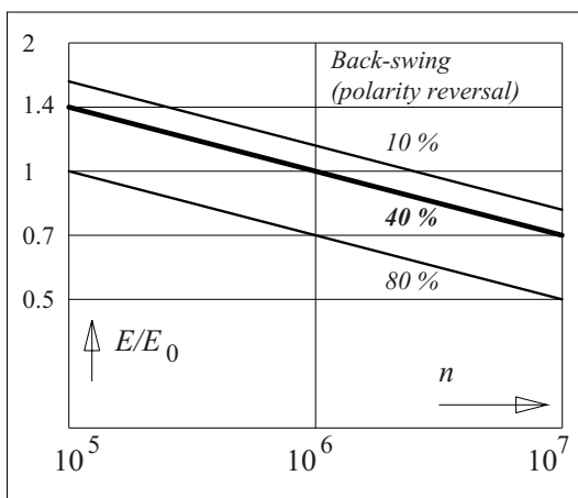
Figure 7.3-3: Service life of an impulse capacitor as a function of field stress and back-swing.
