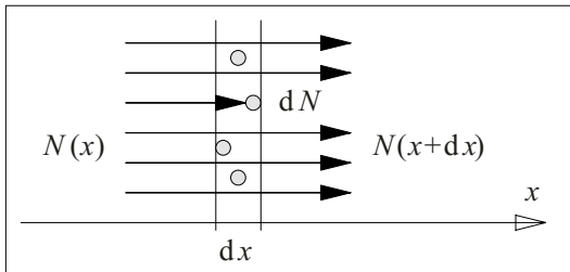
Figure 3.2-11: The Clausius law concerning path lengths.
