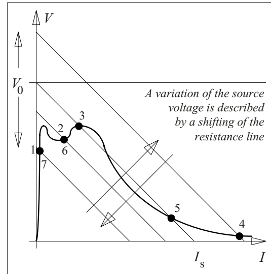
Figure 3.2-3b: Shifting of the working points along the gas discharge characteristic during the increasing of the source voltage (1, 2, 3 and 4) and during the decreasing of the source voltage (4, 5, 6 and 7) by the shifting of the resistance line.
