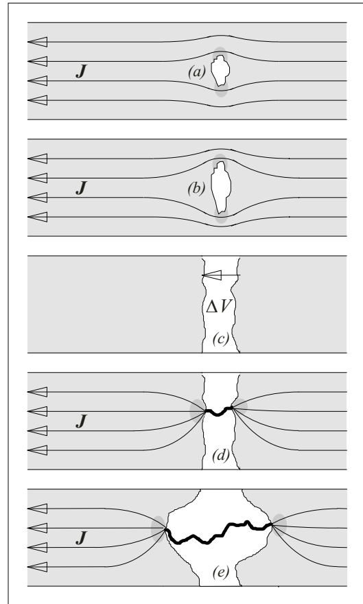
Figure 3.2-37: Phases of pollution flashover:
