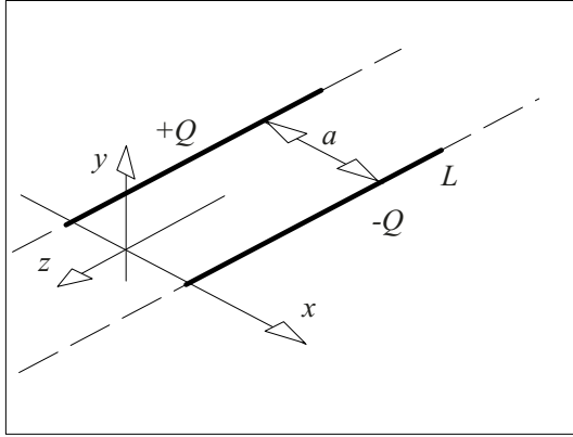
Figure 2.3-21: Infinitely long line charges in parallel (three-dimensional view).
