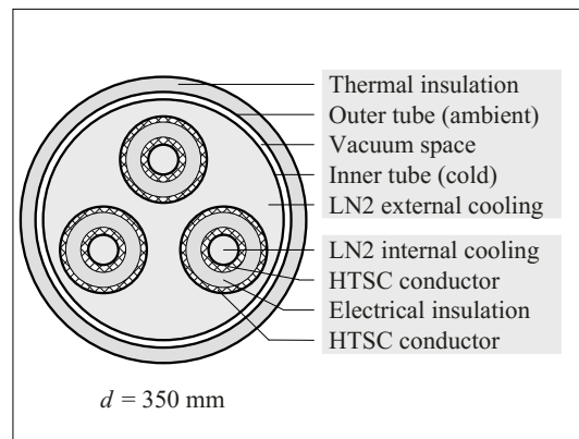
Figure 7.5.4-3: Concept of an 110 kV / 1000 MVA HTSC cable with \text{LN}_2 cooling [202].
