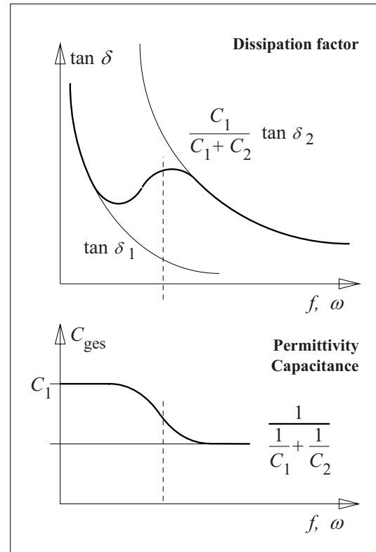
Figure 4.3-8: Maxwell's two-layer model in the frequency domain.
