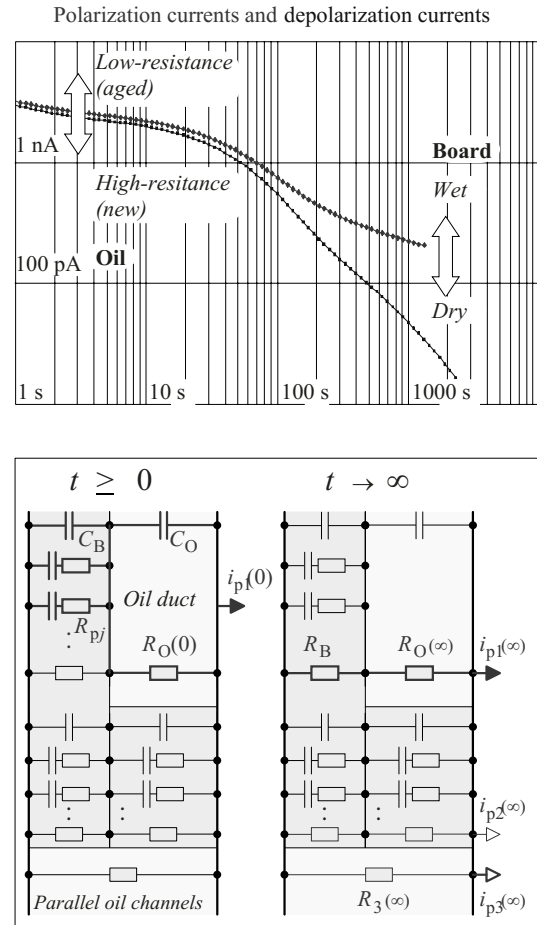
Figure 6.4.7-10: Differtiation of characteristic equivalent circuit elements by a selection of different measuring times.
