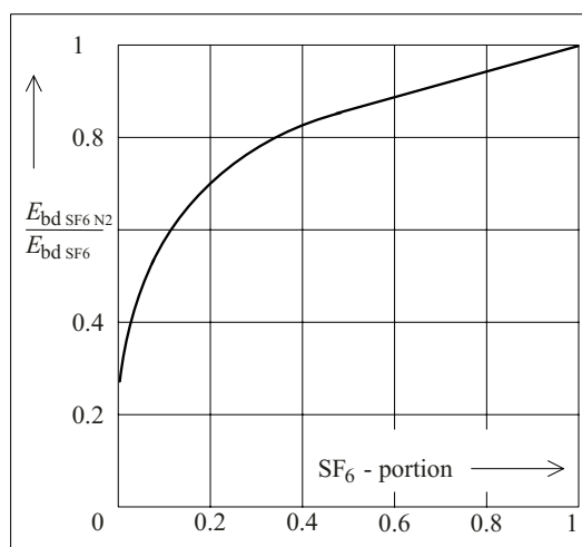
Figure 5.1-2: Electrical strength of mixtures of nitrogen and sulfur hexafluoride [22].
