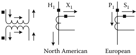
FIGURE 6.4 CT polarity marking
