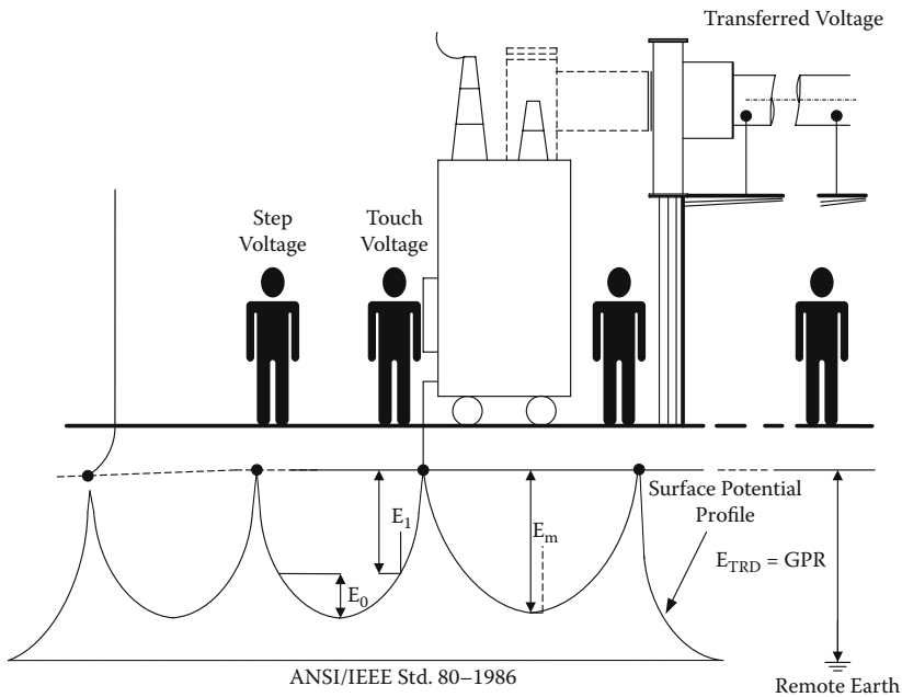
FIGURE 13.6 Basic shock situations
