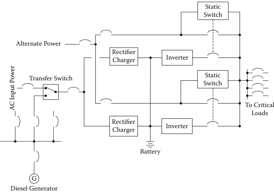
FIGURE 2.3 Redundant UPS
