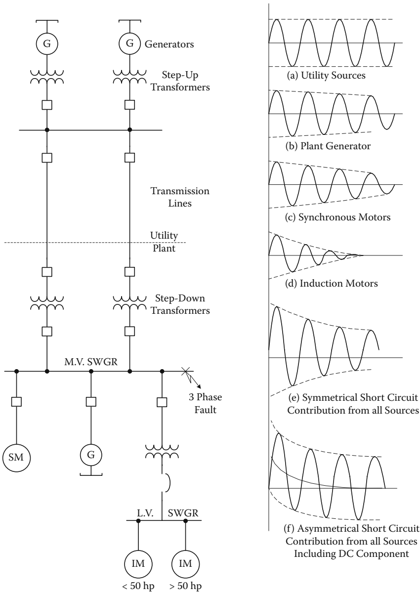
FIGURE 3.1 Fault contribution from different sources
