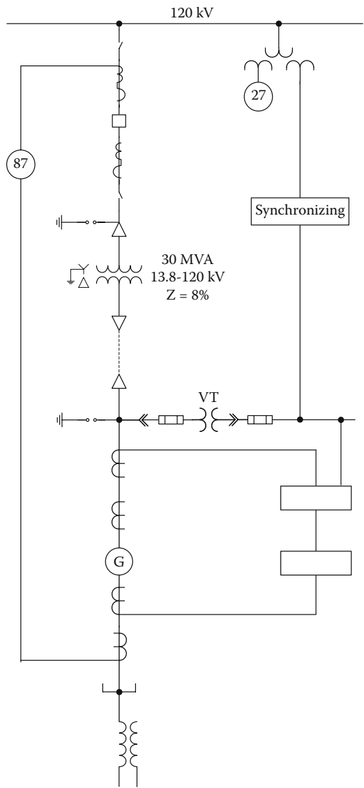
FIGURE 11.35 Protection scheme for a unit-connected generator
