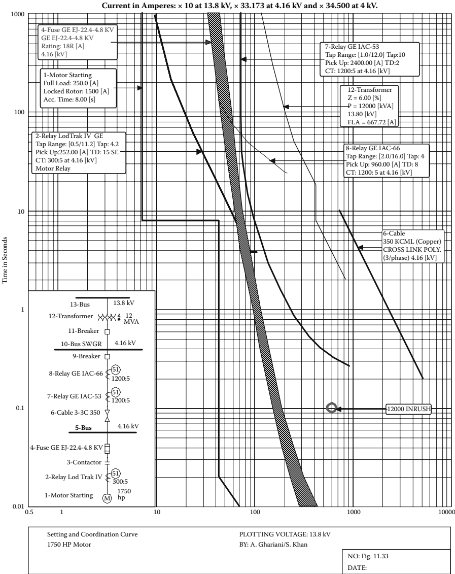
FIGURE 11.33 Setting and coordination curve for a 1750-hp motor
