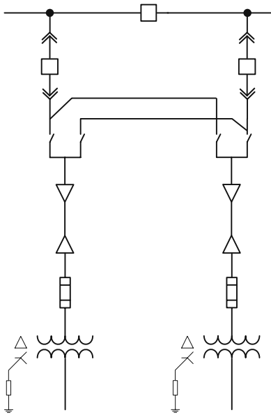
FIGURE 2.6 Primary selective
