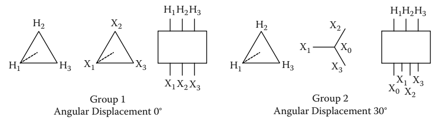
FIGURE 5.2 Angular displacement and terminal markings
