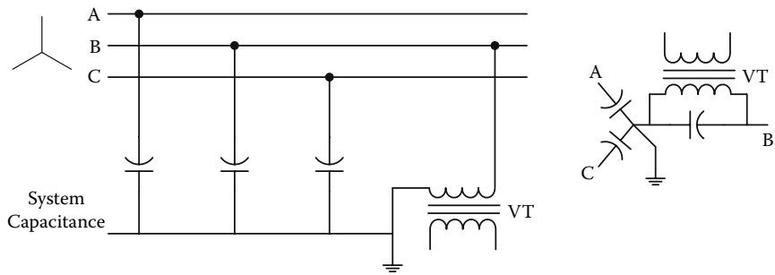
FIGURE 6.7 Ferro-resonance in a voltage transformer
