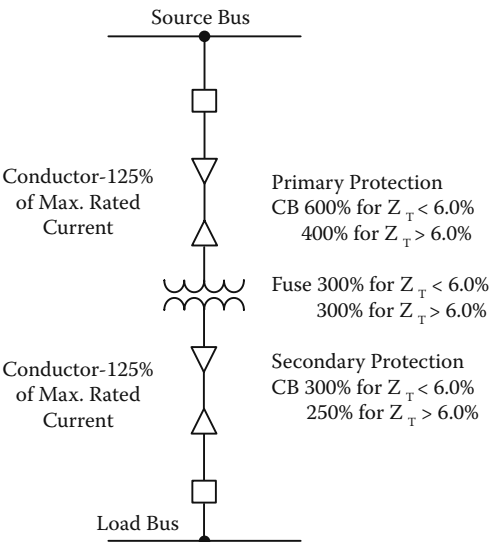
FIGURE 11.8 National Electrical Code rules for transformer protection
