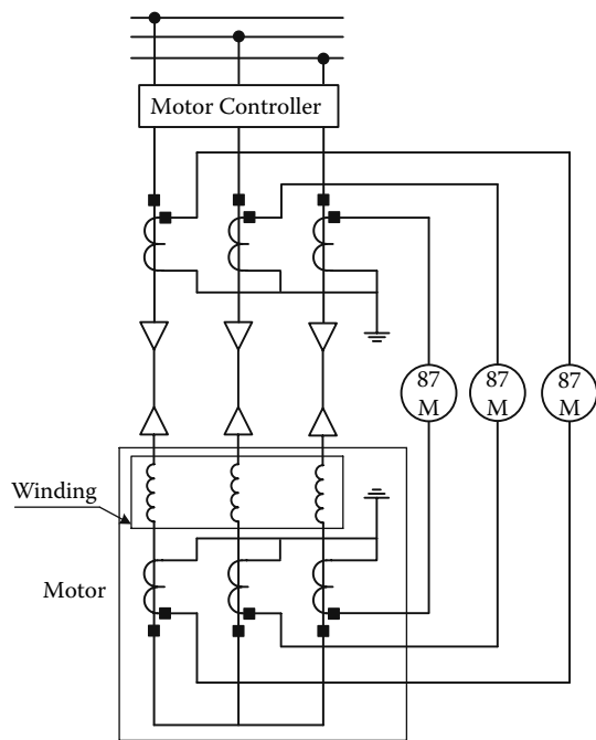
FIGURE 11.26 Overall differential-protection scheme
