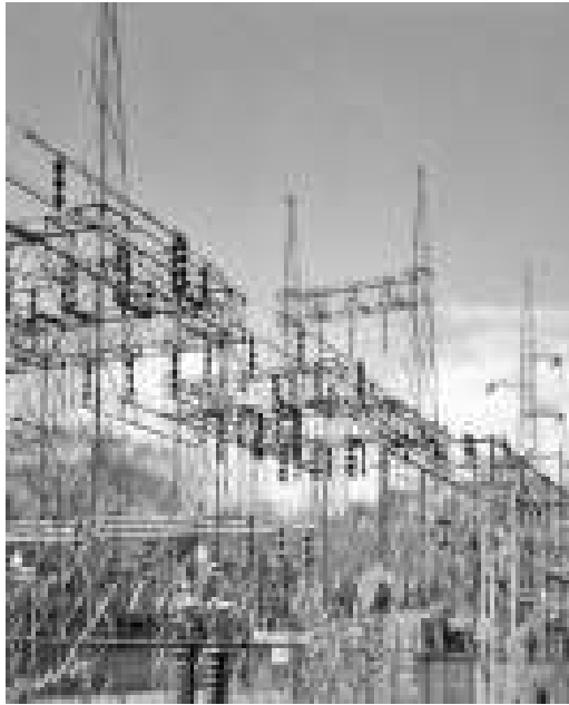
FIGURE 12.16 Switchyard protected by overhead shield wires
