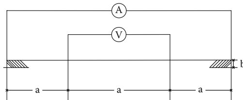
FIGURE 13.5 Measurement techniques
