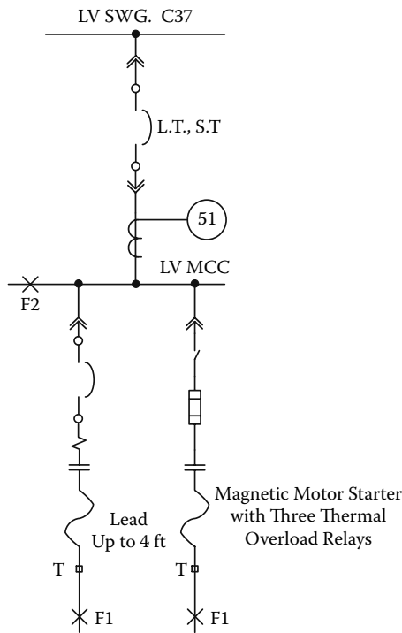
FIGURE 7.14 Low-voltage MCC
