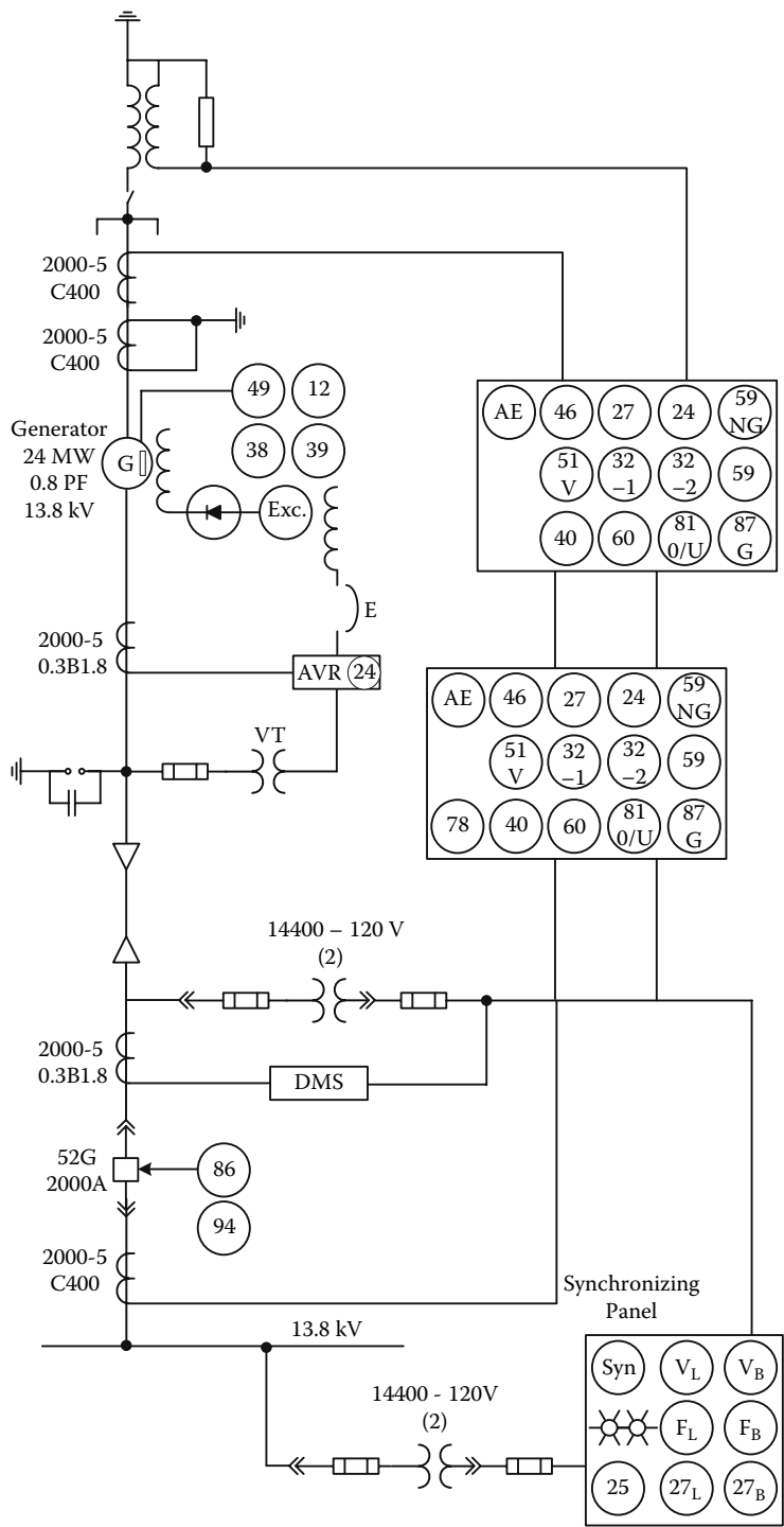
FIGURE 11.34 Protection scheme for a HR-grounded generator
