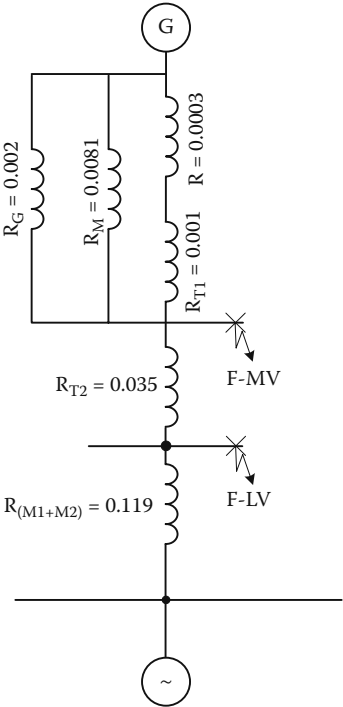
FIGURE 3.13 R diagram for CL/latch duty: MVCB and interrupting duty of LVCB
