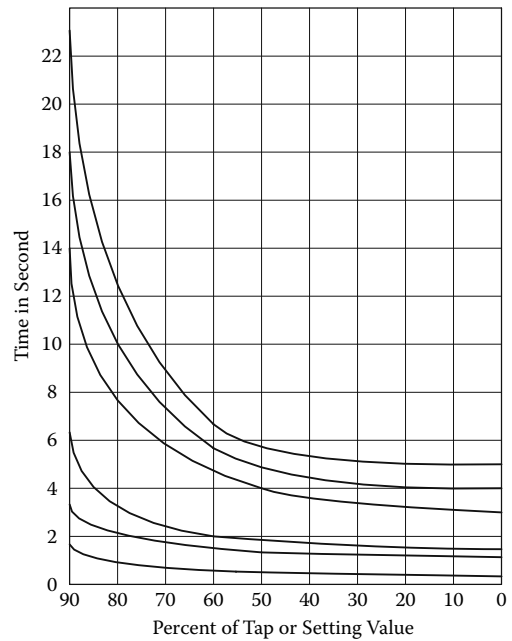
FIGURE 11.22 Inverse-time undervoltage
