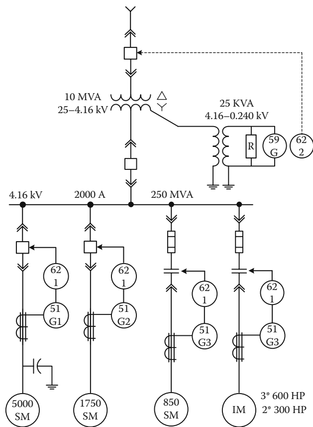
FIGURE 4.7 Single (one)-line diagram to design a HR grounding for a 4.16 kV system
