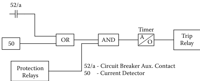
FIGURE 11.45 Logic diagram of a generator breaker-failure scheme
