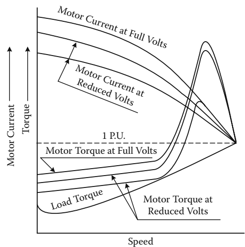
FIGURE 11.16 Motor speed: torque and current
