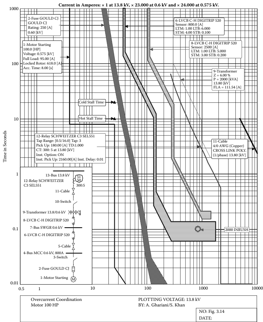
FIGURE 3.14 Overcurrent coordination
