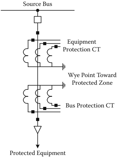
FIGURE 11.2 CT connections
