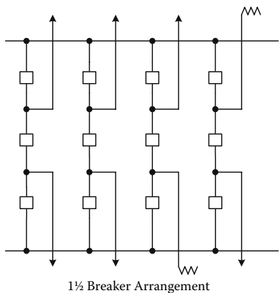
FIGURE 12.5 1½-breaker configuration
