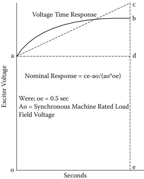
FIGURE 14.3 Excitation system nominal response
