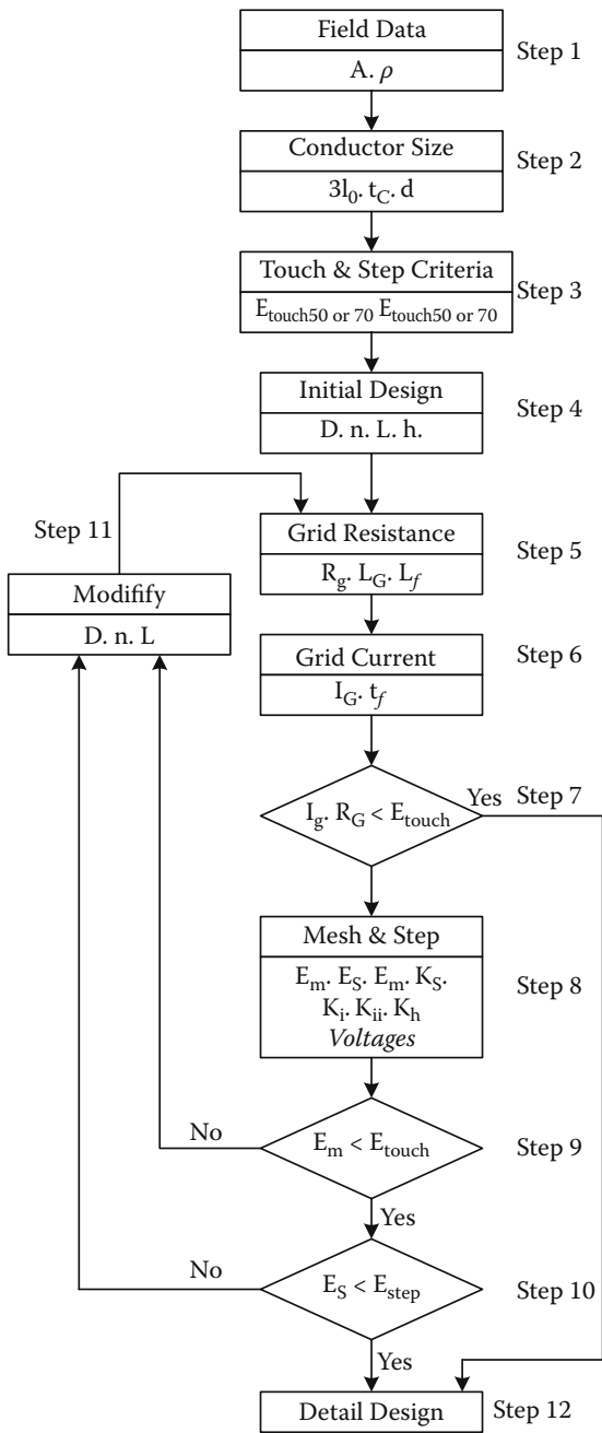
FIGURE 13.13 Design-procedure block diagram
