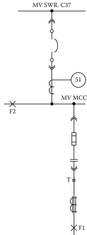
FIGURE 7.15 Medium-voltage MCC
