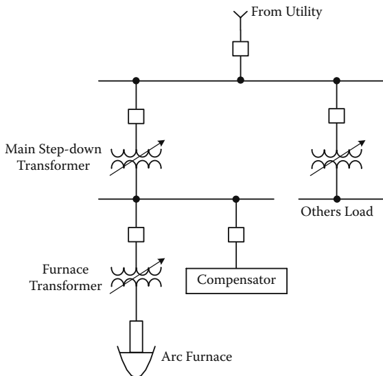
FIGURE 2.10 Power system for an arc furnace
