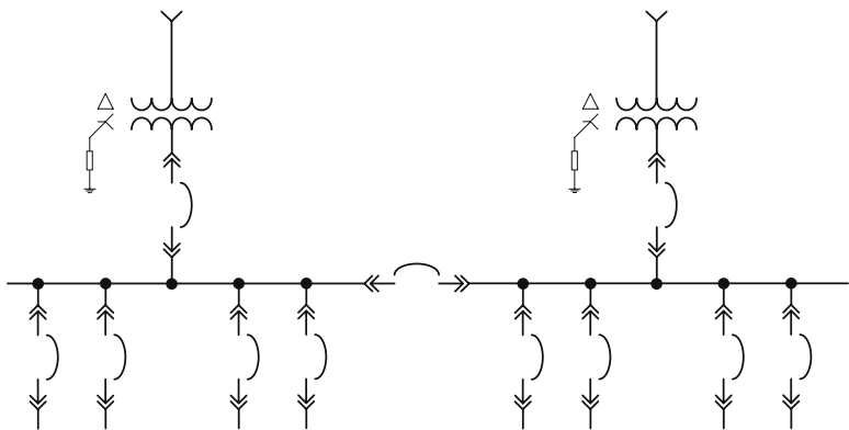
FIGURE 2.7 Secondary selective
