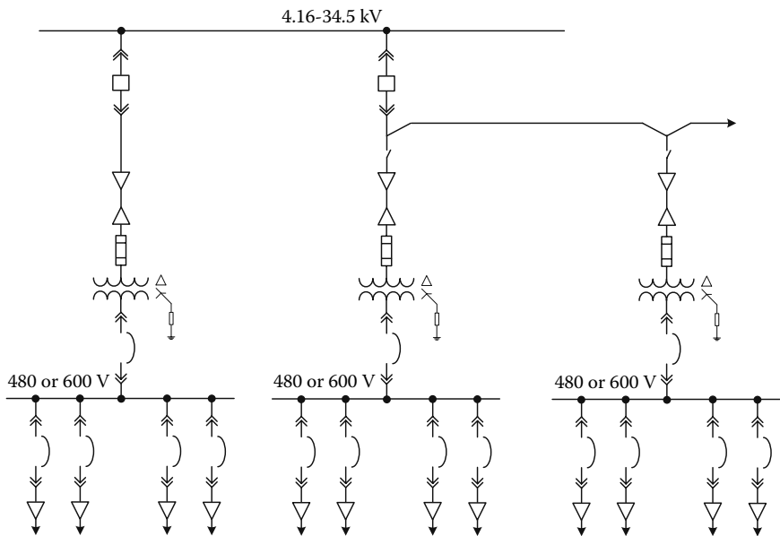
FIGURE 2.4 Simple radial
