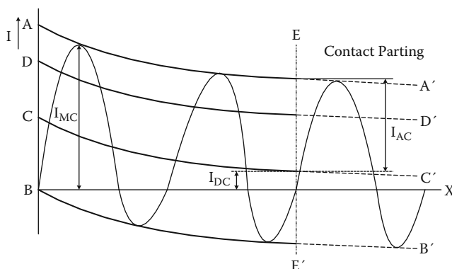
FIGURE 7.10 Short-circuit current
