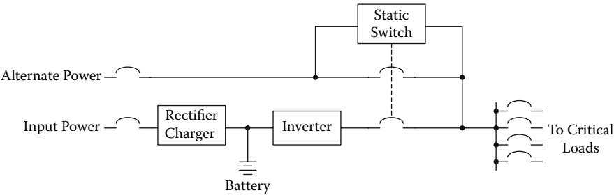
FIGURE 2.2 Nonredundant UPS
