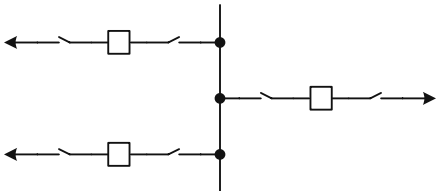
FIGURE 12.6 Basic single-bus configuration
