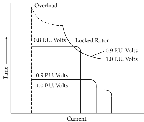
FIGURE 11.17 Motor time–current curve
