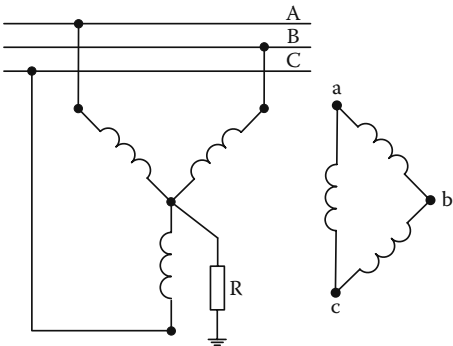
FIGURE 4.19 Wye-Delta grounding transformer for MV system
