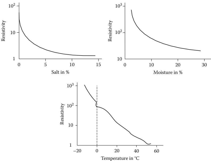
FIGURE 13.3 Earth-resistivity variations
