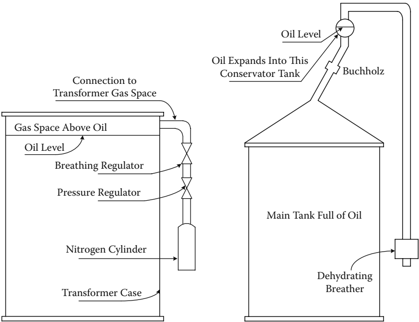
FIGURE 5.5 Oil-preservative system for power transformers
