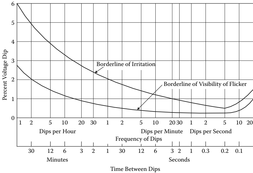
FIGURE 2.9 Range of observable and objectionable voltage flicker vs. time (From IEEE 141-1993, IEEE Recommended Practice for Electric Power Distribution for Industrial Plants (IEEE Red book), chap. 2. With permission.)
