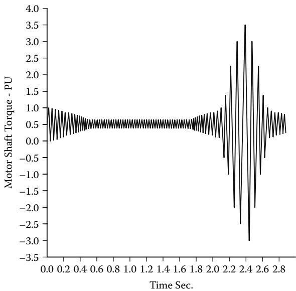
FIGURE 9.14 Torque pulsation
