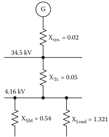
FIGURE 9.18 Impedance diagram
