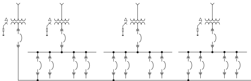
FIGURE 2.8 Sparing transformer
