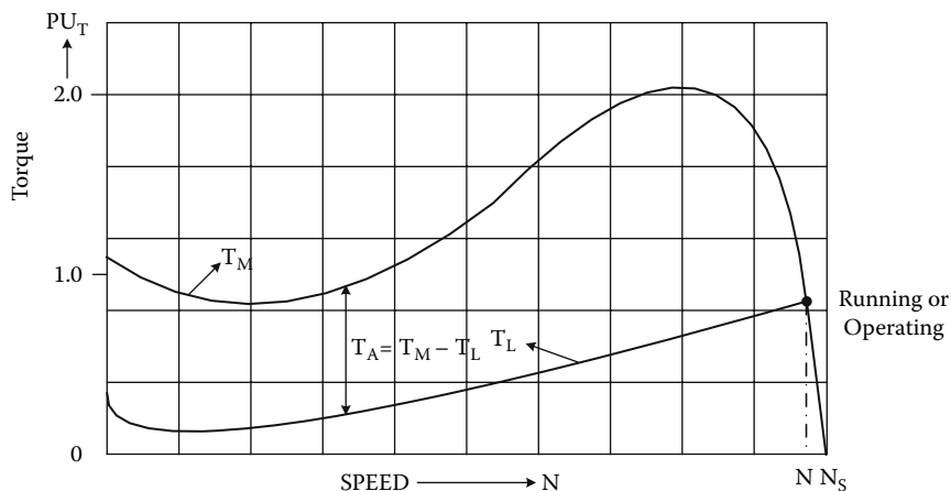
FIGURE 9.3 Speed–torque curve
