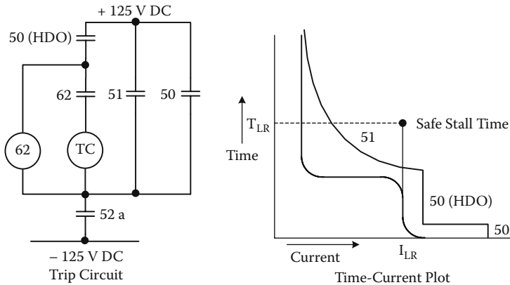
FIGURE 11.24 Application of device 50/51 for the protection of motor driving high-inertia load
