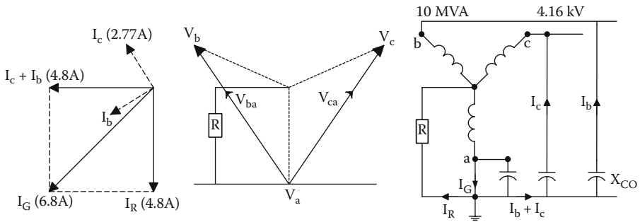
FIGURE 4.6 Ground fault on phase “a” (HR)
