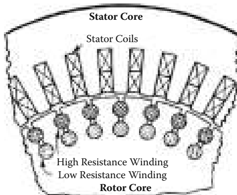
FIGURE 9.7 Double-cage rotor
