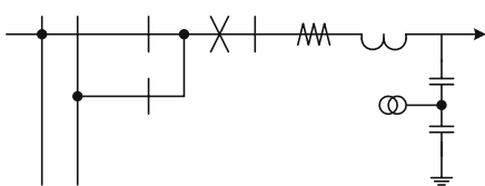
FIGURE 12.7 Double-bus arrangement
