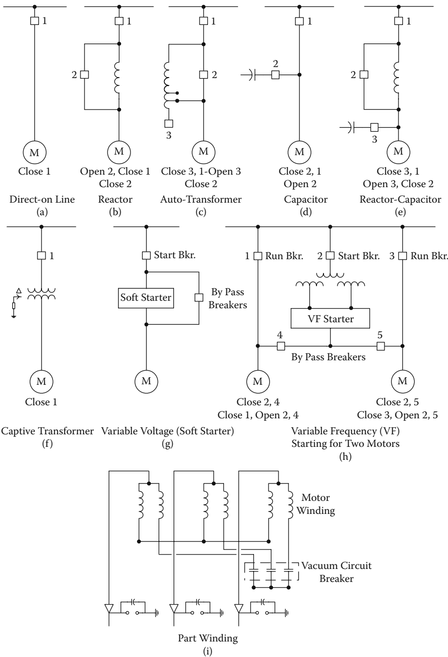
FIGURE 9.21 Motor-starting methods
