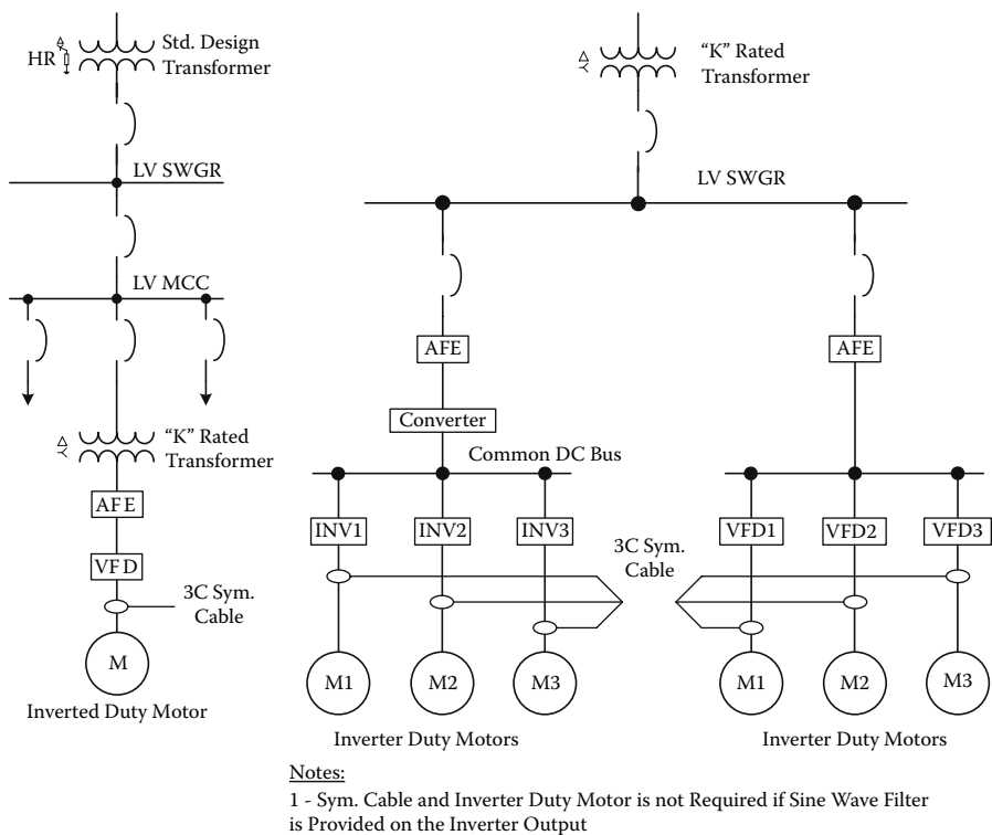
FIGURE 16.8 Suggested arrangements for power supply to low-voltage (<600 V) drives
