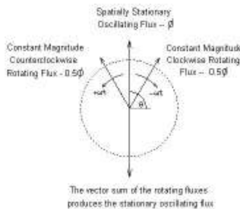
Counter-rotating field concept.
