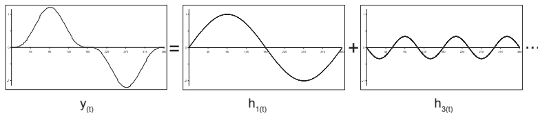
Fig. 30a Analysing a periodic signal into its component harmonics
