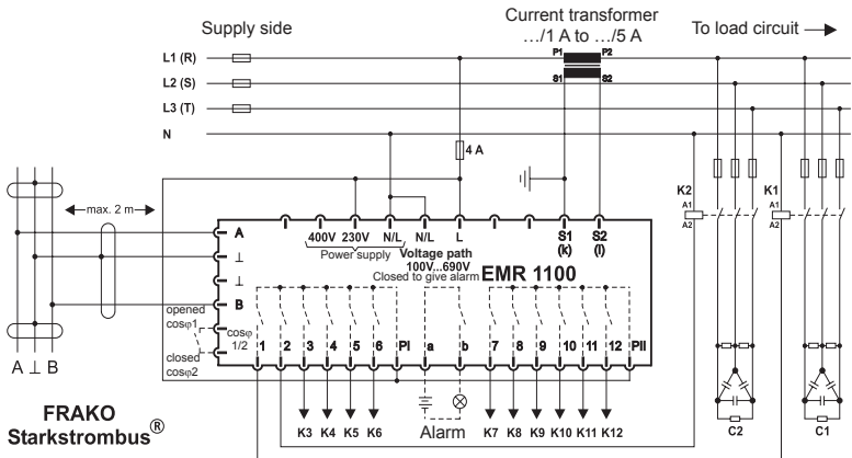
Fig. 22 Typical PFC system circuit
