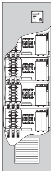
Fig. 21 Typical modular design of a PFC system
