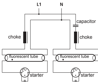
Fig. 14 Split-phase (lead-lag) circuit with the capacitor in series with the lamps, e.g. type LPMI (series capacitor) with 450 V rating
