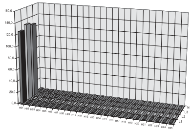
Fig. 46 Harmonics measured with filter
