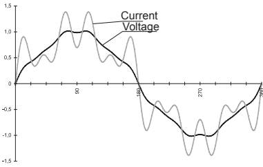
Fig. 30c Network current and voltage superposed with the following harmonics: 5% of the 5th harmonic, 4% of the 7th harmonic and 2.5% of the 11th harmonic
