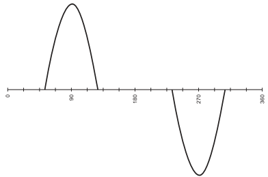
Fig. 32 Line current of a converter for induction motors
