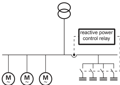
Fig. 29 Incorrect! The current transformer only registers the capacitor current: the capacitor is not switched in. The reactive power control relay gives the message I = 0 (no current in transformer circuit)!
