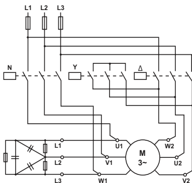
Fig. 20 Motor with individual power factor correction and star-delta contactor
