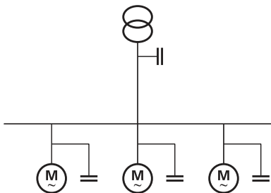
Fig. 8 Typical individual power factor correction
