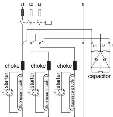
Fig. 15 Group correction for several discharge lamps distributed between the three phases (e.g. with type LKT power capacitor plus accessories)
