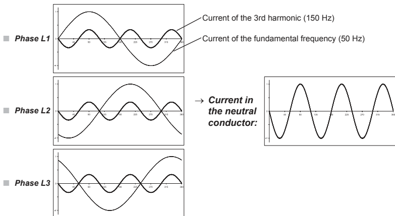
Fig. 30b Cumulative effect of the 3rd harmonic current in the neutral conductor
