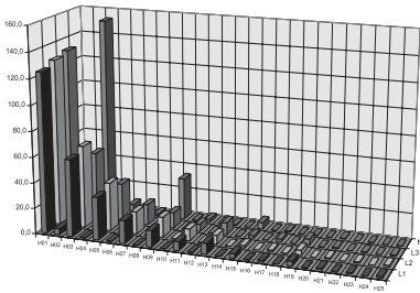
Fig. 45 Harmonics measured without filter
