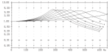
Fig. 35 Amplification of harmonic voltages as a function of the capacitor stages switched in FRAKO - Mains Analysis
