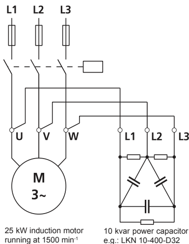
Fig. 17 Typical permanently installed power factor correction for a motor
