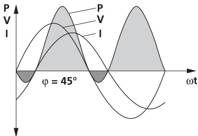
Fig. 2 Voltage, current and power with a resistive and an inductive load ( \varphi = 45^\circ )
