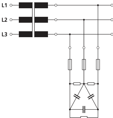
Fig. 16 Typical transformer with permanent power factor correction
