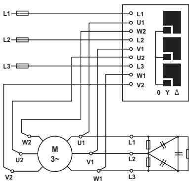
Fig. 19 Manually operated star-delta switch, special version for motors with individual power factor correction
