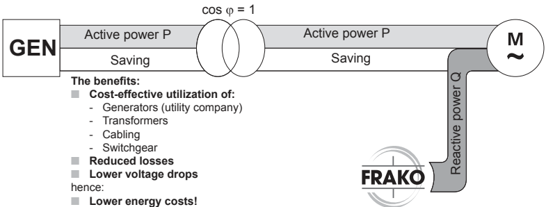
Fig. 7 Active and reactive power in the power distribution system: with PFC
