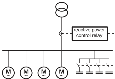
Fig. 10 Typical central PFC system
