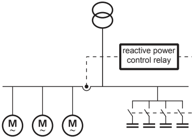
Fig. 28 Incorrect! The current transformer only registers the load current: the capacitor bank is switched in but not out again. The reactive power control relay gives the message "C = 0" (no capacitor current can be measured)
