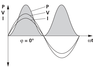
Fig. 1 Voltage, current and power curve for a purely resistive load ( \varphi = 0^\circ )
