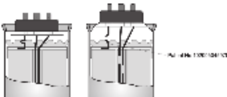
Fig. 23 Sectional view through a FRAKO power capacitor showing the mechanical fuses under excess internal pressure
