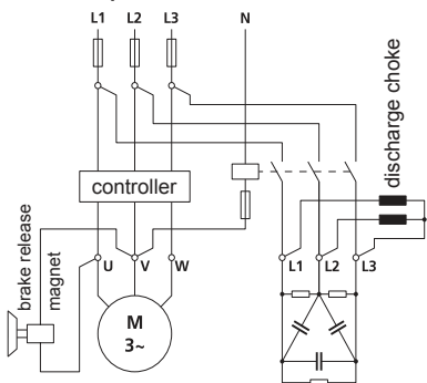
Fig. 18 Elevator motor with own capacitor switching contactor and rapid discharge facility
