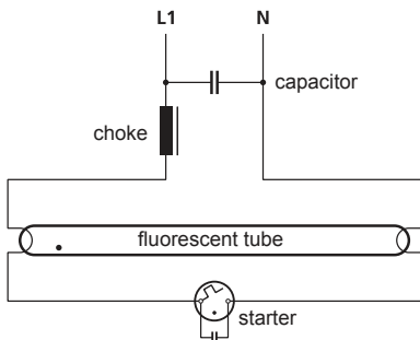
Fig. 12 Individual correction with the capacitor in parallel with the lamp, e.g. type LPM (shunt capacitor) with 230 V rating
