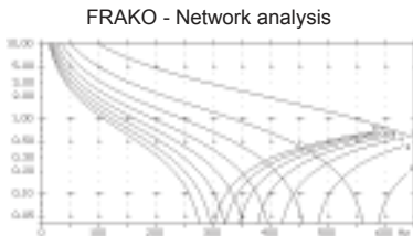
Fig. 37 Impedance factor \alpha^* as a function of the switched-in capacitor stages
