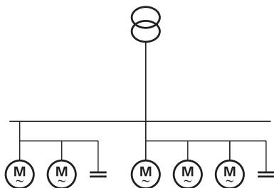
Fig. 9 Typical group power factor correction
