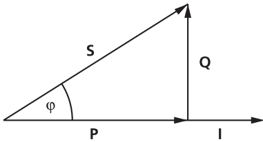
Fig. 4 Power triangle
