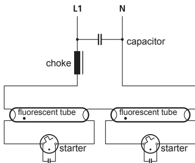
Fig. 13 Two lamps connected in tandem with the capacitor in parallel with them, e.g. type LPM (shunt capacitor) with 230 V rating
