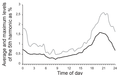
Fig. 33 Average and maximum levels of the 5th harmonic as %
