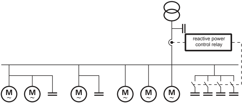
Fig. 11 Typical hybrid PFC system
