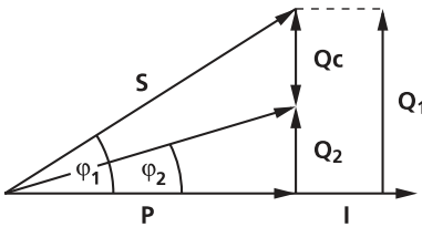
Fig. 5 Power triangle showing the effect of correction
