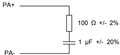
Fig. 5: Bus termination PROFIBUS MBP (PA)
