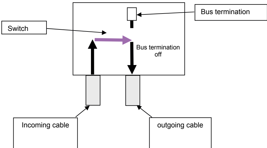
Fig. 6: termination on / incoming and outgoing cable not connected
