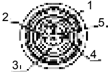
Fig. 10: 5 pin M-12 male plug for RS 485
