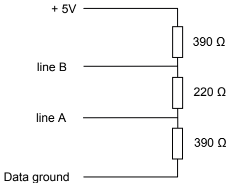
Fig. 4: Bus termination PROFIBUS RS 485
