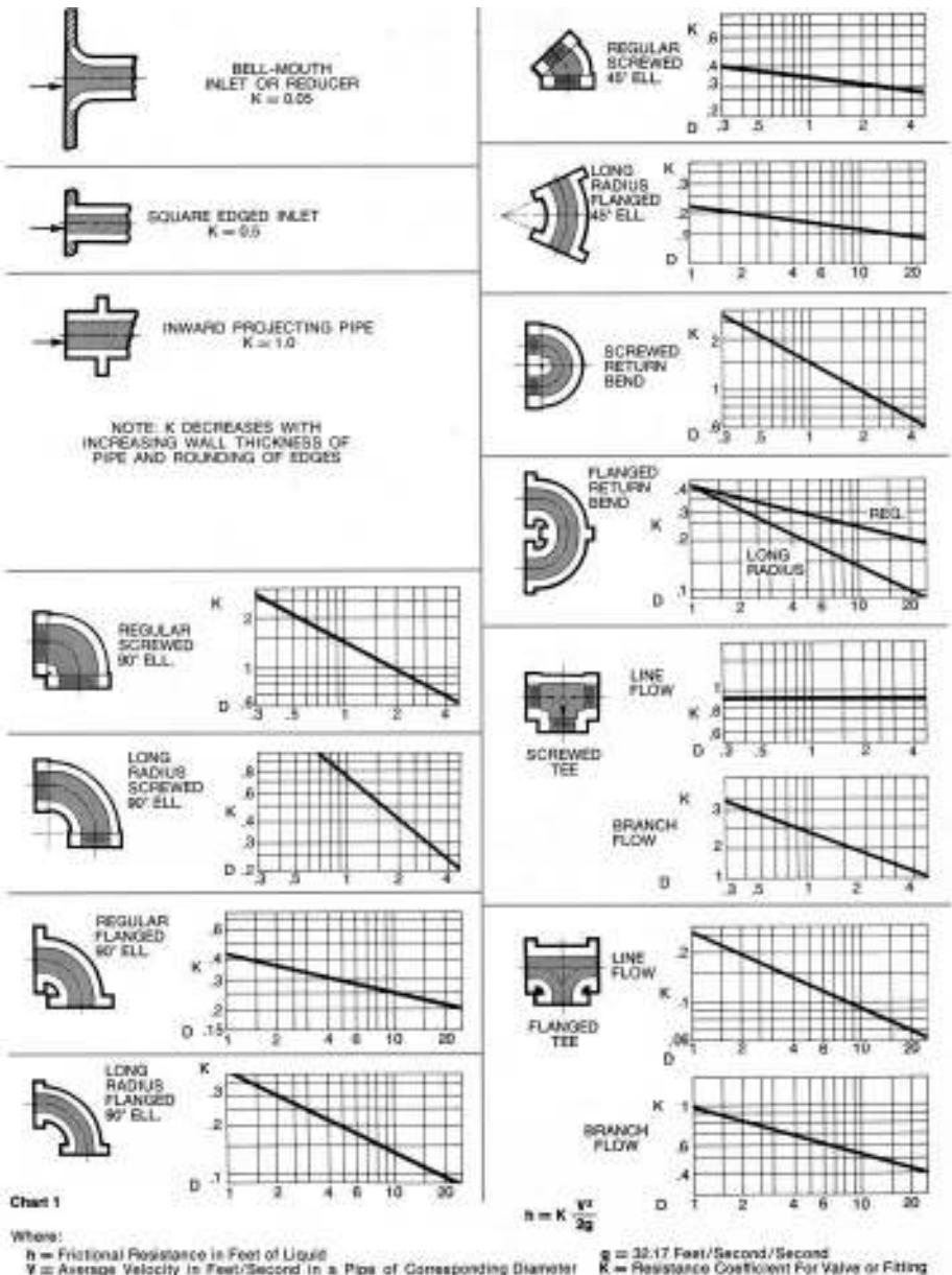
Figure 2.2 Resistance coefficients (K) for valves and fittings. (From Engineering Data Book , 2nd edition. Courtesy of Hydraulic Institute, Parsippany, NJ; www.pumps.org and www.pumplearning.org .)
