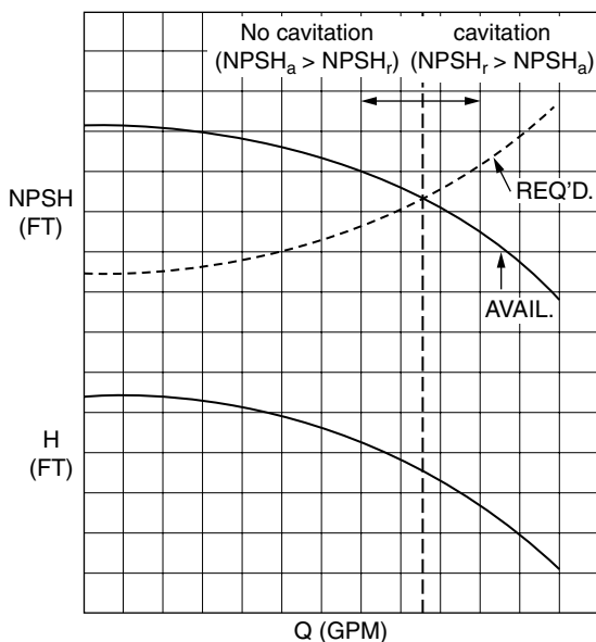
Figure 2.12 Variation of NPSH_a and NPSH_r with flow through the system.
