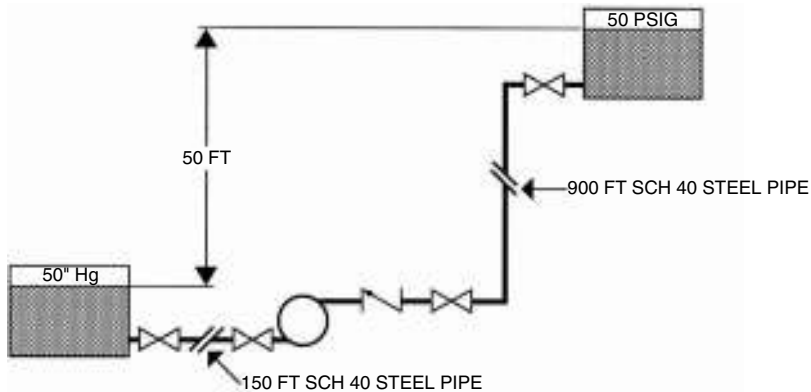
Figure 2.5 System for example problem illustrating selection of line sizes, pump TH, and pump size (Example 2.1); and NPSH a calculation (Example 2.5).
