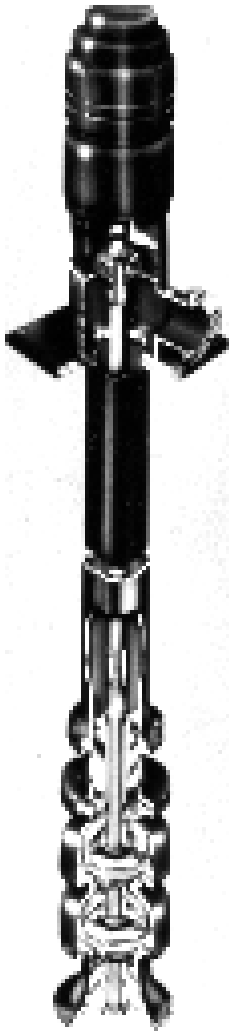
Figure 4.34 Vertical turbine pump. (Courtesy of Johnston Pump Company, Brookshire, TX.)
