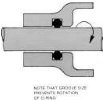
Figure 5.6 Rotary seal. (Courtesy of Parker Hannifin Corporation, Seal Group.)
