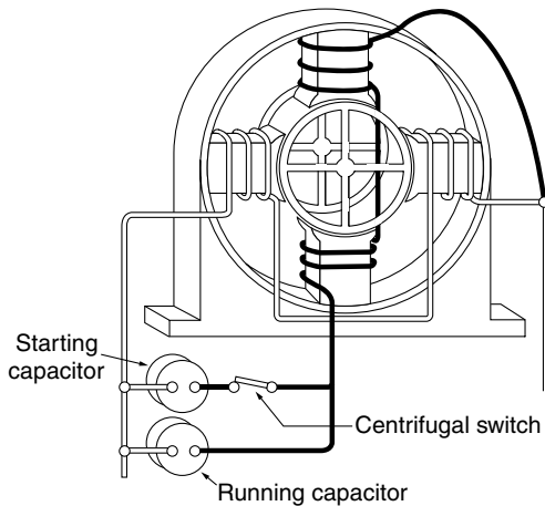
Figure 4.53 Two valve capacitor motors are used in large horsepower single phase motors. (Courtesy of Edward Cowern, P.E., North Haven, CT.)
