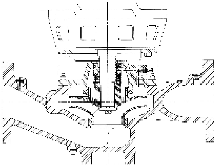
Figure 4.14 Sectional view of inline pump. (Courtesy of Crane Pumps & Systems, Inc., Piqua, OH.)
