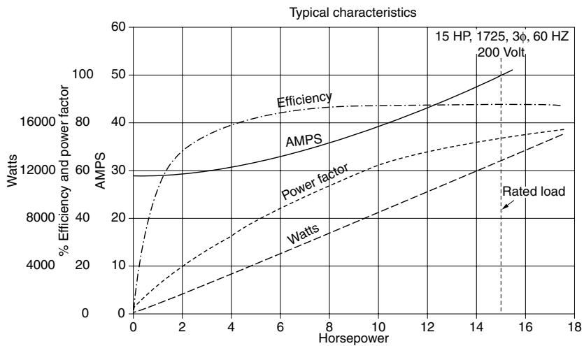
Figure 4.54 Typical motor performance data. (Courtesy of Edward Cowern, P.E., North Haven, CT.)
