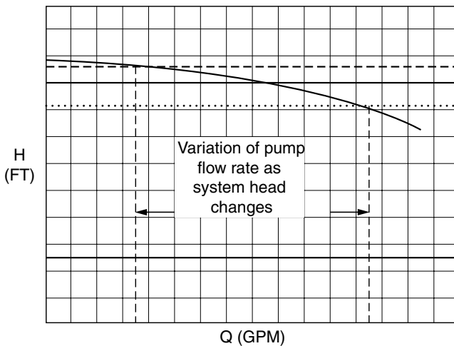
Figure 2.21 The combination of a flat system head curve (no friction or very little friction) with a relatively flat H–Q pump curve produces wide flow swings with relatively small system head variation.
