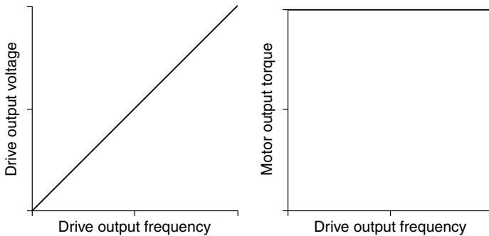
Figure 6.10 Drive output voltage–frequency pattern for constant motor torque. (Courtesy of Danfoss Graham, Milwaukee, WI.)
