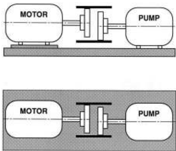
Figure 8.2 Rough parallel alignment check using straight edge.
