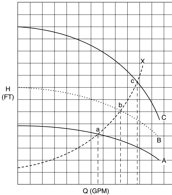
Figure 2.36 Combined pump curve for two nonidentical pumps in series, and system head curve.
