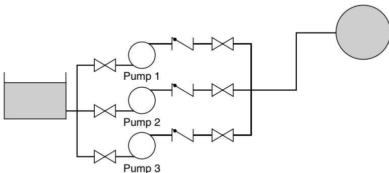
Figure 2.28 Parallel operation.
