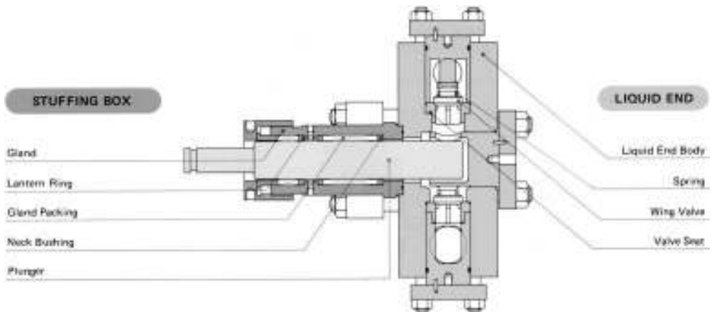
Figure 1.24 Plunger pump liquid end and stuffing box. (Courtesy of NIKKISO Pumps America, Inc., Plumsteadville, PA.)
