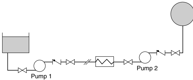
Figure 2.33 Series operation.
