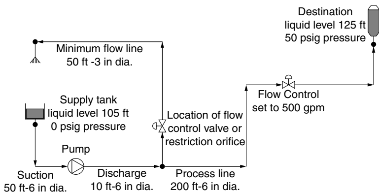
Figure 8.7 Simple piping system with a minimum flow recirculation line. (Courtesy of Engineered Software, www.eng-software.com , Lacey, WA.)
