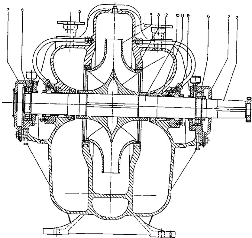
FIGURE 11 Between bearings centrifugal cargo pump (Flowserve Corporation)
