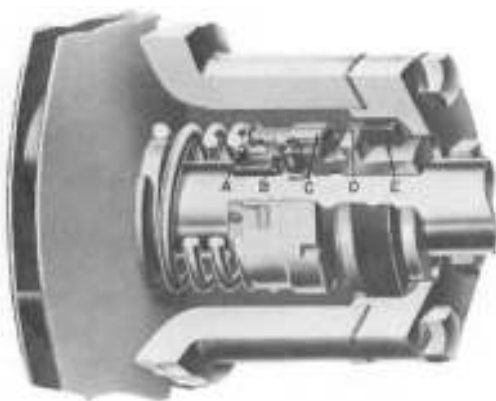
FIGURE 25 A full-convolution bellows seal (John Crane Inc.)
