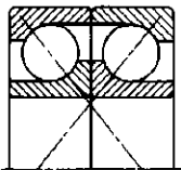
FACE-TO-FACE
