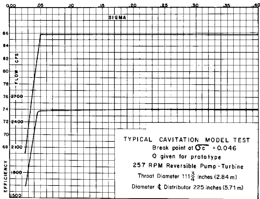
FIGURE 5 Typical cavitation model test ( 1 \text{ ft}^3/\text{s} = 0.0283 \text{ m}^3/\text{s} ) (Voith Siemens Hydro)
