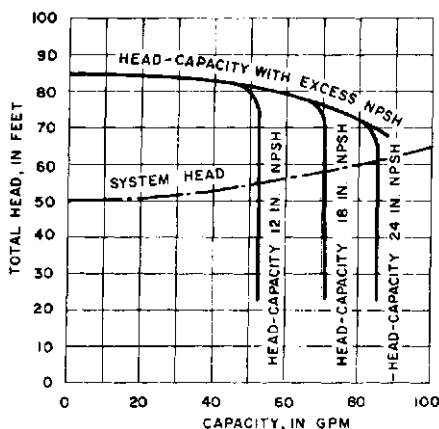
FIGURE 36 Characteristic of a condensate pump operating on a submergence-controlled system
