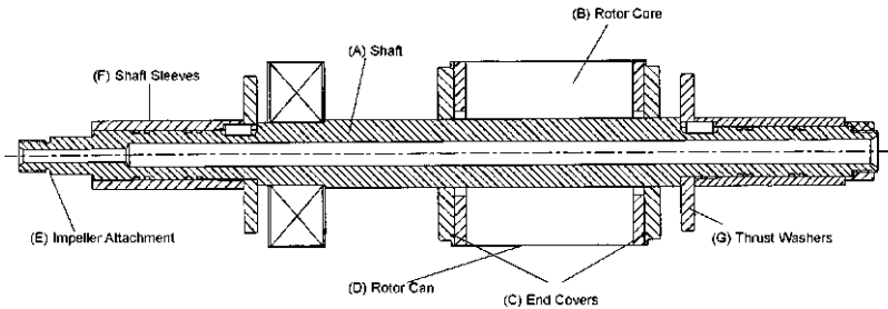
FIGURE 3 Rotor assembly
