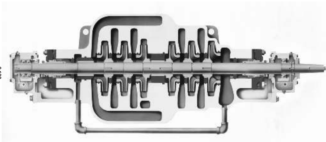
FIGURE 4 Axially split multistage pump API 610 Type BB3 (Flowserve Corporation)
