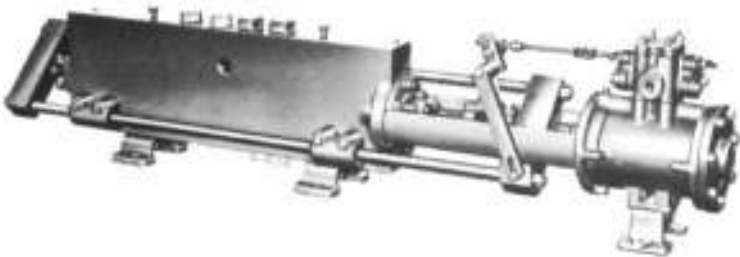
FIGURE 12 Simplex-type plunger pump (Flowserve Corporation)
