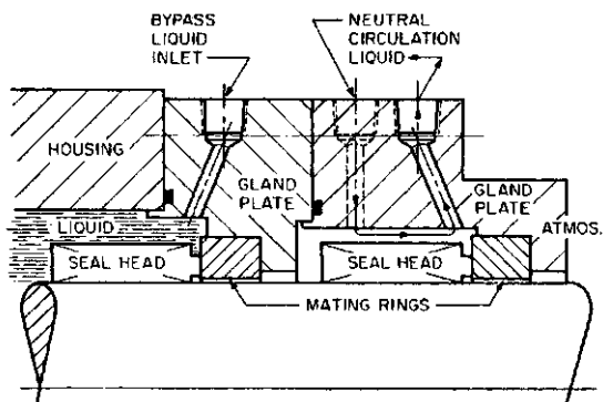
FIGURE 16 Tandem seals
