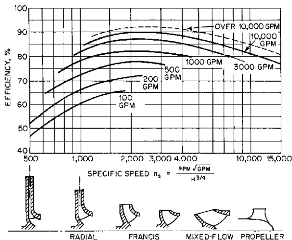
FIGURE 6 Pump efficiency versus specific speed and size ( \text{gpm} \times 0.06309 = \text{l/s} ) (Flowserve Corporation) (\Omega_s = n_s/2733)
