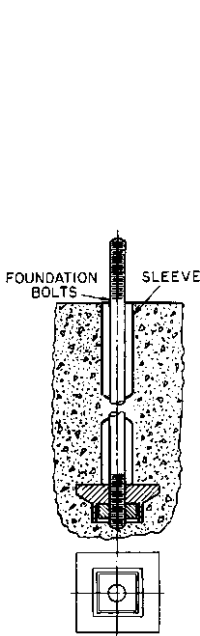
FIGURE 1 Foundation bolt
