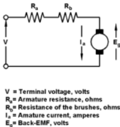
FIGURE 11 The equivalent circuit of a dc motor with a permanent magnet stator
