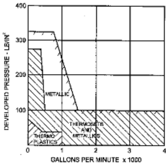
FIGURE 2 Developed pressure versus flow for composite pumps (lb/in 2 × 0.0689 = bar; gpm × 0.227 = m 3 /h)
