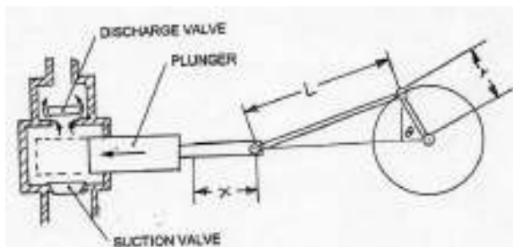
FIGURE 5 Slider-crank mechanism
