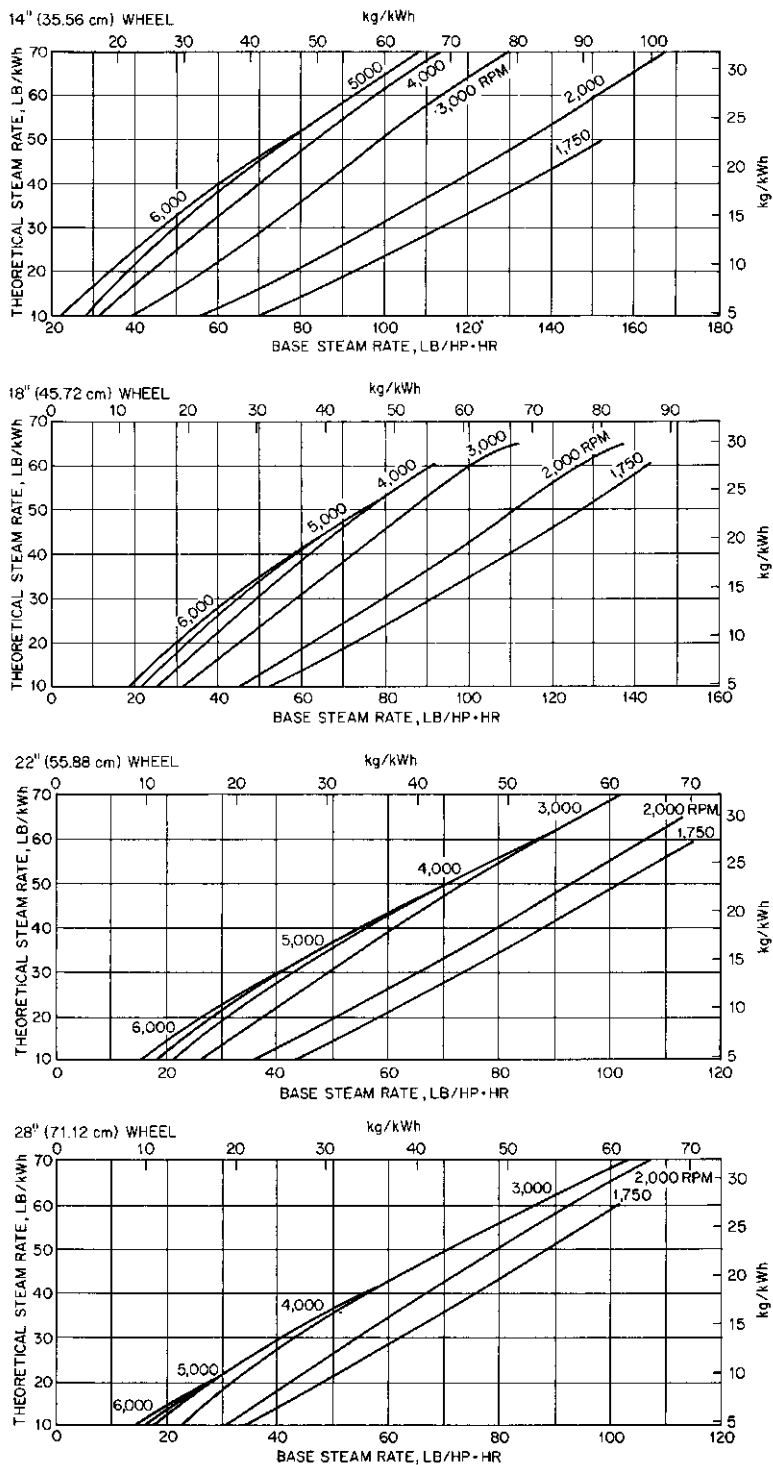
FIGURE 7 Base steam rates (Elliott)
