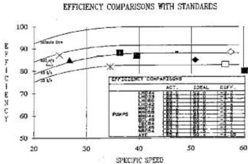
FIGURE 6 Pump efficiency as a function of specific speed n_q , based on m 3 /s, m, and rpm (from Addie and Helmly, 1989). [Note: for specific speed N_s , based on gpm, ft, and rpm, multiply n_q by 51.65; for universal specific speed \Omega_s , divide n_q by 52.92.]
