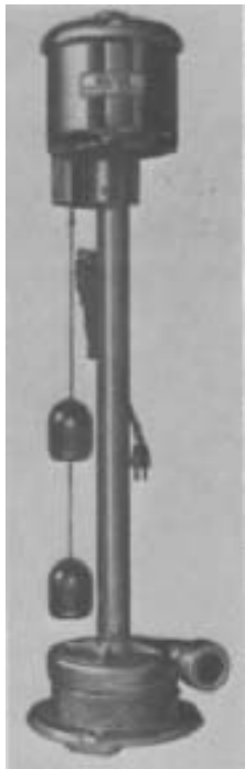
FIGURE 122 A cellar-drainer sump pump (Sta-Rite Products)
