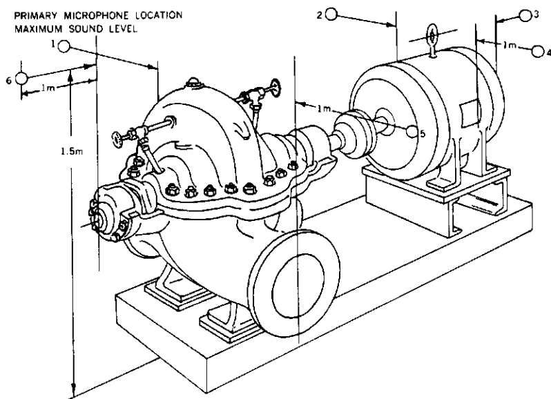
FIGURE 8 Placement of microphones on a horizontally split centrifugal pump (Hydraulic Institute ANSI/HI 2000 Edition Pump Standards, Reference 3)
