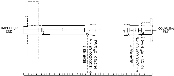
FIGURE 2 Rotor cross section of single-stage overhung pump with normal coupling weight. Rotor weight = 110.4 lb (50 kg); rotor length = 30.3 in (77.0 cm); number of stations = 22; number of bearings = 2
