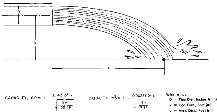
FIGURE 18 Approximating flow from a horizontal pipe
