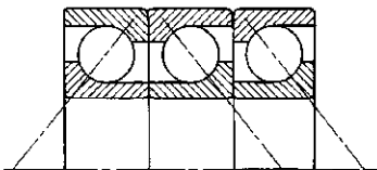
BACK-TO-BACK / TANDEM
