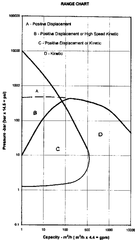
FIGURE 1 General pump overview
