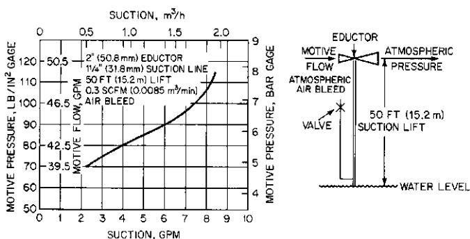
FIGURE 22 Suction capacity of eductor-air-lift combination ( \text{gpm} \times 0.227 = \text{m}^3/\text{h} )
