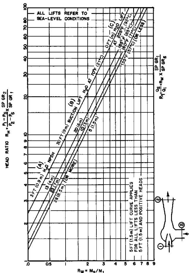
FIGURE 3 Estimating operating ratios for liquid jet ejectors. An ejector can be designed for only one head point (Schutte and Koerting)
