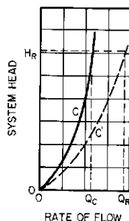
FIGURE 8 Bypass orifice system requirements
