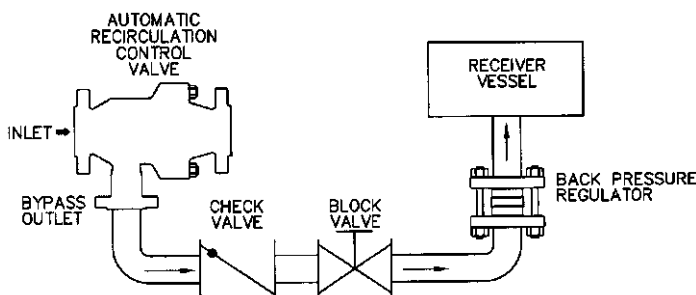
FIGURE 13 Backpressure regulator installation
