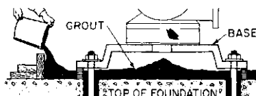
FIGURE 8 Application of grouting. Grout is added until the entire space under the base is filled. Holes in the base (arrow) allow air to escape and permit working of the grout to release air pockets.
