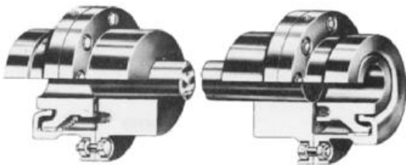
FIGURE 20 Section of floating shaft and couplings (Kop-Flex)
