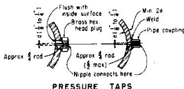
FIGURE 27 Head measurement. In SI units, h_d = [(0.102 P_d / W) + Z_d + (V_d^2 / 2g)] ; h_s = [(0.102 P_s / W) + Z_s + (V_s^2 / 2g)] . (ft \times 0.3048 = m; psi \times 6.894 = kPa; pcf \times .016 = kg/liter)
