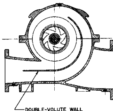
FIGURE 7 Transverse view of a double-volute casing pump.
