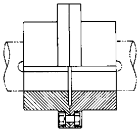
FIGURE 1 Flanged rigid coupling (Kop-Flex)
