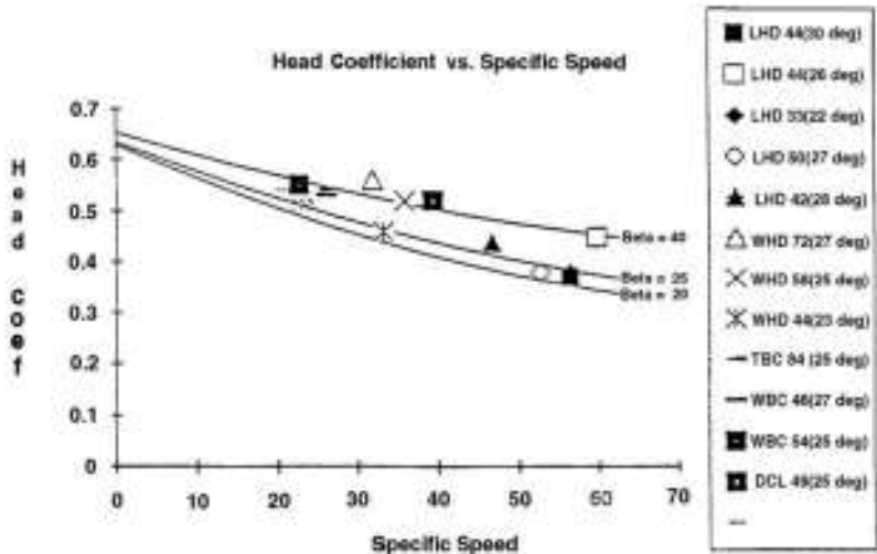
FIGURE 5 Head coefficient versus specific speed n_q , based on m 3 /s, m, and rpm (from Addie and Helmly, 1989). [Note: for specific speed N_s , based on gpm, ft, and rpm, multiply n_q by 51.65; for universal specific speed \Omega_s , divide n_q by 52.92.]
