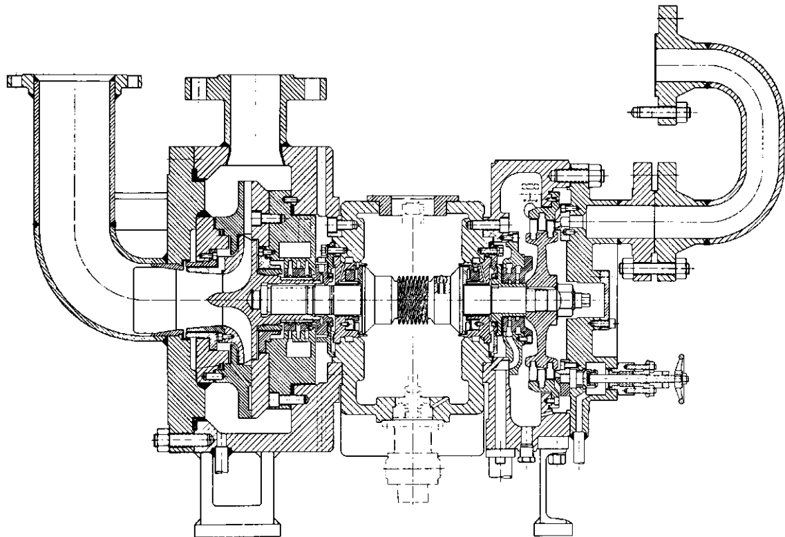
FIGURE 12 High-speed centrifugal pump and single-stage steam turbine mounted on a common shaft. Package is designed for boiler feed in marine, industrial, and process steam plants (Flowserve Corporation).
