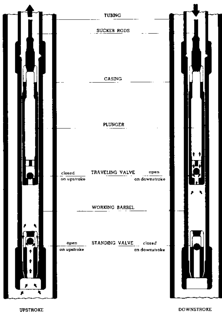
FIGURE 2 Operation of a tubing pump
