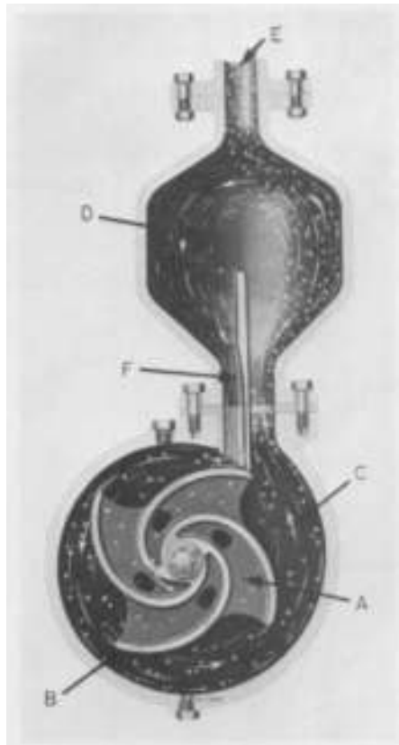
FIGURE 10 Self-priming pump with recirculation at discharge (Flowserve Corporation)
