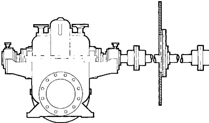
FIGURE 13A Horizontal centrifugal cargo pump with jackshaft (Flowserve Corporation)
