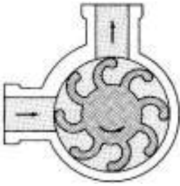
FIGURE 3 Flexible vane pump
