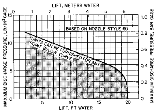
FIGURE 21 Air pumping liquid (Schutte and Koerting)
