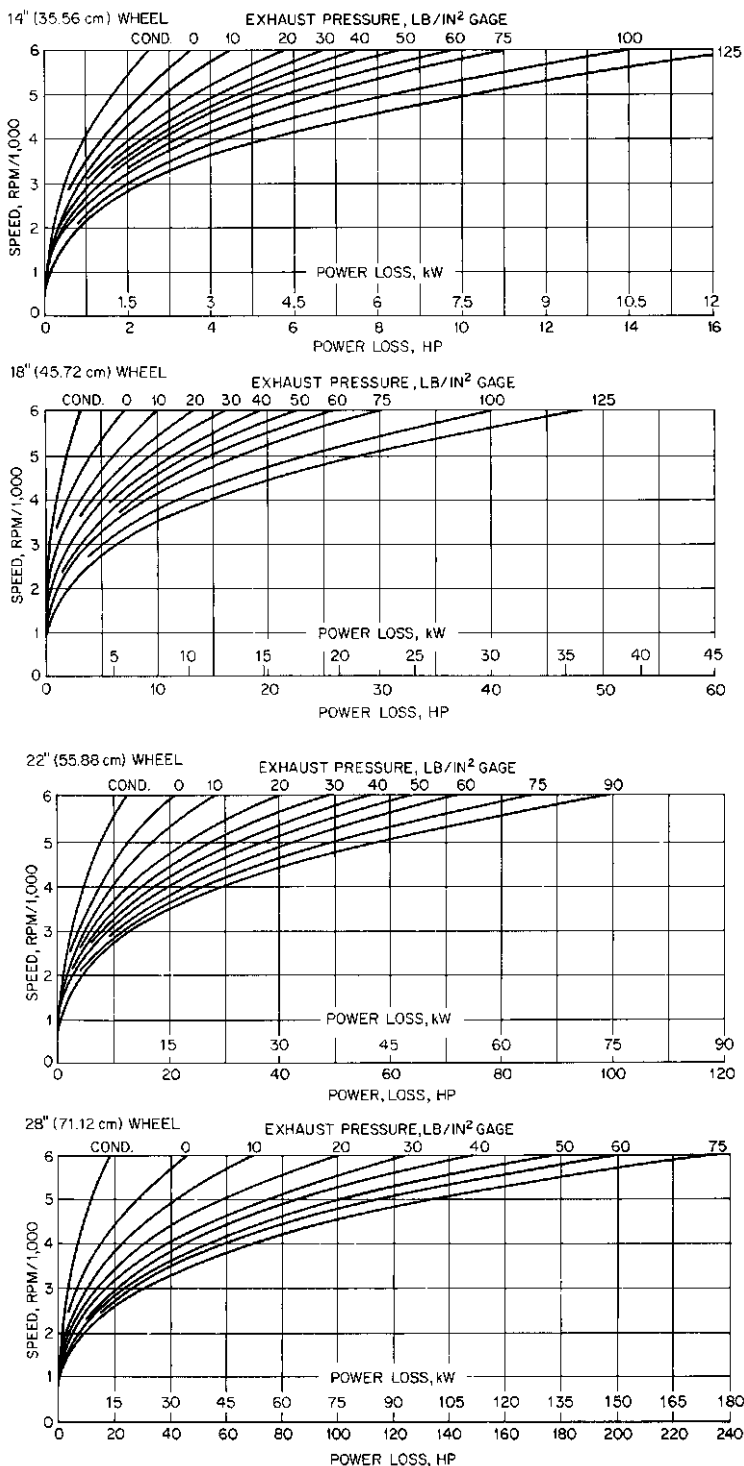
FIGURE 8 Power loss ( \text{lb/in}^2 \times 6.895 = \text{kPa} ) (Elliott)
