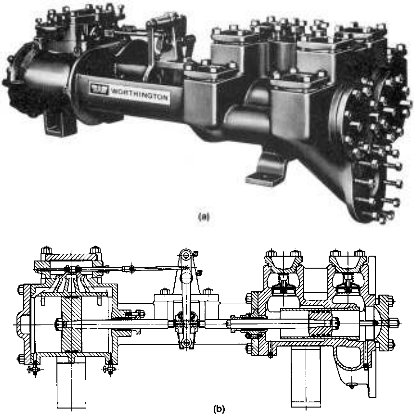
FIGURE 13A and B Side-pot piston pump (Flowserve Corporation)
