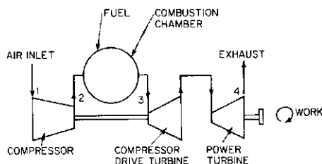
FIGURE 3 Components of a split-shaft gas turbine
