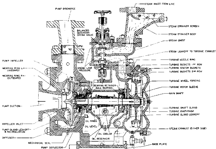
FIGURE 4 Close-coupled single-stage centrifugal main feed pump (Coffin Turbopump)
