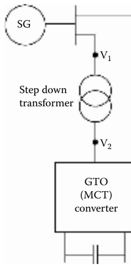
FIGURE 6.50 Advanced static voltage controller (SVC) = STATCOM.
