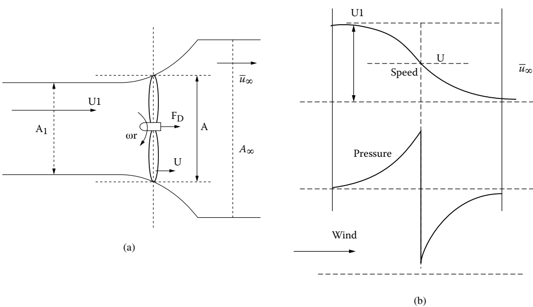
FIGURE 3.53 (a) Basic wind turbine speed and (b) pressure variation.
