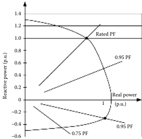
FIGURE 7.2 Reactive power capability curve.
