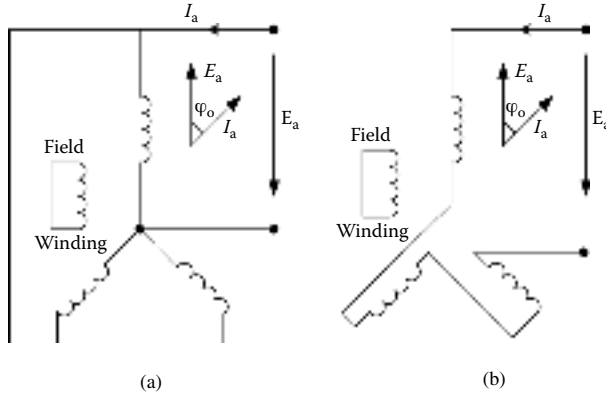
FIGURE 8.20 Single-phase supply tests to determine Z_o .
