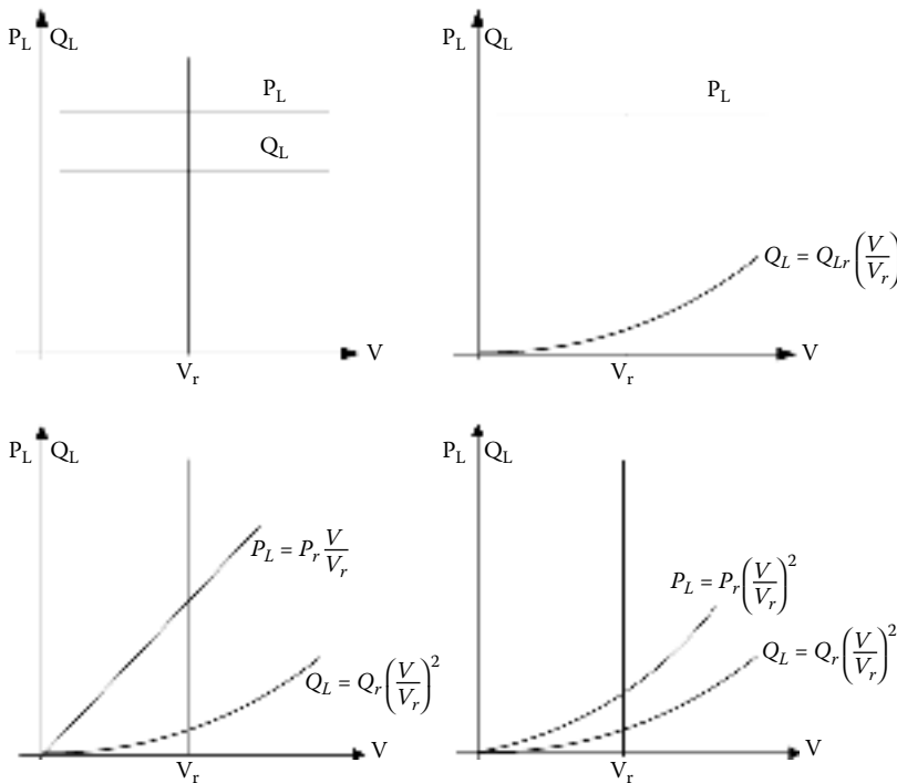
FIGURE 6.19 Typical P_L , Q_L load powers vs. voltage.
