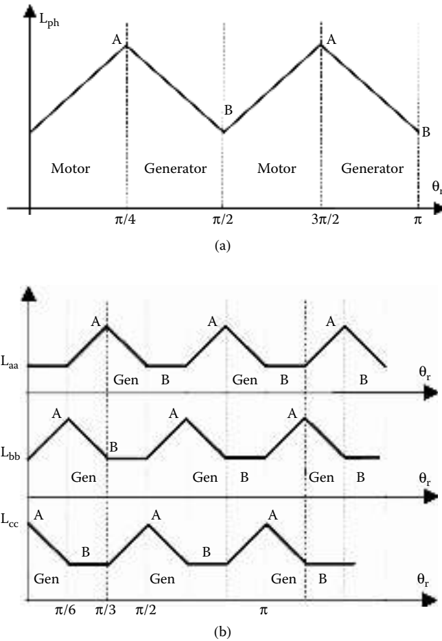
FIGURE 2.21 Phase inductance vs. rotor position: (a) the single-phase 4/4 switched reluctance generator (SRG) and (b) the three-phase 6/4 SRG.
