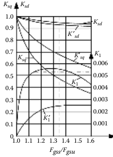
FIGURE 7.26 Saturation coefficients to account for cross-coupling magnetic saturation. (Redrawn from V.V. Dombrowski, A.G. Eremeev, N.P. Ivanov, P.M. Ipatov, M.I. Kaplan, and G.B. Pinski, Design of Hydrogenerators , vols. I and II, Energy Publishers, Moscow, 1965 [in Russian].)
