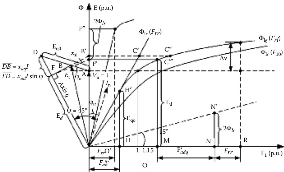
FIGURE 7.25 The partial magnetization curves method.
