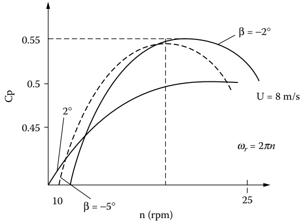
FIGURE 3.55 Typical C_p - n(\lambda) - \beta curves.
