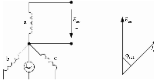
FIGURE 8.21 Sustained two line-to-neutral short-circuit.
