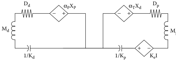
FIGURE 3.31 Free-piston Stirling engine dynamics model.
