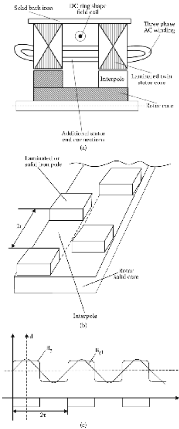
FIGURE 2.14 The homopolar synchronous generator: (a) and (b) the geometry and (c) airgap excitation field distribution.
