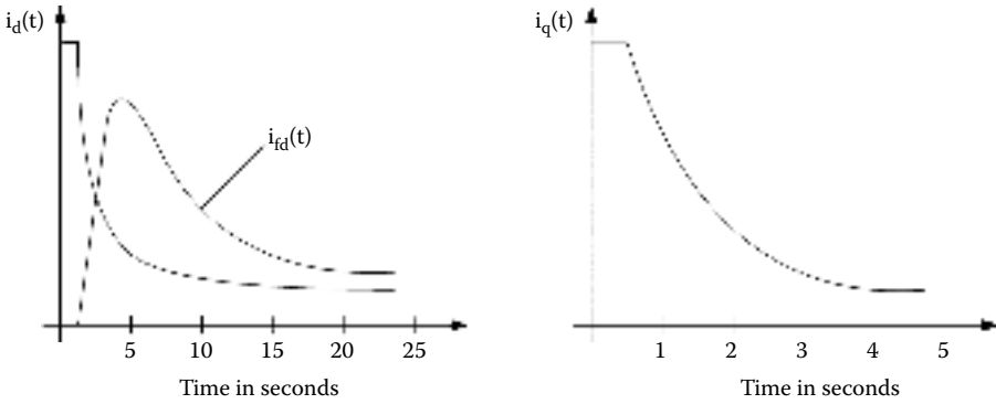
FIGURE 8.31 Flux decay transients at standstill.
