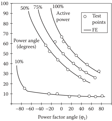
FIGURE 5.25 Power angle \delta_v vs. power factor angle \phi_1 of a 150 MVA, 13.8 kV, two-pole synchronous generator.
