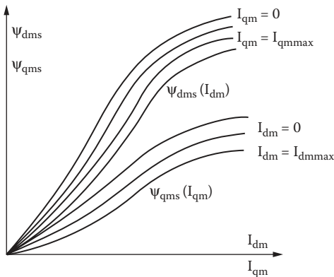
FIGURE 5.10 Family of magnetization curves.
