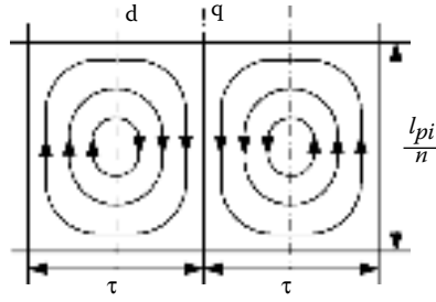
FIGURE 7.29 Solid iron rotor eddy currents trajectory in axis d .
