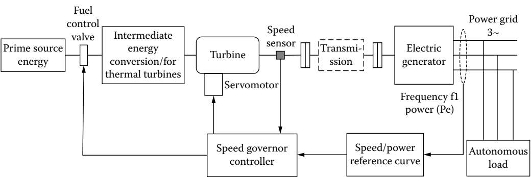
FIGURE 3.1 Basic prime-mover generator system.
