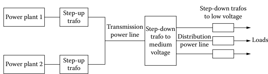
FIGURE 1.4 Single transmission in a multiple power plant — standard power grid.
