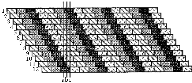
FIGURE 3.18 Twelve-cylinder engine timing.
