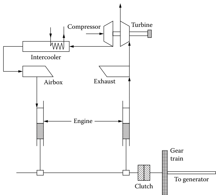
FIGURE 3.21 Diesel engine with turbocharger.
