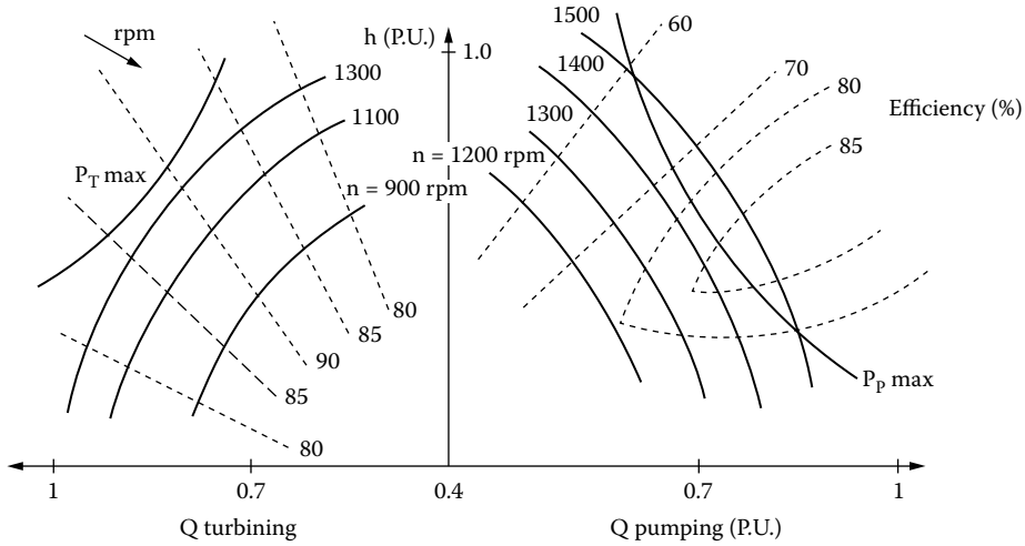
FIGURE 3.45 Typical characteristics of the pumping system of a radial-axial turbine plus pump.
