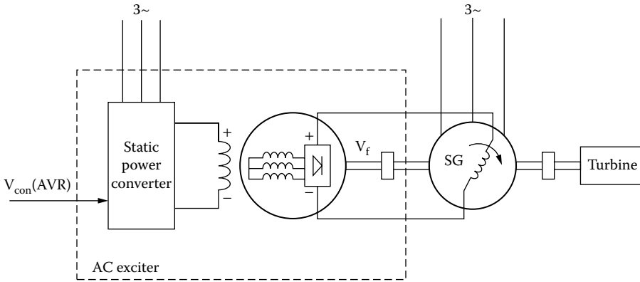
FIGURE 6.22 Alternating current (AC) exciter.
