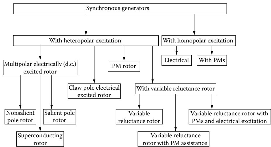
FIGURE 2.1 Synchronous generators.
