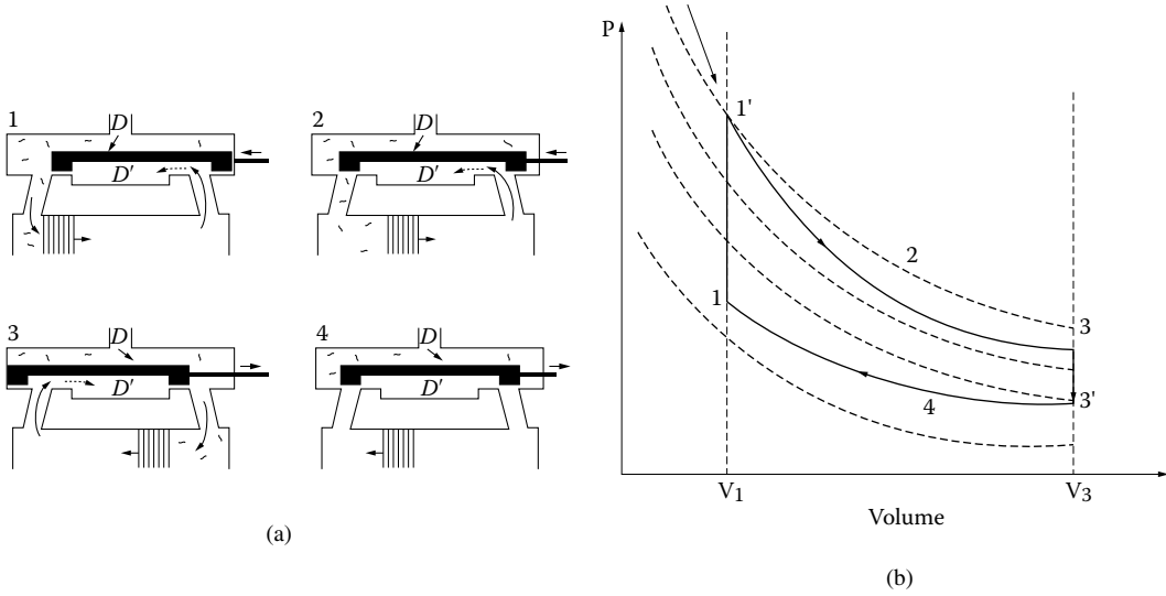
FIGURE 3.23 The steam engine “cycle”: (a) the four steps and (b) PV diagram.
