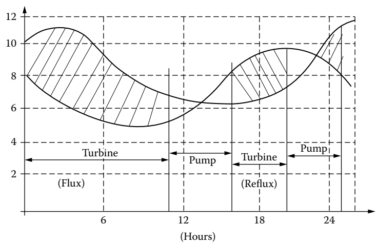
FIGURE 3.47 Head/time of the day in a tidal-wave turbine/pump.
