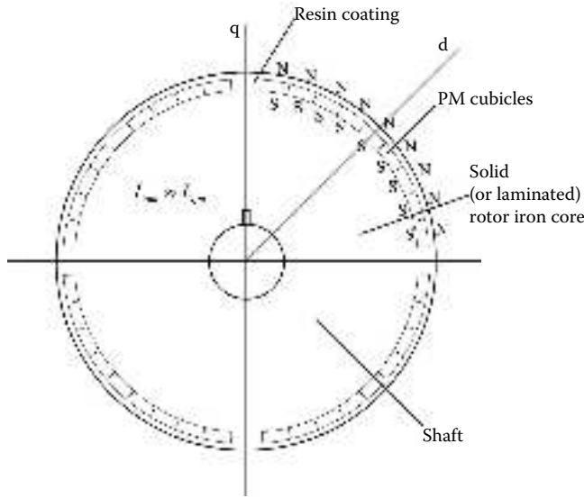
FIGURE 2.10 Surface PM rotor ( 2p_1 = \text{four poles} ).
