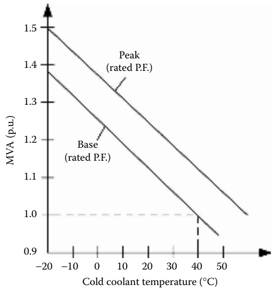
FIGURE 7.5 Ambient following synchronous generator ratings.
