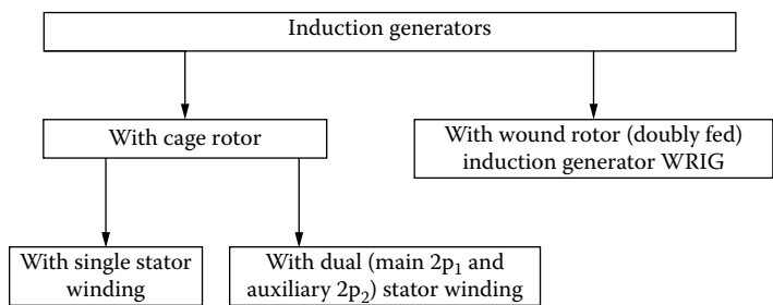
FIGURE 2.2 Induction generators.
