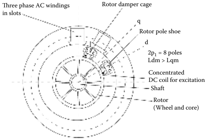
FIGURE 2.5 Synchronous generator with salient pole heteropolar DC concentrated excitation.
