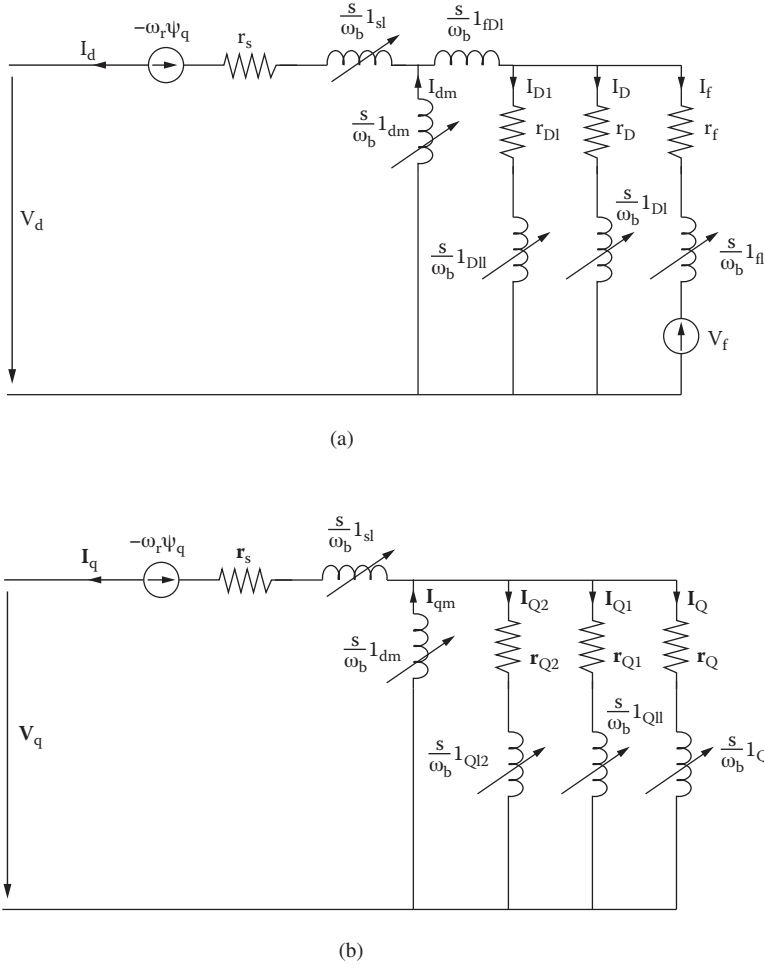
FIGURE 5.20 Three-circuit synchronous generator model with some variable inductances: (a) axis d and (b) axis q .
