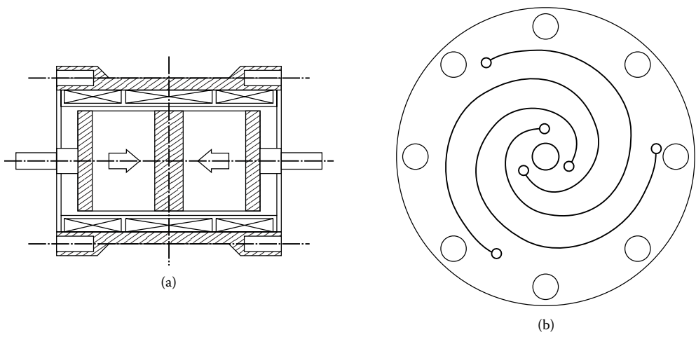
FIGURE 2.30 (a) Tubular linear motion alternator (LMA) and (b) with plunger supported on flexural springs.
