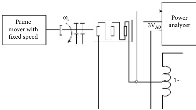
FIGURE 4.38 Measuring homopolar \underline{Z}_0 .
