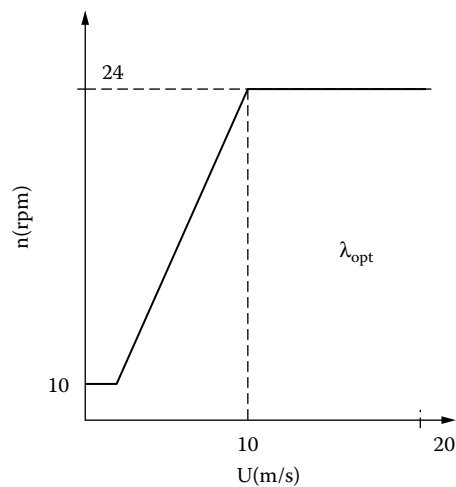
FIGURE 3.56 Typical optimum turbine/wind speed correlation.
