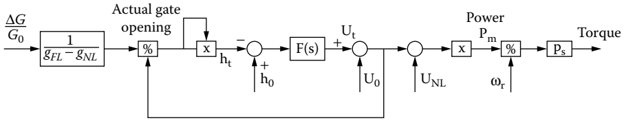
FIGURE 3.40 Nonlinear model of hydraulic turbine with hammer and surge tank effects.
