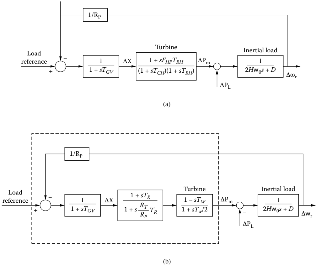
FIGURE 6.10 (a) Basic speed governor and steam turbine generator; (b) basic speed governor and hydraulic turbine generator.
