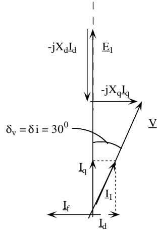
Phasor diagram for \cos \varphi_1 = 1 and zero losses.
