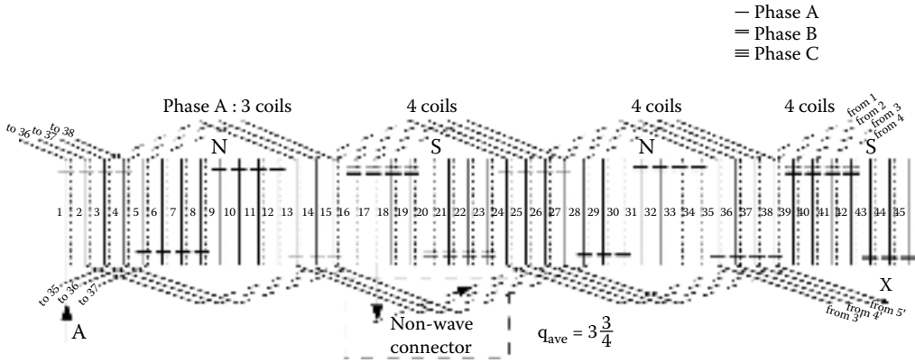
FIGURE 7.12 450-slot, 40-poles, q = 3 \frac{3}{4} bar-wave winding/phase A for the first N_s/t = 45 slots.
