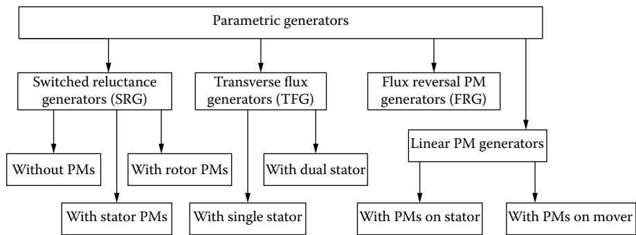
FIGURE 2.3 Parametric generators.
