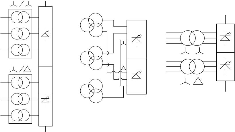
(a) 1-ph 2-winding (b) 1-ph 3-winding (c) 3-ph 2-winding
