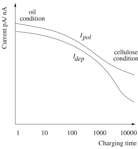
Figure 14.6 PDC curves: influences of oil conductivity and moisture in cellulose [37, 42].
