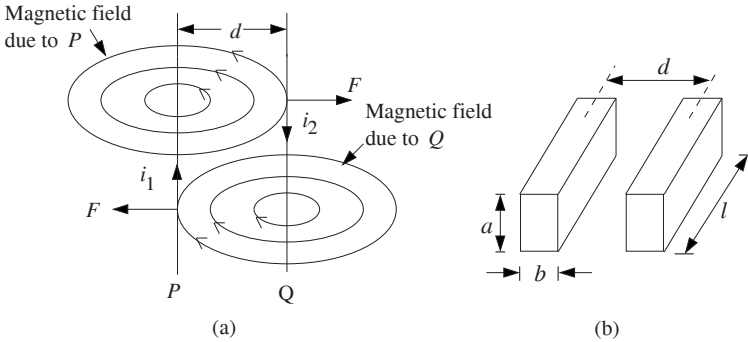
Figure 6.17 Force between parallel conductors.
