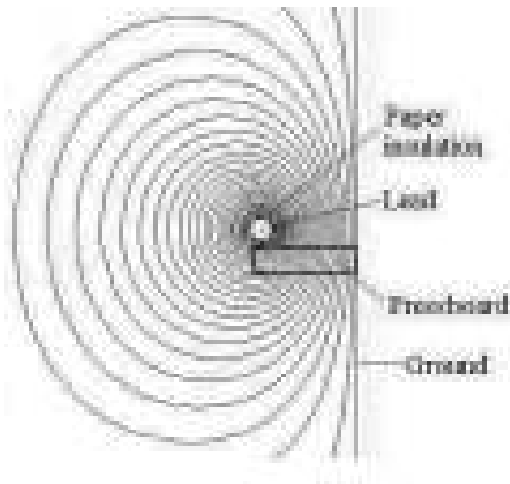
Figure 8.21 Optimum creepage distance calculation by FEM analysis.
