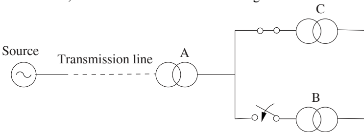
Figure 2.16 Sympathetic inrush.
