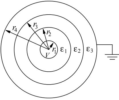
Figure 8.3 Concentric cylindrical electrodes with multiple dielectrics.
