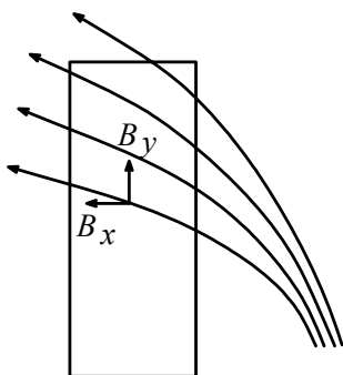
Figure 4.7 Winding conductor in a leakage field.
