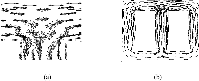
Figure 2.20 Rotational flux in a T-joint.
