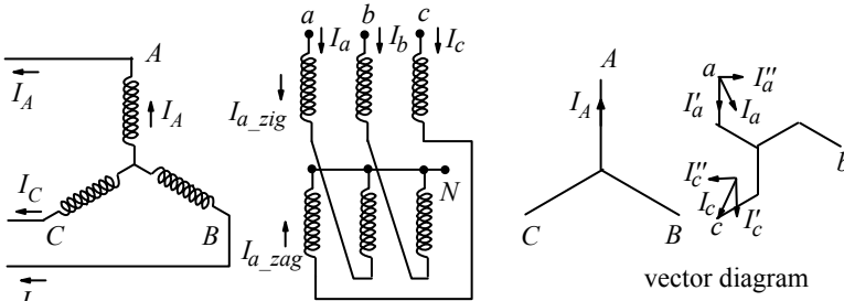
Figure 3.18 Reactance calculation of a transformer having a zigzag winding.
