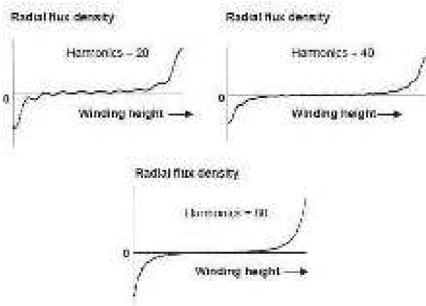
Figure 3.7 The effect of the number of space harmonics on the accuracy.
