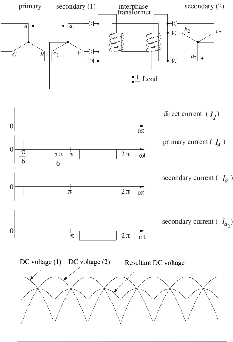
Figure 11.2 Interphase transformer: arrangement and waveforms.
