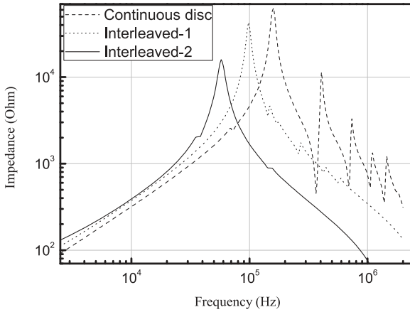
Figure 14.11 FRA curve of three coils with different series capacitance.
