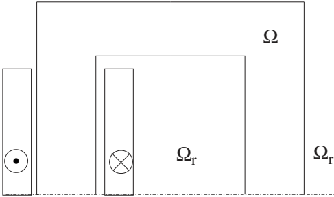
Figure 12.8 Use of total and reduced magnetic scalar potentials.
