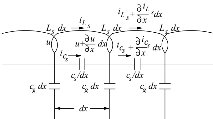
Figure 7.2 Impulse response: representation of a transformer winding.
