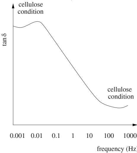
Figure 14.9 Interpretation of dissipation factor measurement [43, 46].
