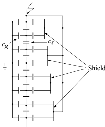
Figure 7.4 Electrostatic shields.
