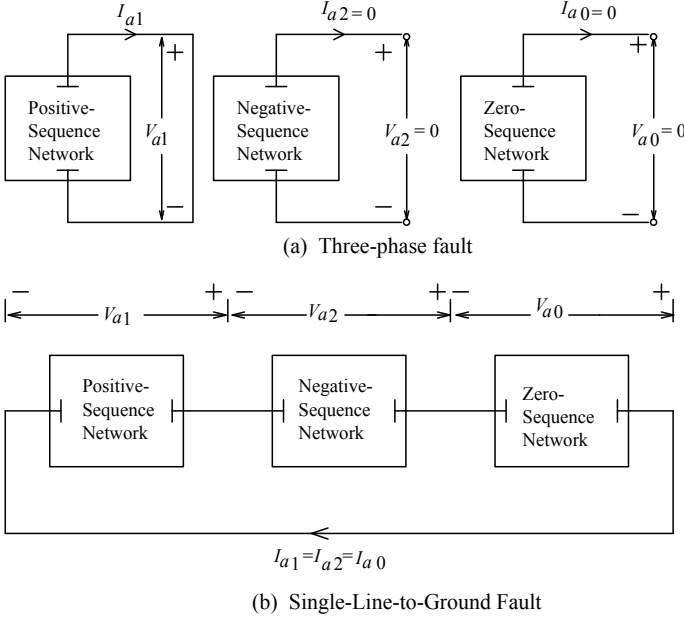
Figure 6.1 Sequence networks.
