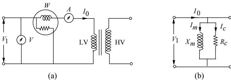
Figure 1.8 Open-circuit test.
