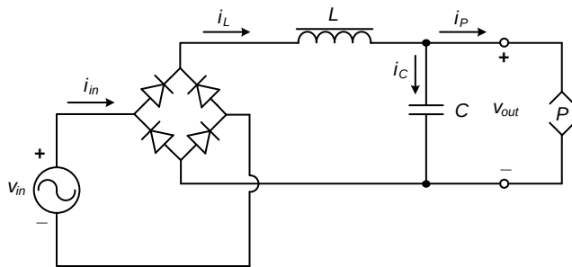
Figure 10.12 Rectifier circuit with passive power factor correction.
