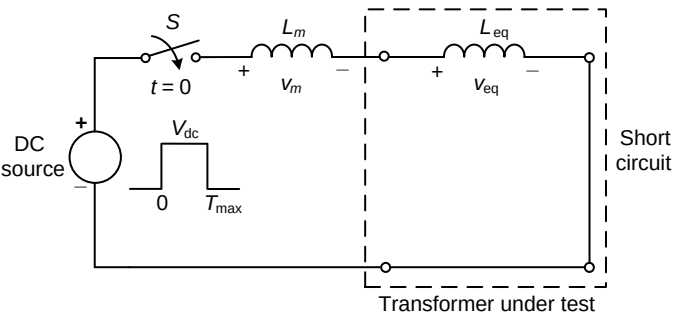
Figure 8.13 Transformer short-circuit test at high frequency.
