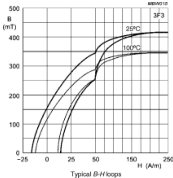
Figure 1.8 Temperature dependence of saturation flux density [Reproduced with permission of Ferroxcube].
