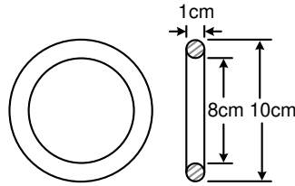
Figure 7.9 Toroidal core.
