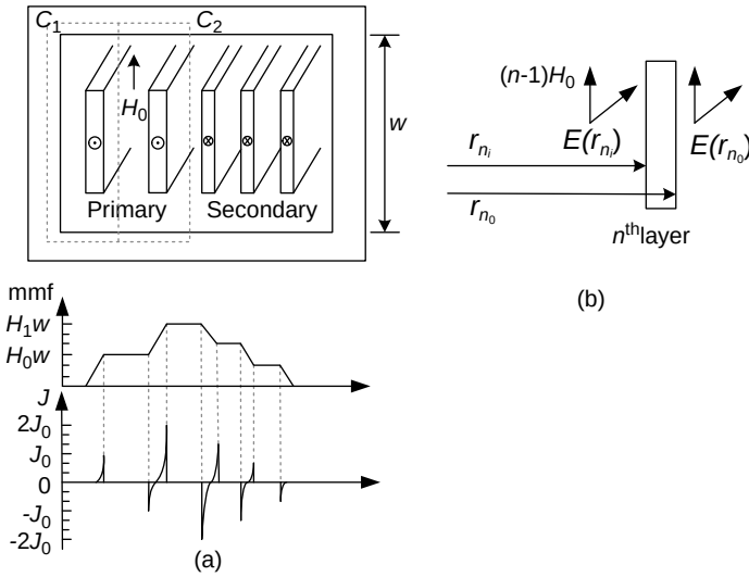
Figure 6.6 Transformer cross-section with (a) associated mmf diagram and current density at high frequency, (b) generalized n th layer.
