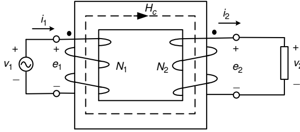
Figure 4.2 Two-winding transformer: load conditions.
