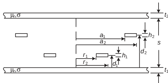
Figure 9.9 Planar coils in a sandwich structure.
