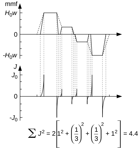
Figure 6.18 Current density distribution after interleaving.
