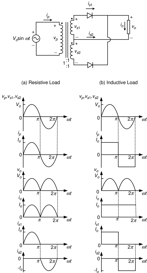
Figure 4.18 Centre-tapped rectifier and associated waveforms for (a) resistive and (b) inductive loads.
