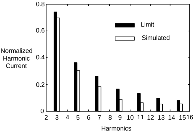
Figure 10.21 Harmonics with the variable inductor.
