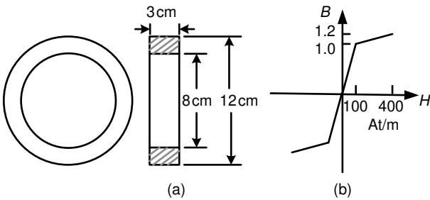
Figure 2.21 Problem 2.2 toroidal core.
