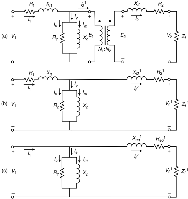
Figure 4.11 Transformer equivalent circuits.
