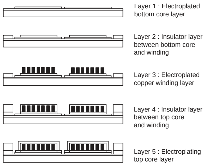
Figure 9.21 Microfabrication process flow for an inductor.
