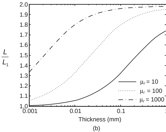
Figure 9.7 Enhancement of inductance with magnetic substrate: (a) as a function of \mu_r , (b) as a function of t .
