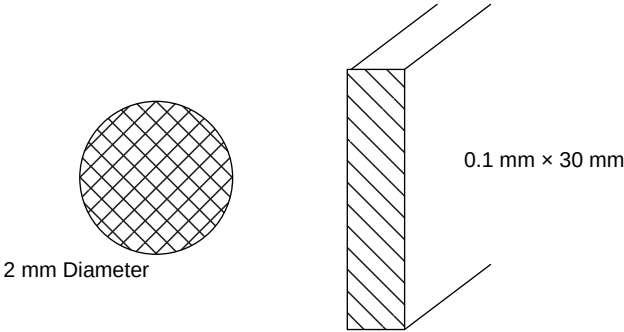
Figure 6.14 Round versus foil conductor.
