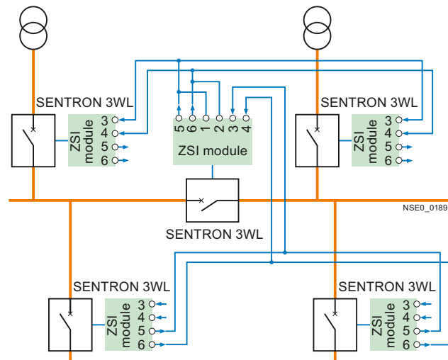
ZSI function: Connection using a coupling switch, use of 3WL circuit breakers
