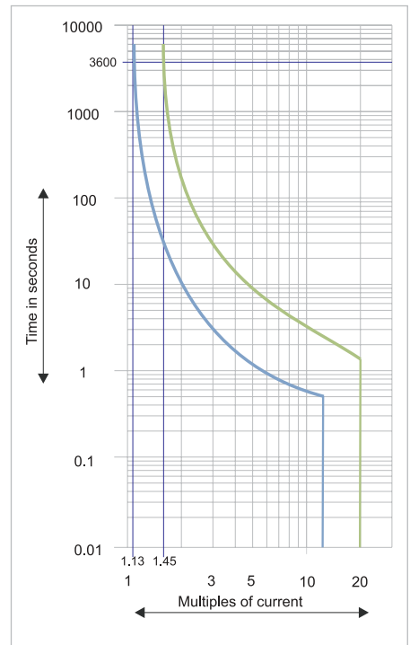
D Curve
