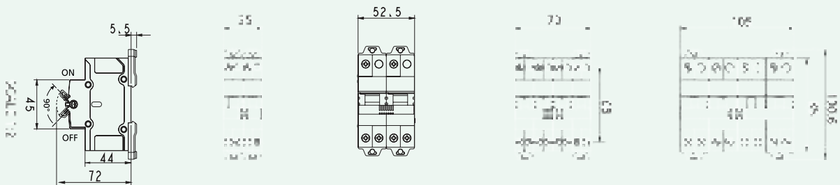
SIDE VIEW 2 POLE (25/40A) 2 POLE (63A) 4 POLE (40A) 4 POLE (63A)
