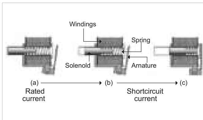
Solenoid
