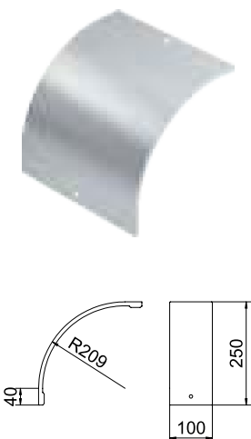
Cover for 90° vertical bend (falling) fitting with 100 mm side height for GKS... cable tray types
