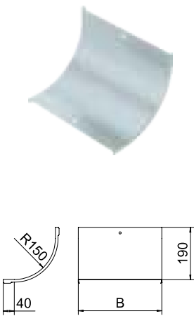
Cover for 90° vertical bend (rising) fitting for GKS... cable tray types
