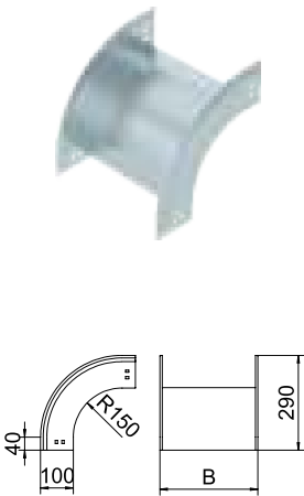
90° vertical bend, falling, for all GKS... cable tray types of 100 mm side height.
