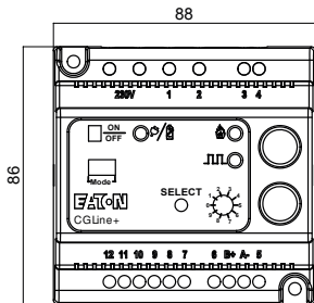
Dimensional drawings, data in mm
