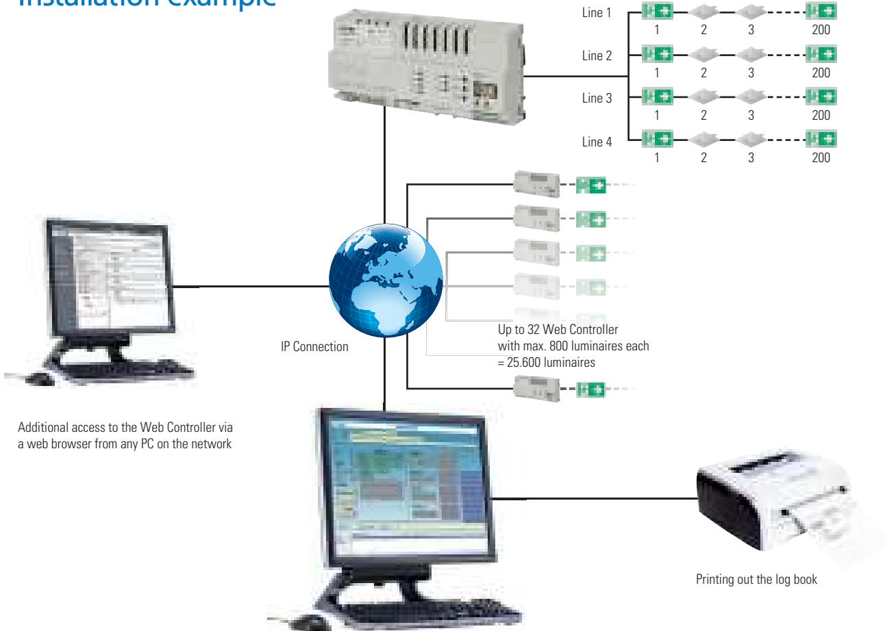
CGVision PC : Configuration and complete visualisation of all luminaires
