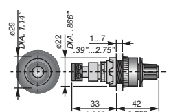
CT-POT.02
