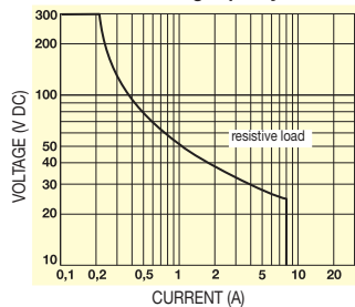
RB 121 A 1: 110 V AC/DC block 2: 135 V AC/DC block
