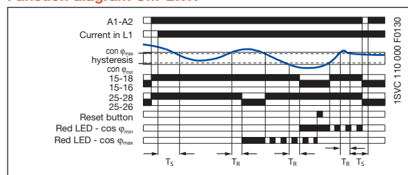
Function diagram CM-LWN
