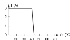
RB 131 CV Very low level
