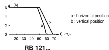
Derating curve
