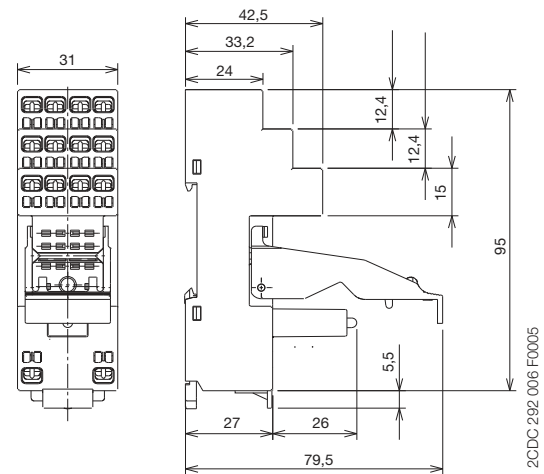
CR-M2LC , CR-M4LC
