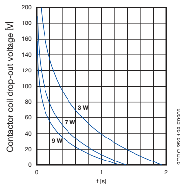
Time delay guideline values 200-240 V AC version with jumper 3/4
