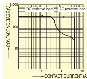
Derating curves
