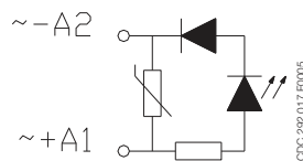
CR-P/M 62C, CR-P/M 92C, CR-P/M 62DV, CR-P/M 62D, CR-P/M 62CV, CR-P/M 92CV
