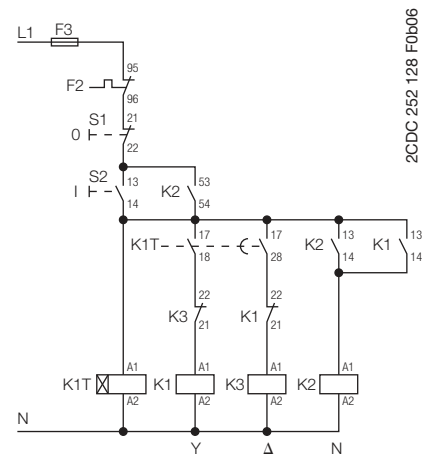
Control circuit diagram
