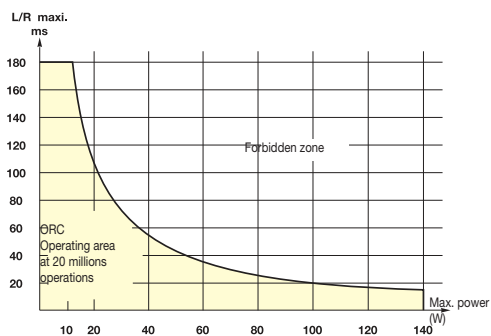
Derating curves
