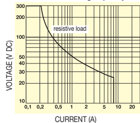
Max. DC load breaking capacity : curve 2
