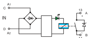
ORC 111
