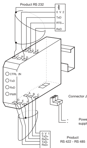
RS 422 - RS 485 4 WIRE SERIAL LINKS
