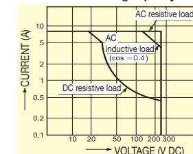
Max. DC load breaking capacity : curve 2
