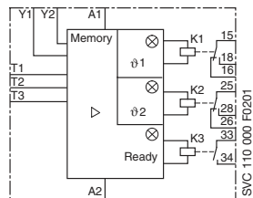
C512
