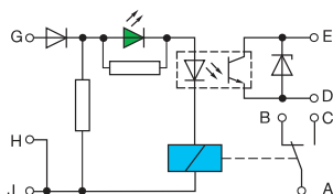
ROB 121
