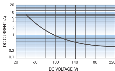
Derating curves
