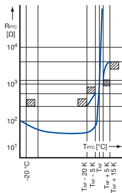
Temperature sensor characteristic
