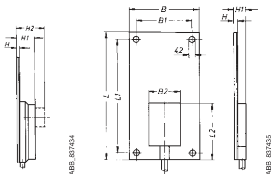
Dimensional drawing 2
