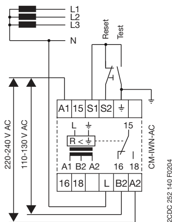
Three-phase IT-N system
