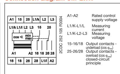
Connection diagram CM-LWN
