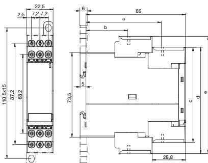
C510 / C511 22.5 mm
