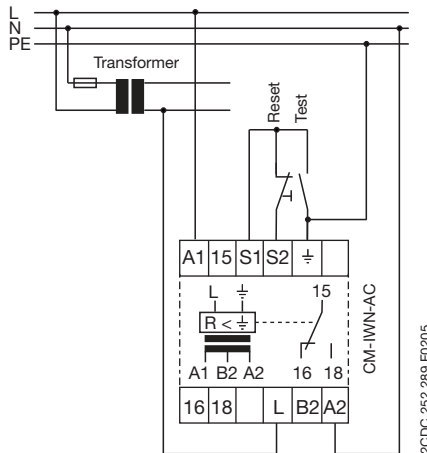
Single-phase IT-N system
