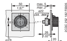
CT-POT.03
