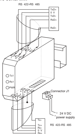
RS 422 - RS 485 4 wire serial link
