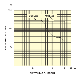
Derating curve
