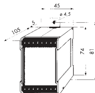
C558.01 45 mm
