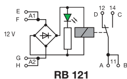
Relay blocks R900
