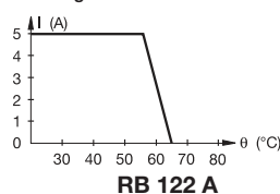
Derating curves
