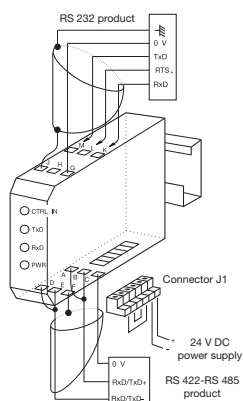
RS 422 - RS 485 2 WIRE SERIAL LINKS
