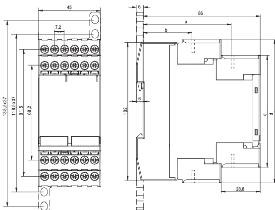
C512/C513 45 mm
