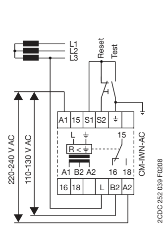
Three-phase IT system
