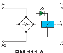
RM 111 A
