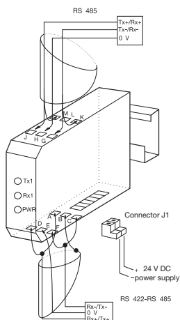
RS 422 - RS 485 2 wire serial link
