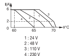
D 2,5/5-R121
