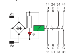
RB 114 A
