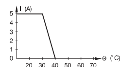
RB 131 BCVR Very low level
