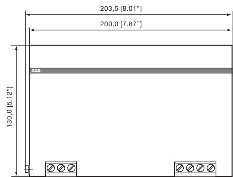
CP-S 24/20.0 CP-C 24/20.0
