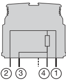
Plug with 250 Ω accuracy resistance for analogical signals.
