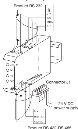
RS 422 - RS 485 SERIAL LINK (2 wires)
