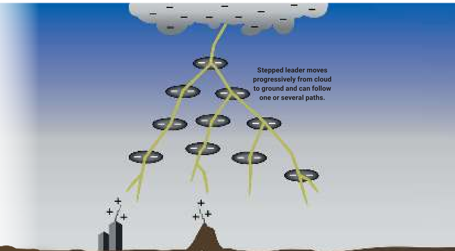
Figure 4. Electric field due to downleader increases to the point of initiation of an upward leader.
