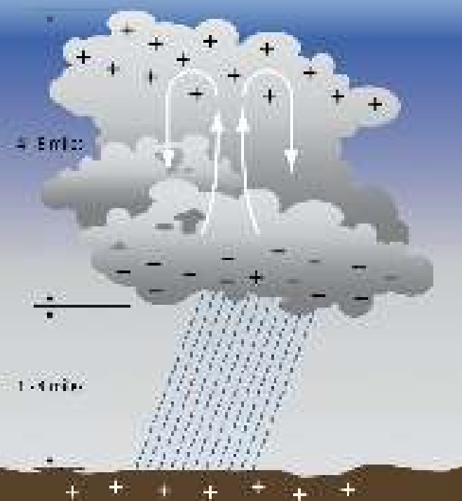
Figure 1. Typical positive and negative charge distribution in the cumulonimbus cloud.
