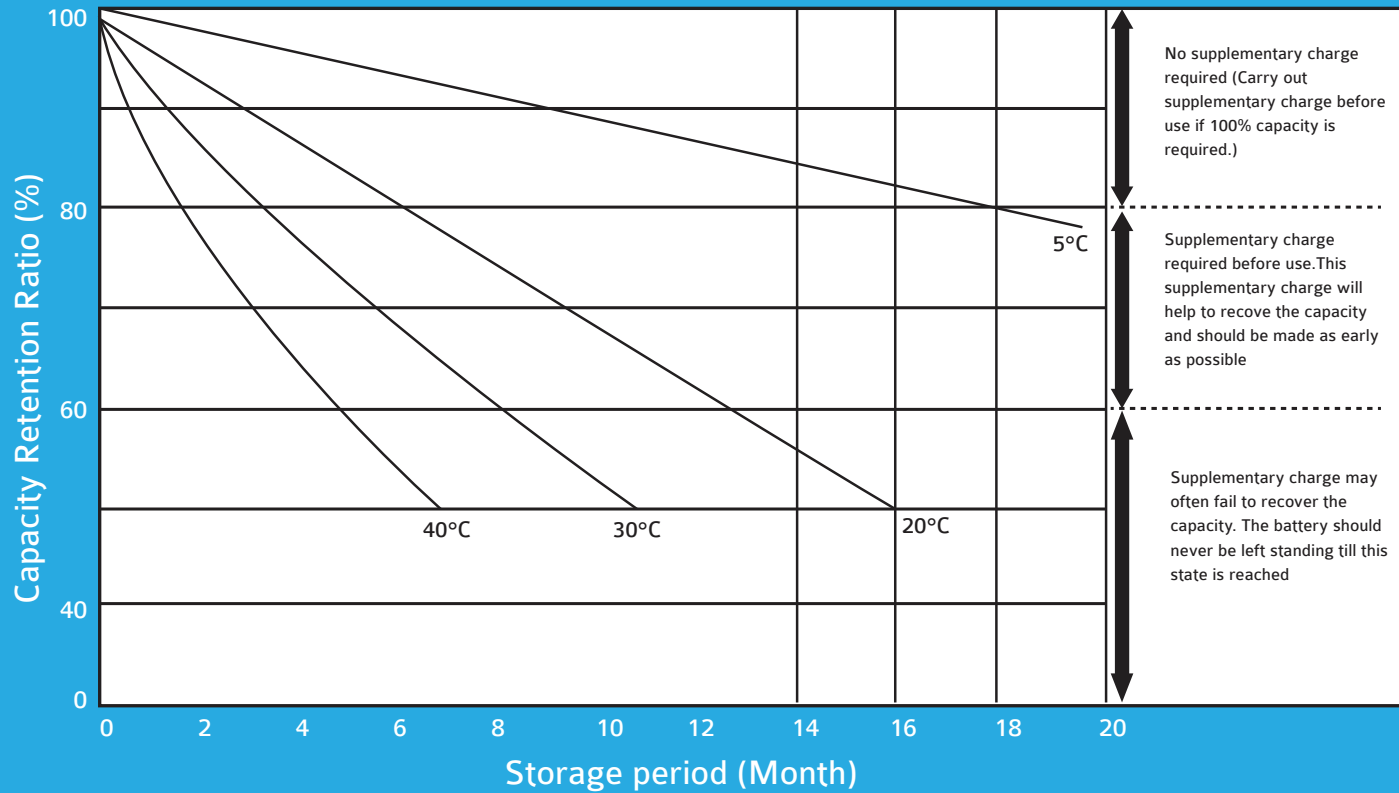
Capacity retention characteristics and the supplementary charge and storage guideline
