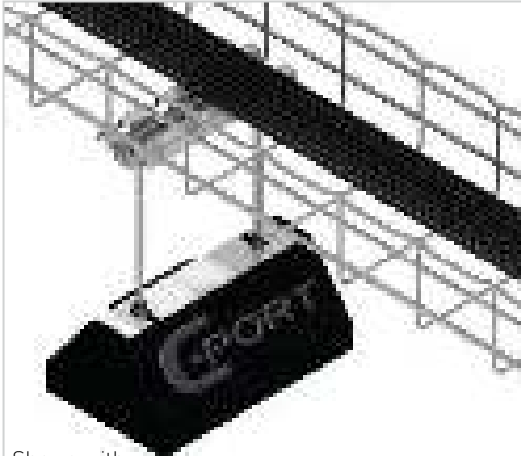
Shown with CFEP (Cablofil Extension Plate) increases load capacity to 500 lbs.
