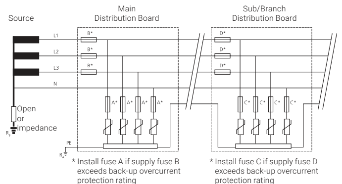
Figure 103. IT system identification – with distributed neutral.
