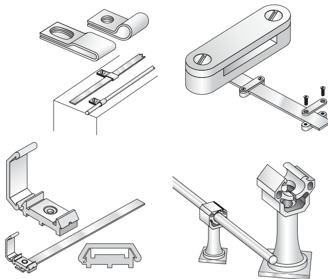
Figure 57. Typical down-conductor fixings.
