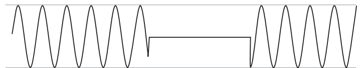
Figure 84. Dropout.
