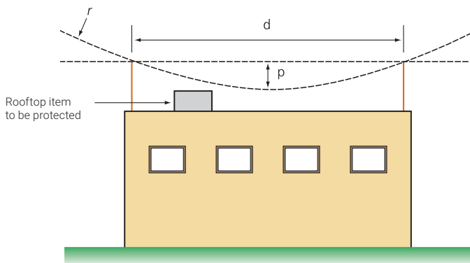
Figure 29. Penetration distance of rolling sphere.
