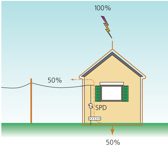
Figure 89. Simplified current distribution.
