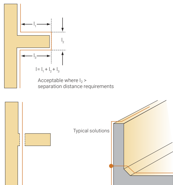
Figure 55. Down-conductor loops.
