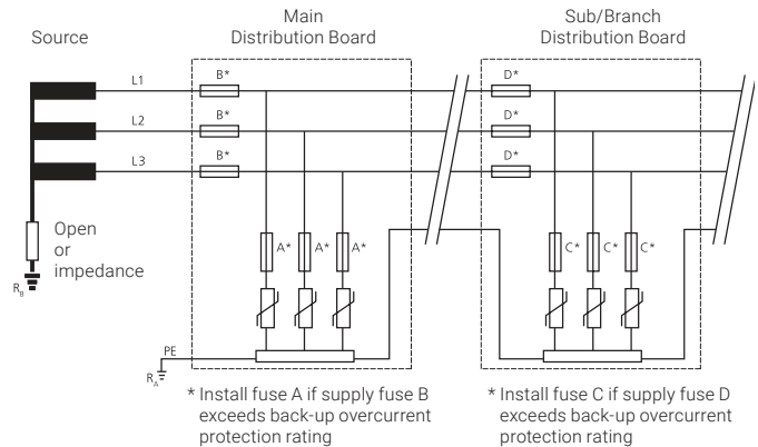
Figure 102. IT system identification – without distributed neutral.
