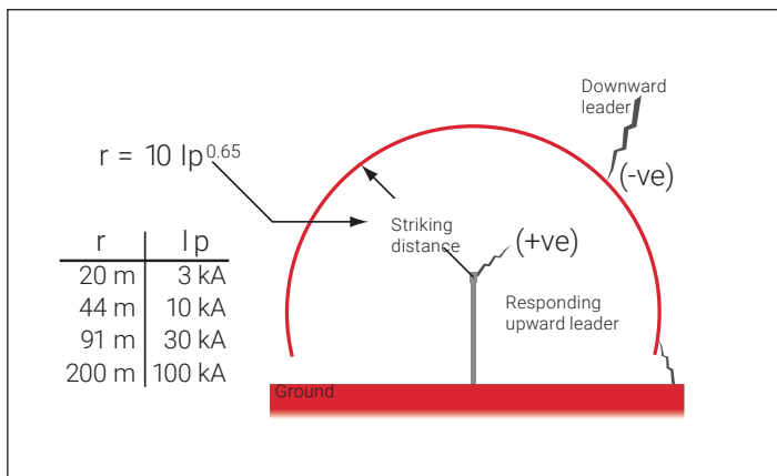
Figure 7. Striking Distance.
