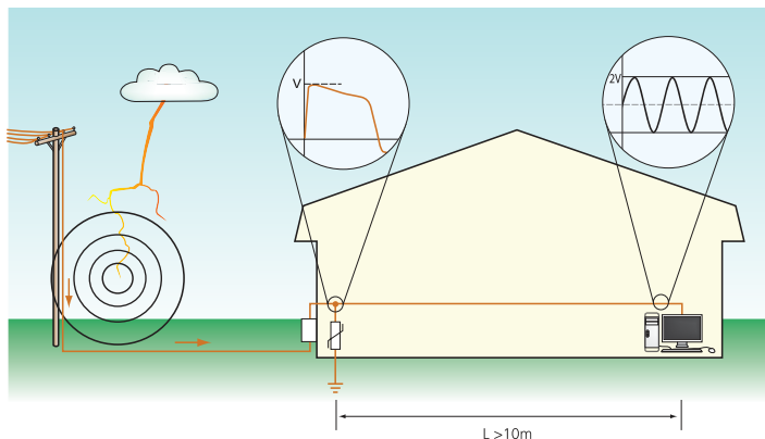
Figure 95. Oscillation effect.
