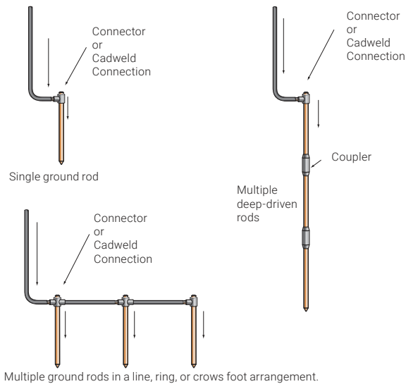
Figure 69. Example vertical electrode arrangements.
