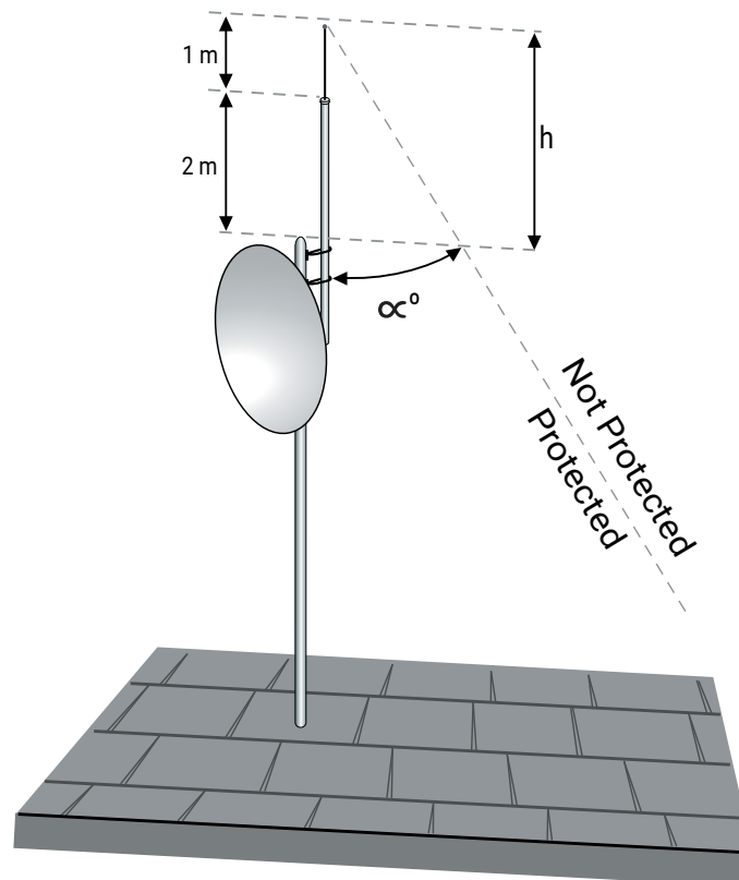
Figure 64. Isolated mast and Isolated Down-conductor protecting a roof-top antenna.
