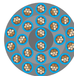
Drawing (a) 24 Core Cable
