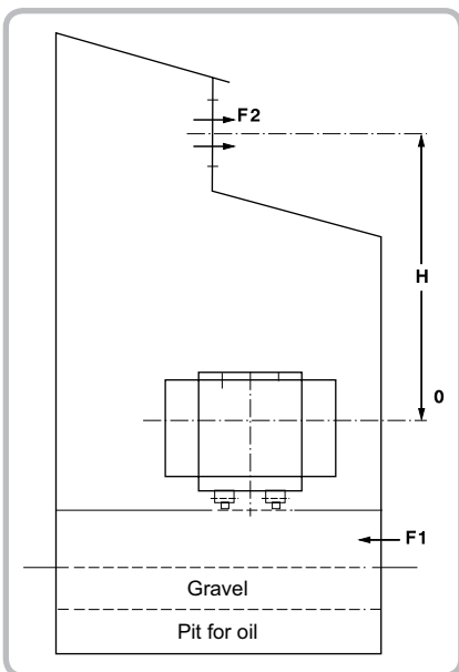
Dimensions of transformer installation room
