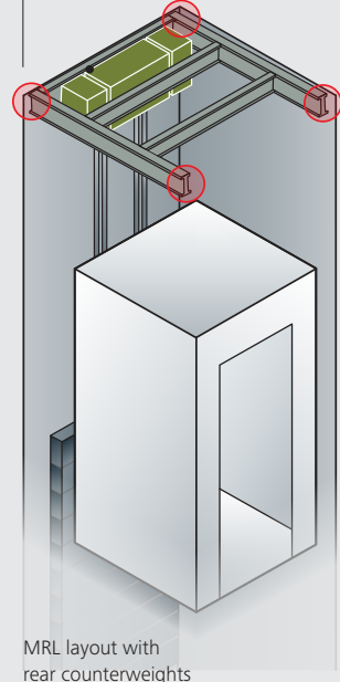
Elevator machine loads transferred to the building
