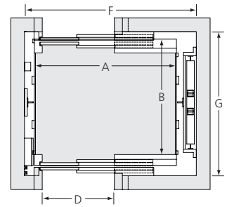
Front/rear opening 10 two-speed left opening (2SSO)
