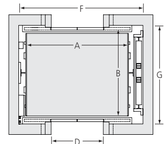
Front/rear opening single-speed center opening (SSCO)
