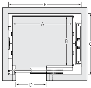
Front opening two-speed left opening (2SSO)
