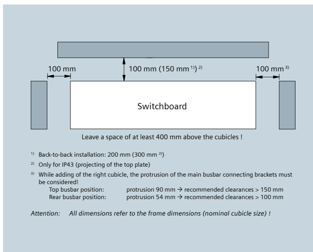
Fig. 8/1: Clearances to obstacles
