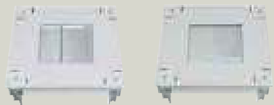
For bases whose width and depth are identical, the direction of the runners on the cable gland plate can be reversed
