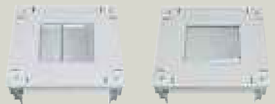
For enclosures whose width and depth are identical, the direction in which the compartment opens can be altered
